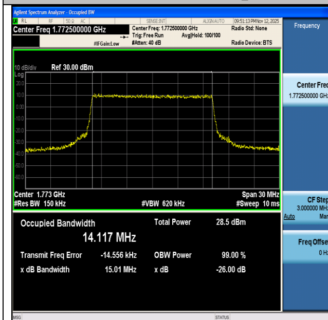
NTNV-n66-PC3-15-15-H-CP-16QAM-Outer_Full-Ant1-PASS
