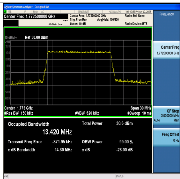
NTNV-n66-PC3-15-15-H-DFT-QPSK-Outer_Full-Ant1-PASS
