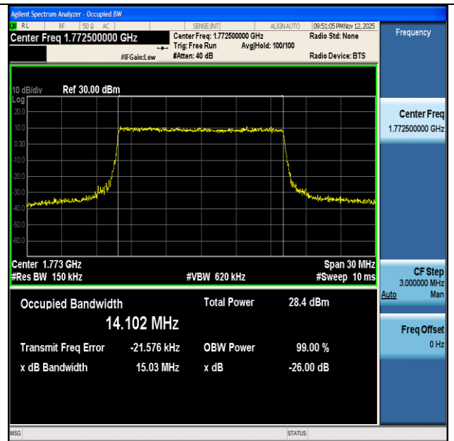
NTNV-n66-PC3-15-15-H-CP-QPSK-Outer_Full-Ant1-PASS
