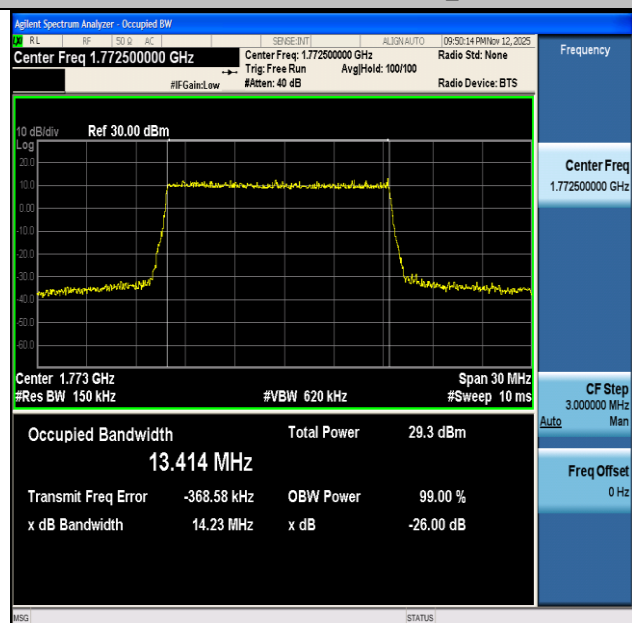
NTNV-n66-PC3-15-15-H-DFT-64QAM-Outer_Full-Ant1-PASS
