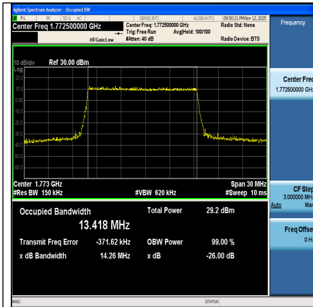
NTNV-n66-PC3-15-15-H-DFT-256QAM-Outer_Full-Ant1-PASS
