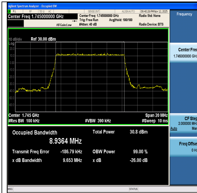
NTNV-n66-PC3-15-10-M-DFT-BPSK-Outer_Full-Ant1-PASS
