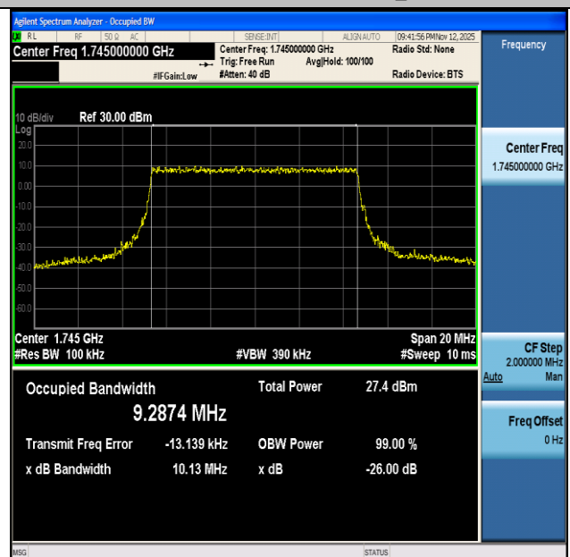
NTNV-n66-PC3-15-10-M-CP-64QAM-Outer_Full-Ant1-PASS
