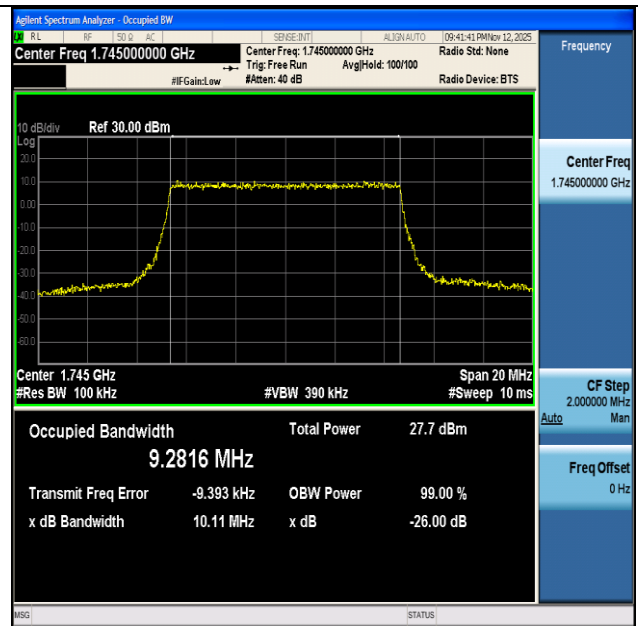
NTNV-n66-PC3-15-10-M-CP-QPSK-Outer_Full-Ant1-PASS
