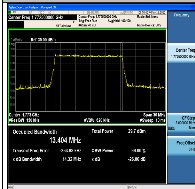
NTNV-n66-PC3-15-15-H-DFT-16QAM-Outer_Full-Ant1-PASS
