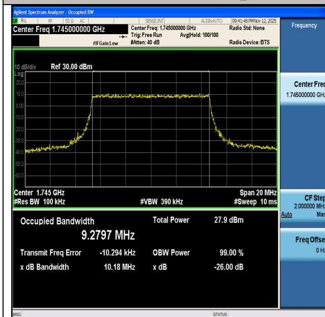
NTNV-n66-PC3-15-10-M-CP-16QAM-Outer_Full-Ant1-PASS
