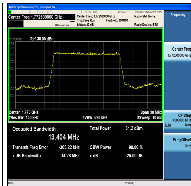
NTNV-n66-PC3-15-15-H-DFT-BPSK-Outer_Full-Ant1-PASS
