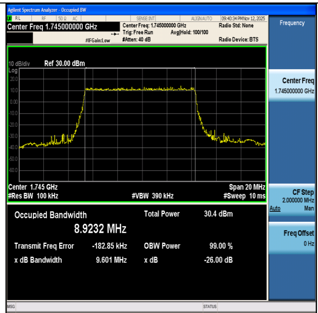
NTNV-n66-PC3-15-10-M-DFT-QPSK-Outer_Full-Ant1-PASS
