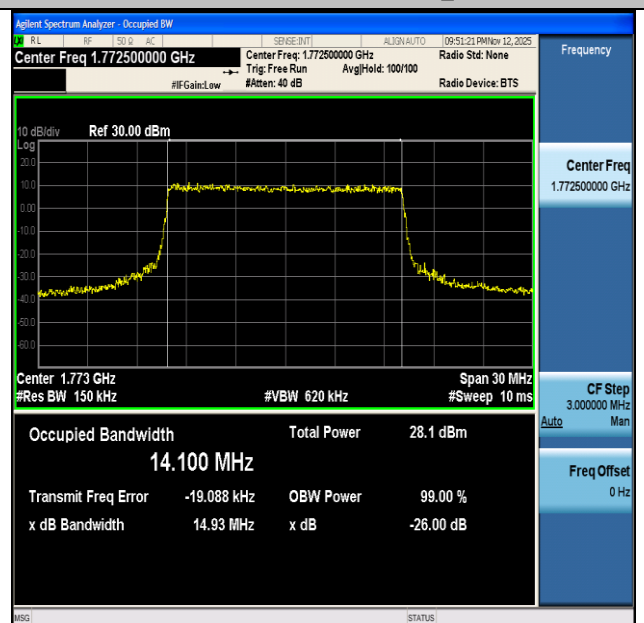
NTNV-n66-PC3-15-15-H-CP-64QAM-Outer_Full-Ant1-PASS
