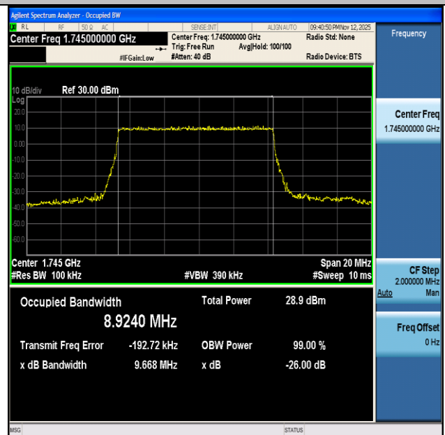
NTNV-n66-PC3-15-10-M-DFT-64QAM-Outer_Full-Ant1-PASS
