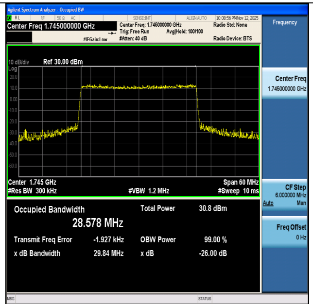
NTNV-n66-PC3-15-30-M-DFT-QPSK-Outer_Full-Ant1-PASS
