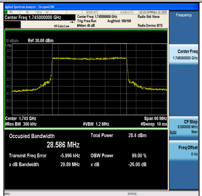
NTNV-n66-PC3-15-30-M-CP-64QAM-Outer_Full-Ant1-PASS
