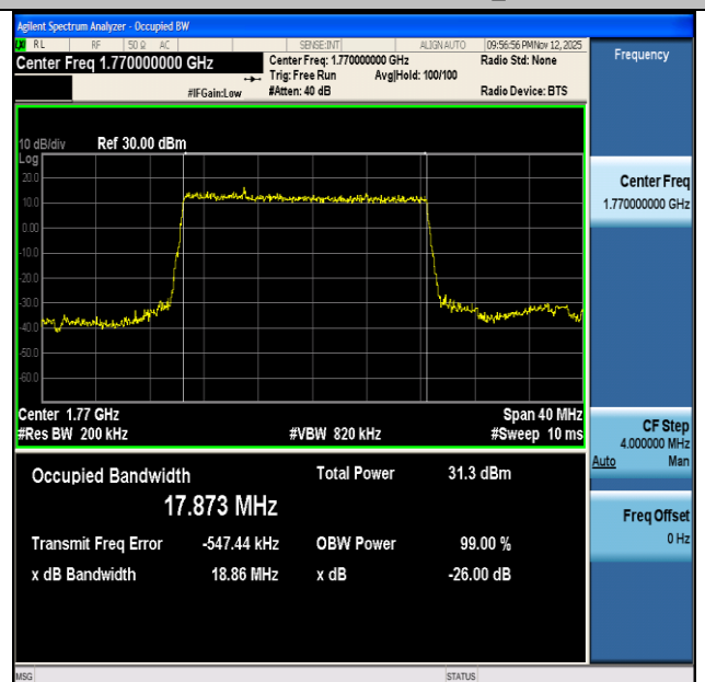
NTNV-n66-PC3-15-20-H-DFT-BPSK-Outer_Full-Ant1-PASS
