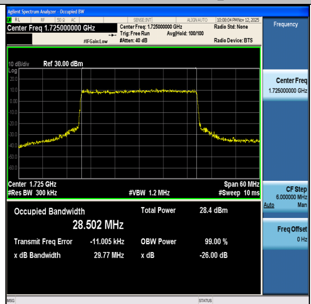
NTNV-n66-PC3-15-30-L-CP-256QAM-Outer_Full-Ant1-PASS
