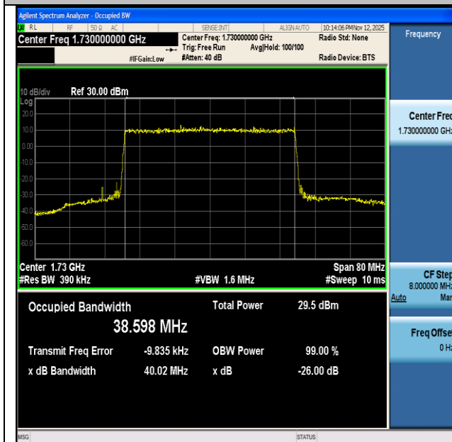
NTNV-n66-PC3-15-40-L-DFT-256QAM-Outer_Full-Ant1-PASS
