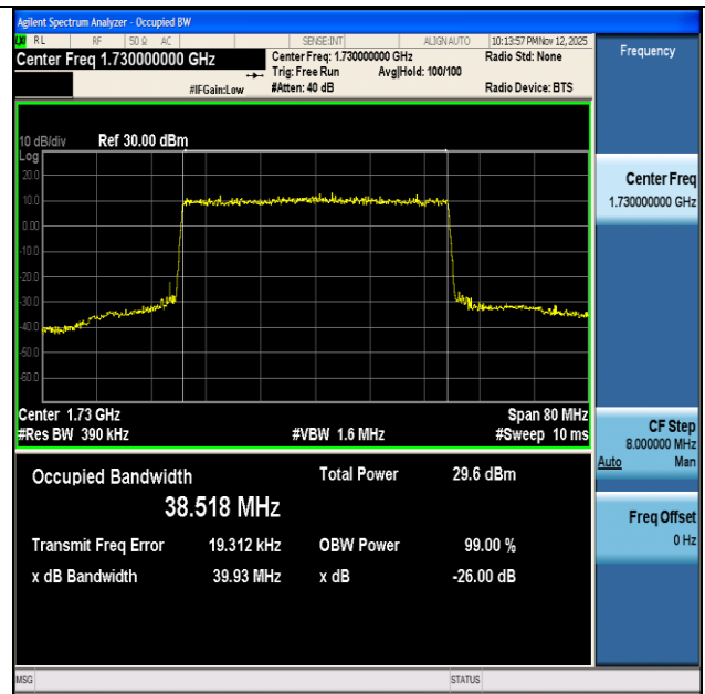
NTNV-n66-PC3-15-40-L-DFT-64QAM-Outer_Full-Ant1-PASS
