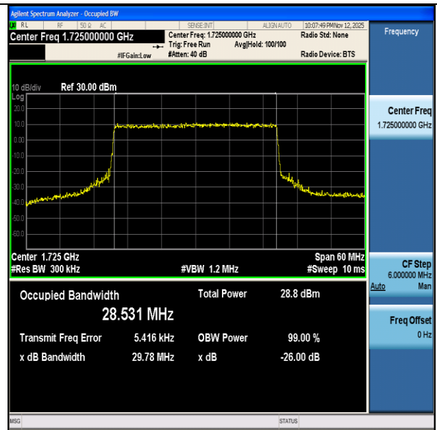
NTNV-n66-PC3-15-30-L-CP-16QAM-Outer_Full-Ant1-PASS
