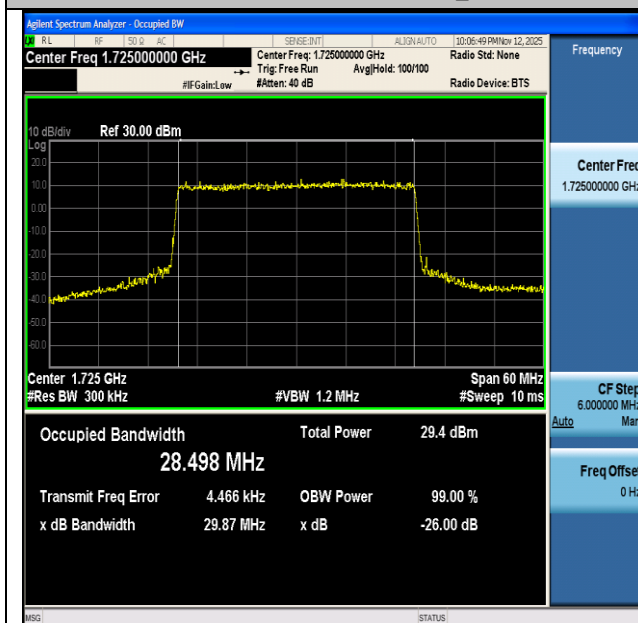
NTNV-n66-PC3-15-30-L-DFT-64QAM-Outer_Full-Ant1-PASS
