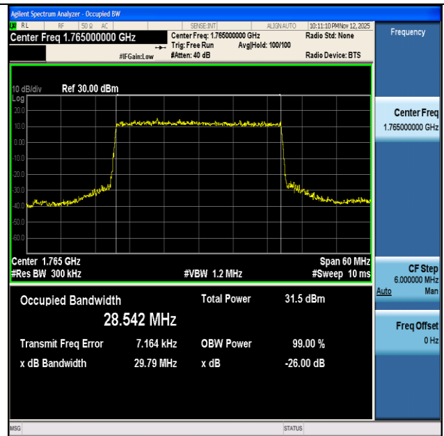
NTNV-n66-PC3-15-30-H-DFT-BPSK-Outer_Full-Ant1-PASS
