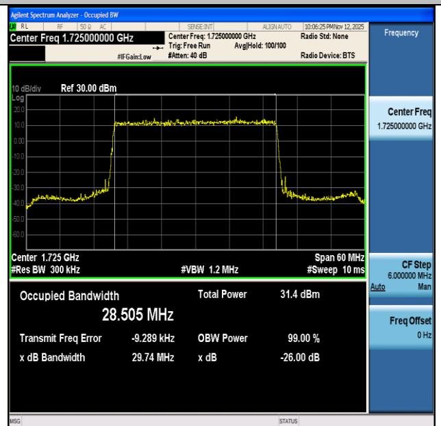
NTNV-n66-PC3-15-30-L-DFT-BPSK-Outer_Full-Ant1-PASS
