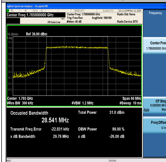
NTNV-n66-PC3-15-30-H-DFT-QPSK-Outer_Full-Ant1-PASS
