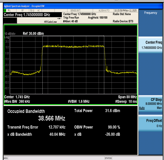
NTNV-n66-PC3-15-40-M-DFT-BPSK-Outer_Full-Ant1-PASS
