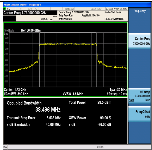
NTNV-n66-PC3-15-40-L-CP-64QAM-Outer_Full-Ant1-PASS
