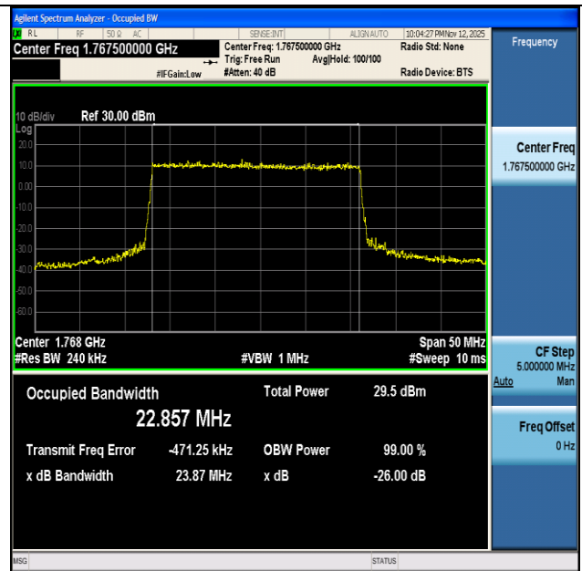
NTNV-n66-PC3-15-25-H-DFT-64QAM-Outer_Full-Ant1-PASS
