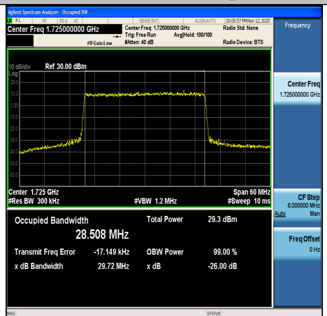
NTNV-n66-PC3-15-30-L-DFT-256QAM-Outer_Full-Ant1-PASS
