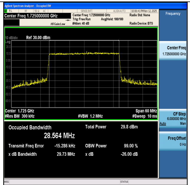
NTNV-n66-PC3-15-30-L-DFT-16QAM-Outer_Full-Ant1-PASS
