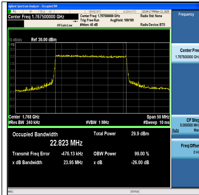
NTNV-n66-PC3-15-25-H-DFT-16QAM-Outer_Full-Ant1-PASS
