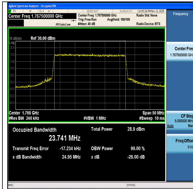
NTNV-n66-PC3-15-25-H-CP-16QAM-Outer_Full-Ant1-PASS
