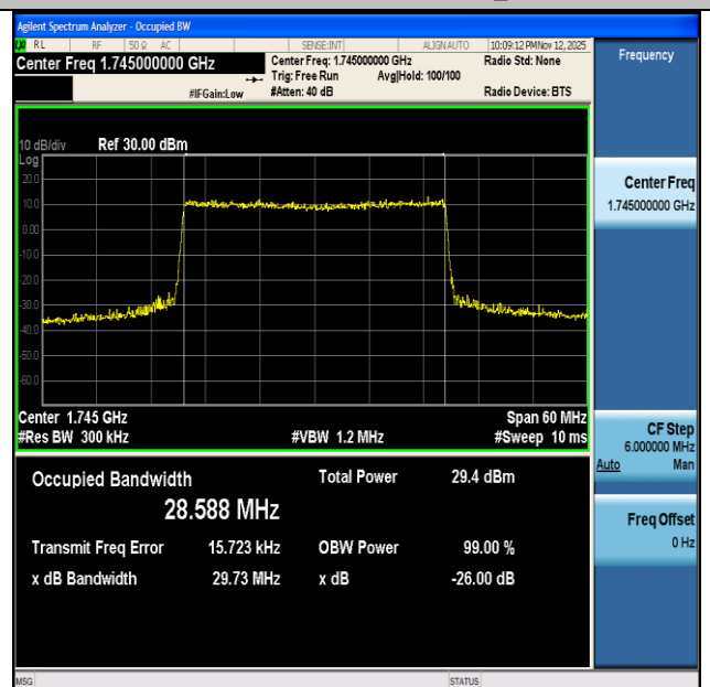
NTNV-n66-PC3-15-30-M-DFT-64QAM-Outer_Full-Ant1-PASS
