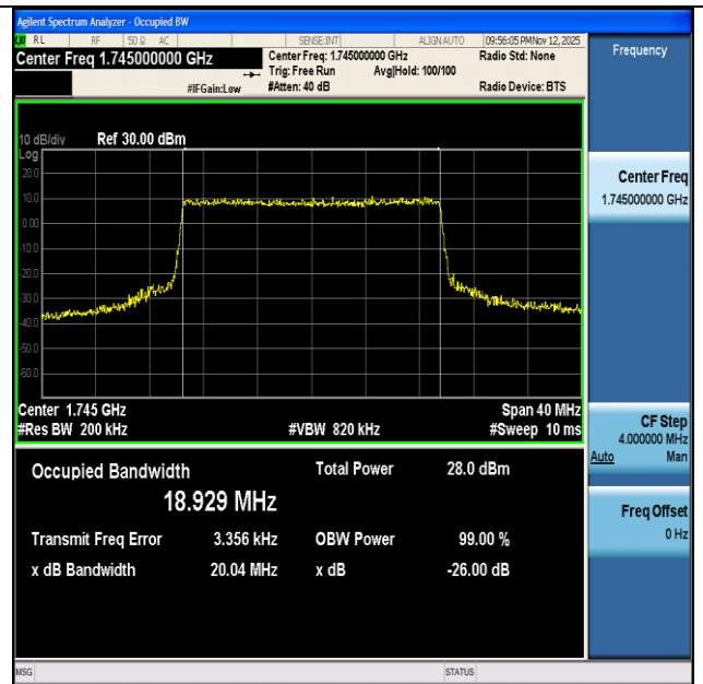
NTNV-n66-PC3-15-20-M-CP-64QAM-Outer_Full-Ant1-PASS
