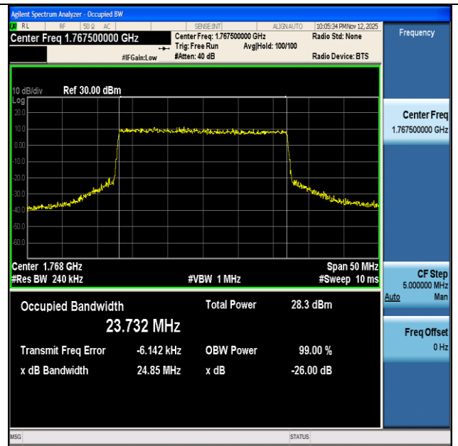
NTNV-n66-PC3-15-25-H-CP-64QAM-Outer_Full-Ant1-PASS
