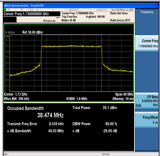
NTNV-n66-PC3-15-40-L-CP-QPSK-Outer_Full-Ant1-PASS
