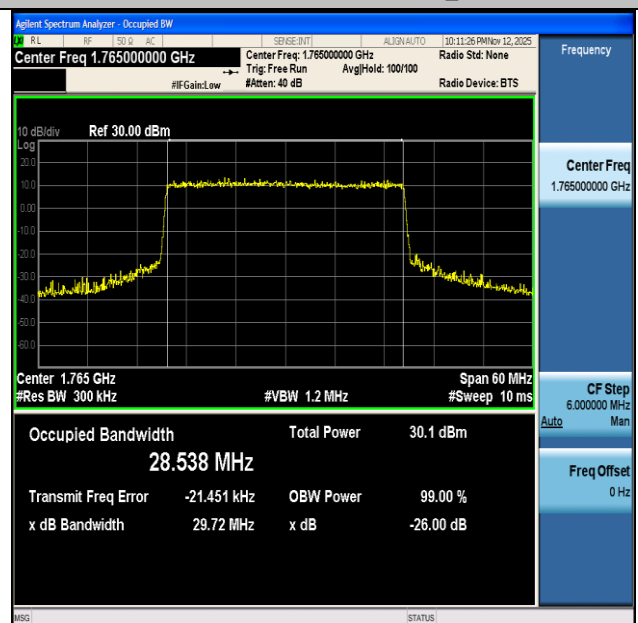
NTNV-n66-PC3-15-30-H-DFT-16QAM-Outer_Full-Ant1-PASS
