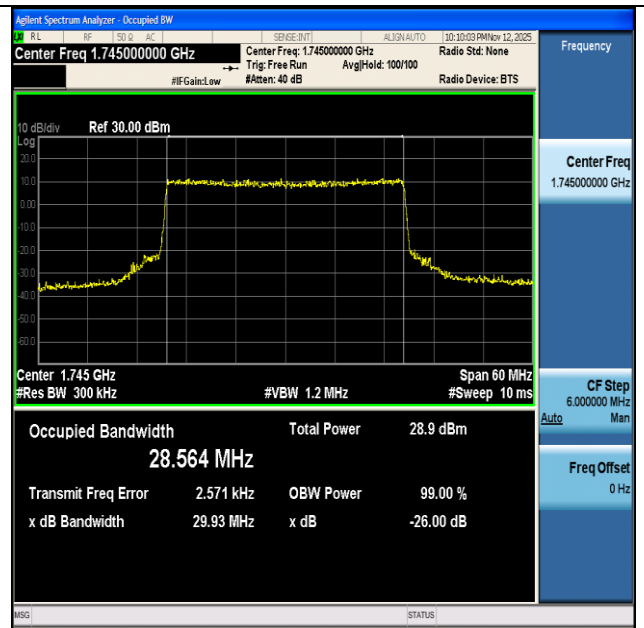
NTNV-n66-PC3-15-30-M-CP-QPSK-Outer_Full-Ant1-PASS
