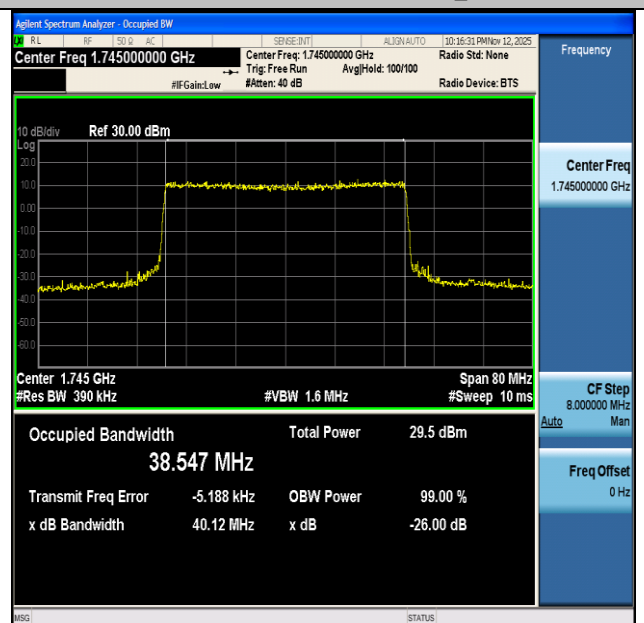
NTNV-n66-PC3-15-40-M-DFT-256QAM-Outer_Full-Ant1-PASS
