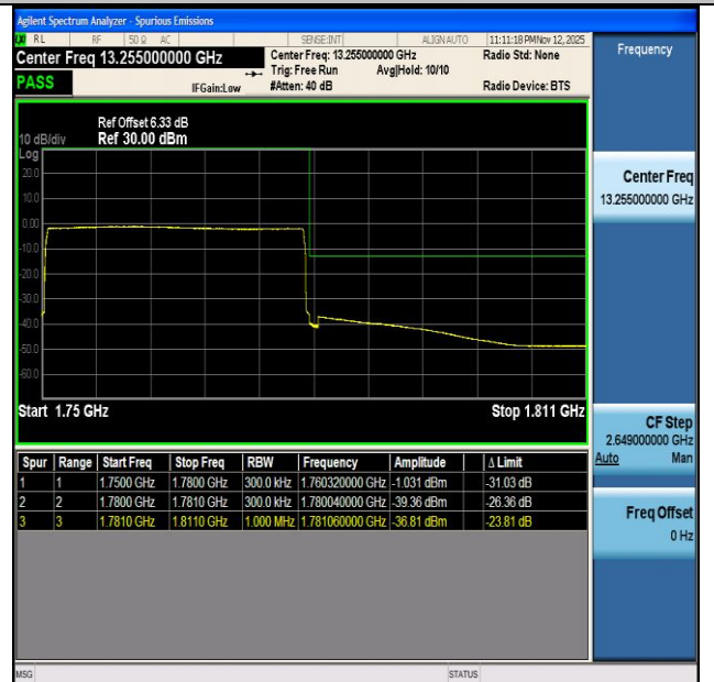
NTNV-n66-PC3-15-30-H-CP-QPSK-Outer_Full-PASS
