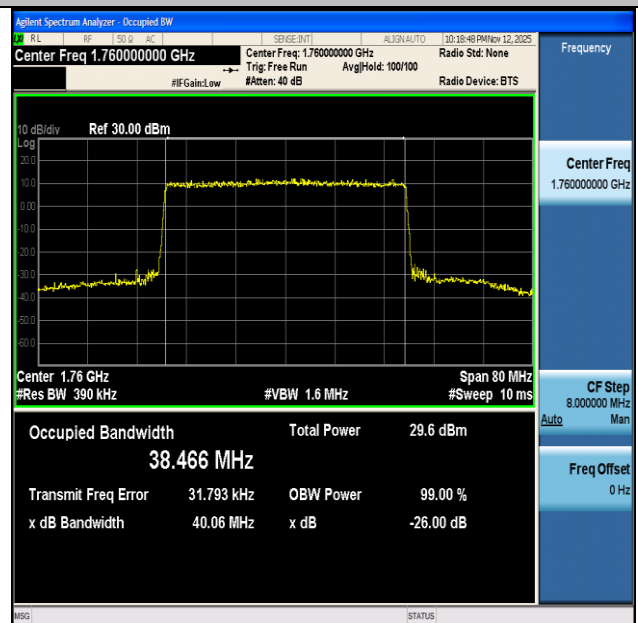
NTNV-n66-PC3-15-40-H-DFT-64QAM-Outer_Full-Ant1-PASS
