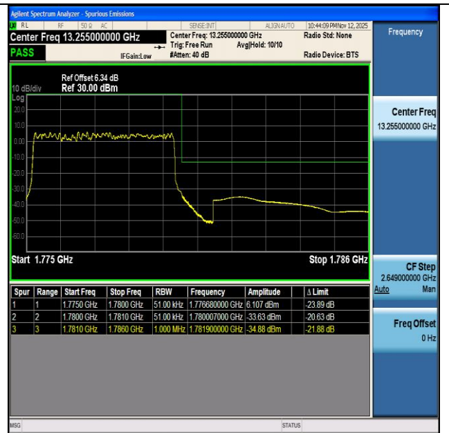
NTNV-n66-PC3-15-5-H-DFT-BPSK-Outer_Full-PASS
