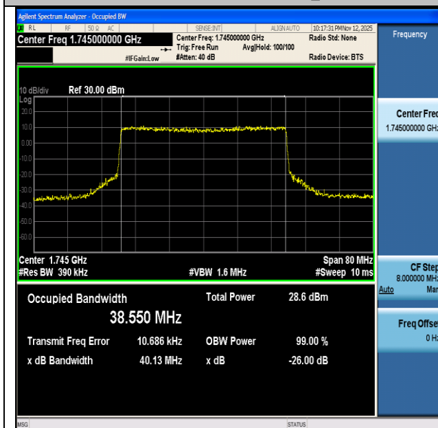
NTNV-n66-PC3-15-40-M-CP-64QAM-Outer_Full-Ant1-PASS
