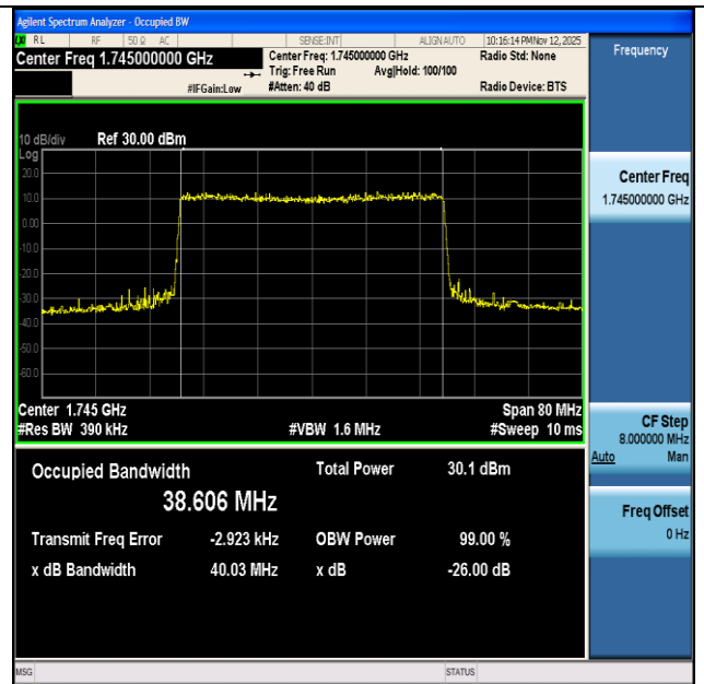
NTNV-n66-PC3-15-40-M-DFT-16QAM-Outer_Full-Ant1-PASS
