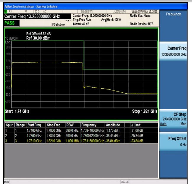
NTNV-n66-PC3-15-40-H-CP-QPSK-Outer_Full-PASS
