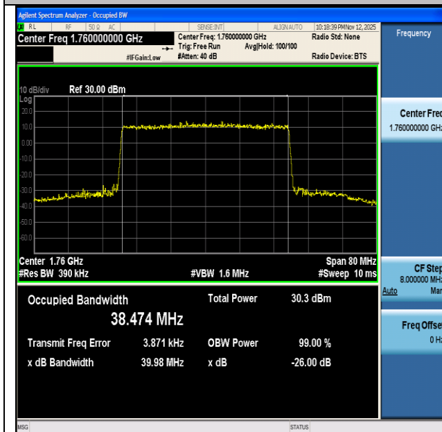
NTNV-n66-PC3-15-40-H-DFT-16QAM-Outer_Full-Ant1-PASS
