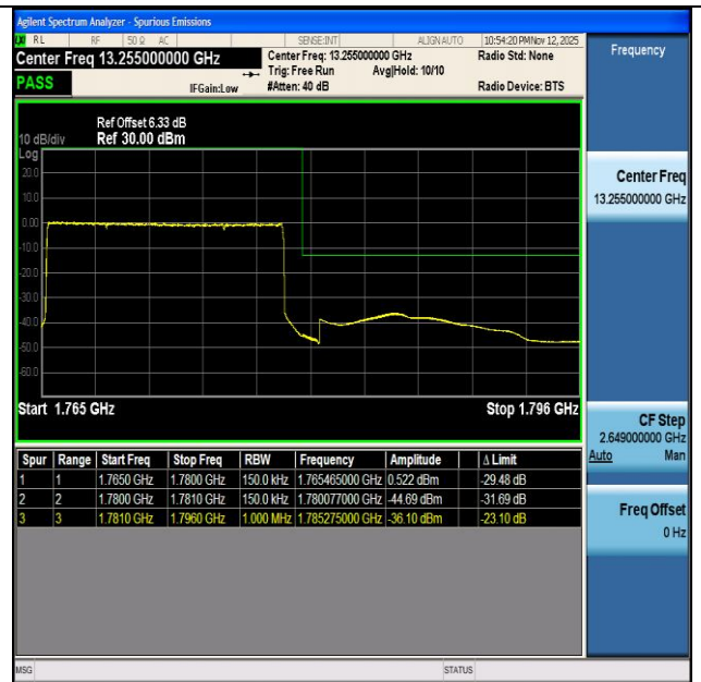
NTNV-n66-PC3-15-15-H-DFT-BPSK-Outer_Full-PASS
