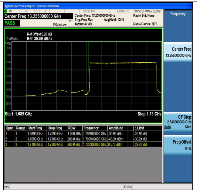
NTNV-n66-PC3-15-20-L-DFT-BPSK-Outer_Full-PASS
