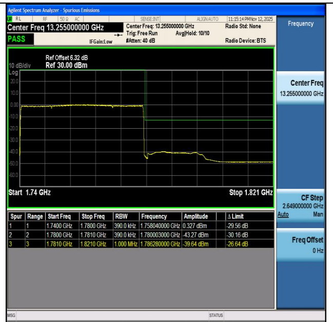
NTNV-n66-PC3-15-40-H-DFT-BPSK-Outer_Full-PASS
