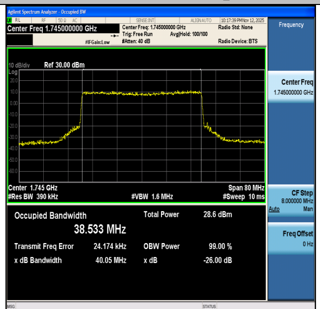
NTNV-n66-PC3-15-40-M-CP-256QAM-Outer_Full-Ant1-PASS
