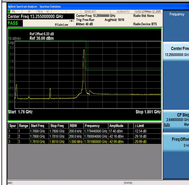
NTNV-n66-PC3-15-20-H-CP-QPSK-Edge_1RB_Right-PASS
