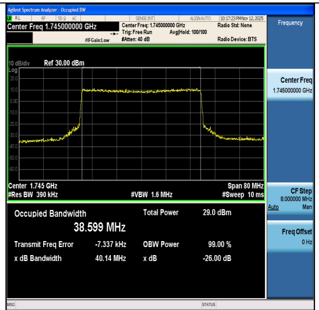
NTNV-n66-PC3-15-40-M-CP-16QAM-Outer_Full-Ant1-PASS
