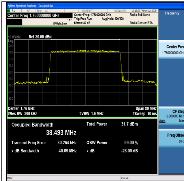
NTNV-n66-PC3-15-40-H-DFT-BPSK-Outer_Full-Ant1-PASS
