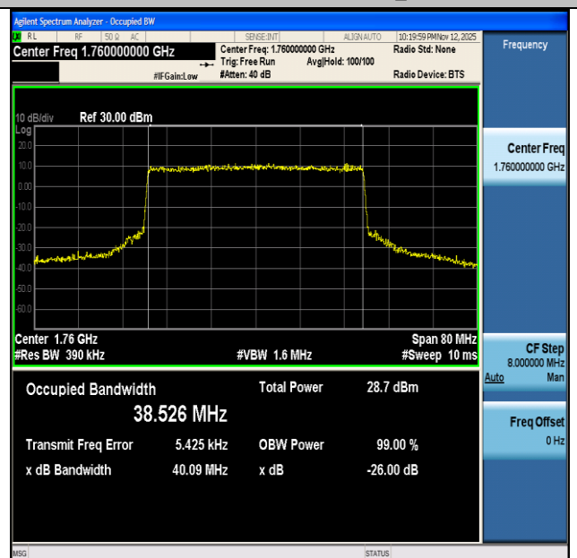
NTNV-n66-PC3-15-40-H-CP-64QAM-Outer_Full-Ant1-PASS
