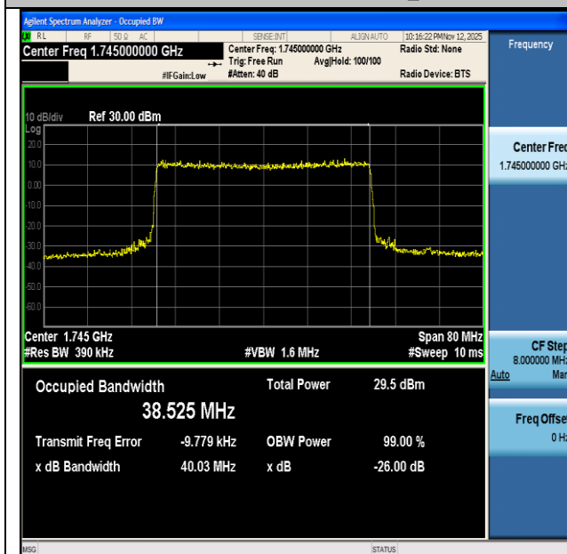
NTNV-n66-PC3-15-40-M-DFT-64QAM-Outer_Full-Ant1-PASS
