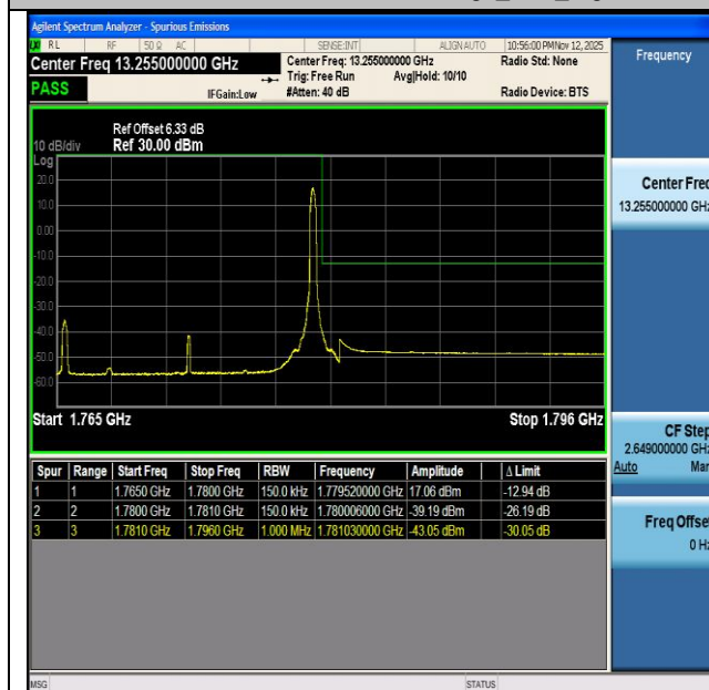
NTNV-n66-PC3-15-15-H-CP-QPSK-Edge_1RB_Right-PASS
