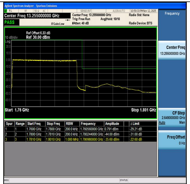
NTNV-n66-PC3-15-20-H-DFT-BPSK-Outer_Full-PASS
