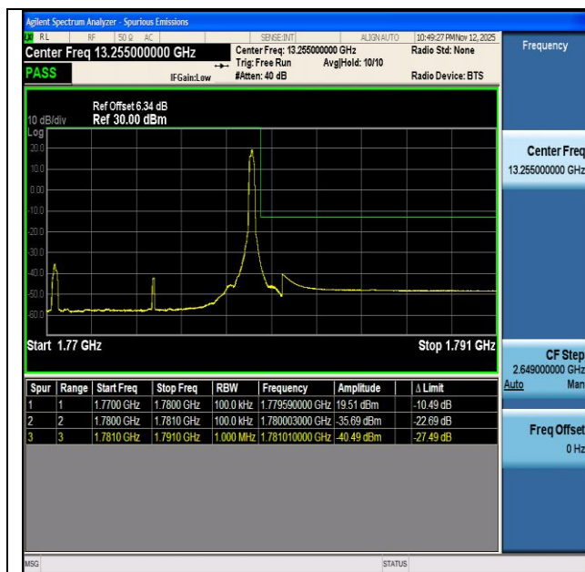
NTNV-n66-PC3-15-10-H-DFT-BPSK-Edge_1RB_Right-PASS
