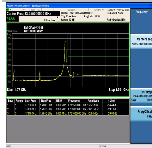
NTNV-n66-PC3-15-10-H-CP-QPSK-Edge_1RB_Right-PASS
