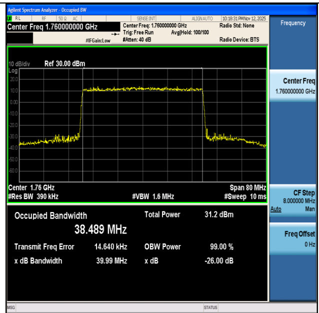
NTNV-n66-PC3-15-40-H-DFT-QPSK-Outer_Full-Ant1-PASS
