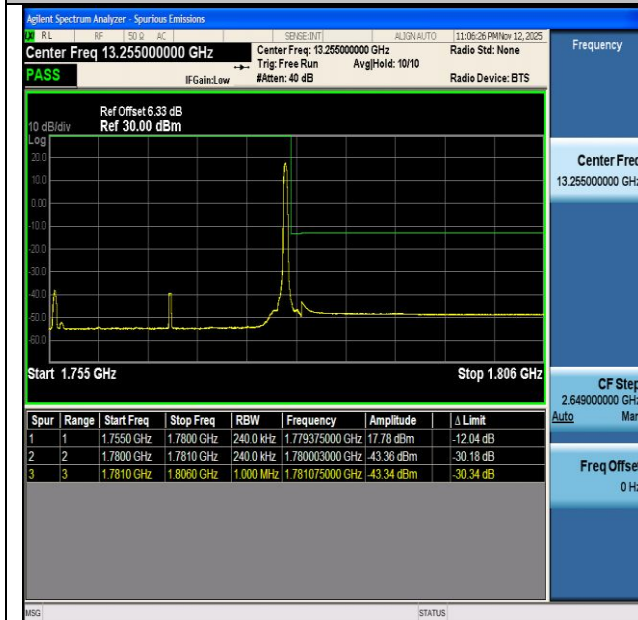
NTNV-n66-PC3-15-25-H-CP-QPSK-Edge_1RB_Right-PASS
