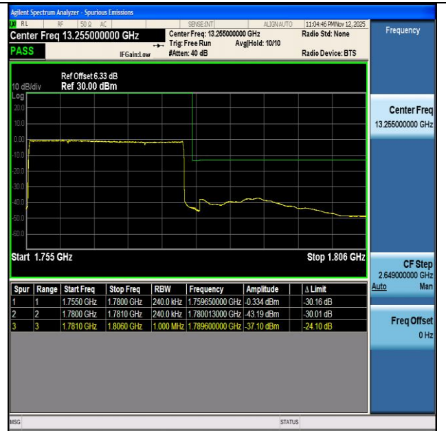
NTNV-n66-PC3-15-25-H-DFT-BPSK-Outer_Full-PASS
