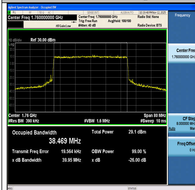
NTNV-n66-PC3-15-40-H-CP-16QAM-Outer_Full-Ant1-PASS
