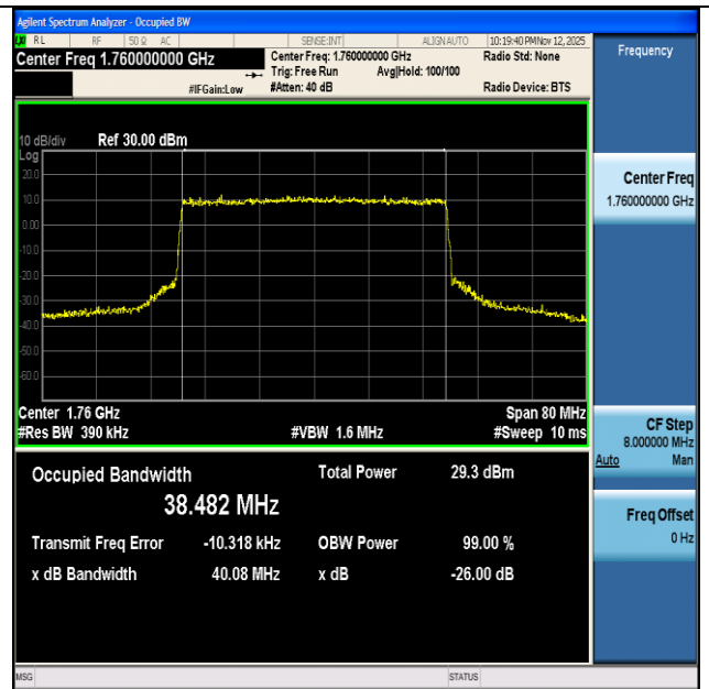
NTNV-n66-PC3-15-40-H-CP-QPSK-Outer_Full-Ant1-PASS
