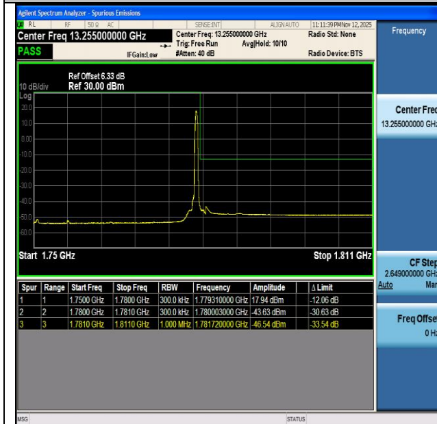
NTNV-n66-PC3-15-30-H-CP-QPSK-Edge_1RB_Right-PASS
