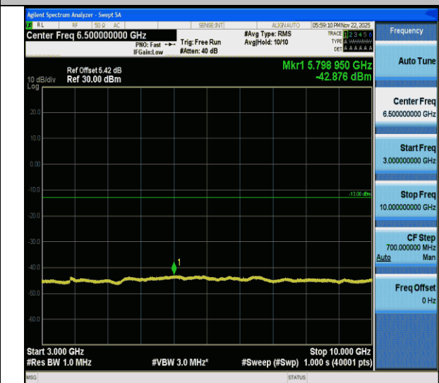
Band26(824-849)-15MHz-QPSK-26915-1RB#0-3000~10000-PASS
