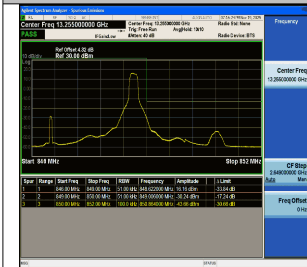
Band26(824-849)-5MHz-QPSK-27015-1RB#24-PASS
