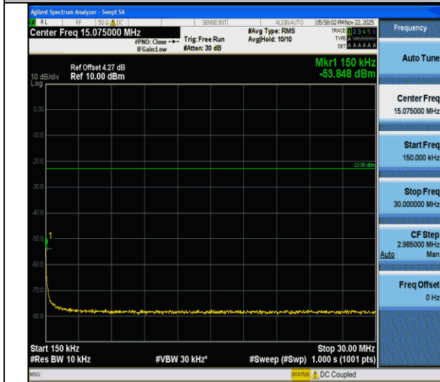
Band26(824-849)-15MHz-QPSK-26915-1RB#0-0.15~30-PASS
