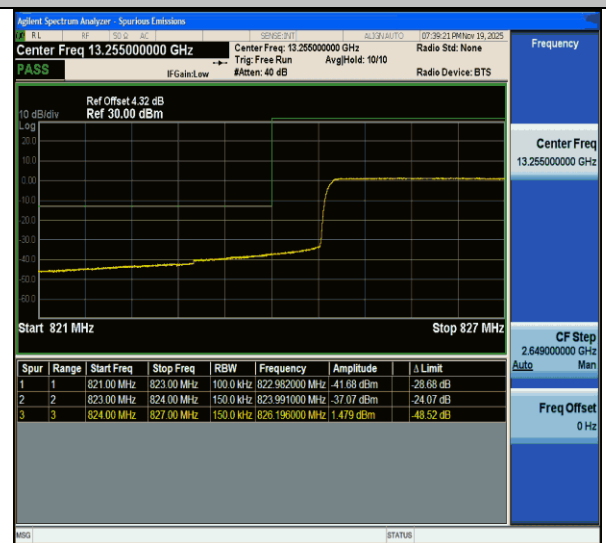
Band26(824-849)-15MHz-QPSK-26865-75RB#0-PASS
