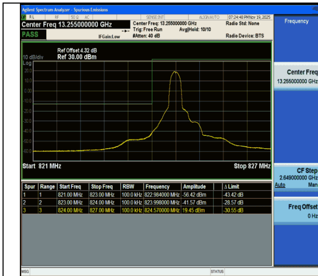
Band26(824-849)-10MHz-QPSK-26840-1RB#0-PASS
