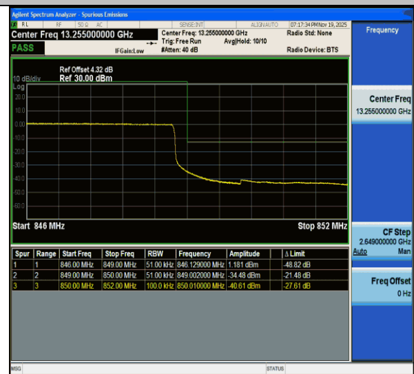
Band26(824-849)-5MHz-QPSK-27015-25RB#0-PASS
