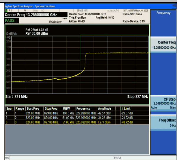
Band26(824-849)-5MHz-QPSK-26815-25RB#0-PASS
