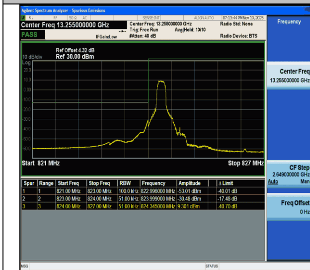
Band26(824-849)-5MHz-QPSK-26815-1RB#0-PASS
