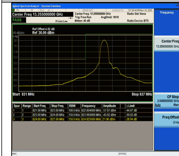
Band26(824-849)-15MHz-QPSK-26865-1RB#0-PASS
