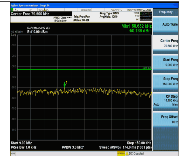
Band26(824-849)-15MHz-QPSK-26915-1RB#0-0.009~0.15-PASS
