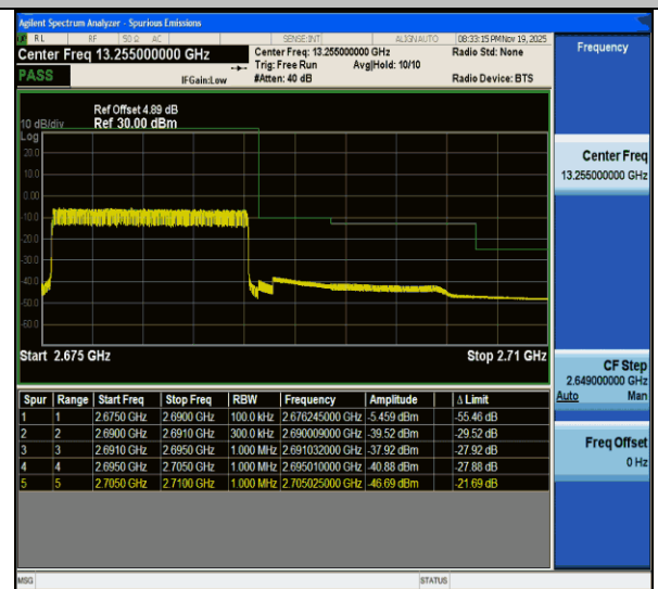
Band41-15MHz-QPSK-41515-75RB#0-PASS
