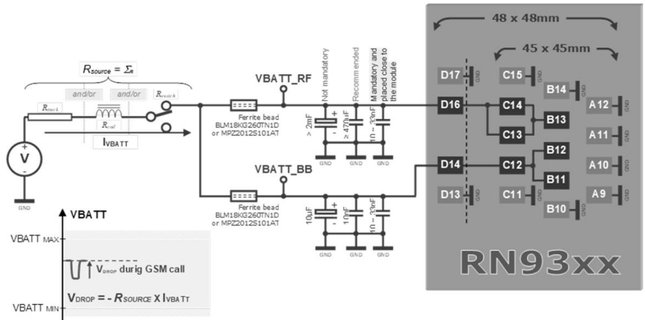
Figure 3-1 Power Recommendation
