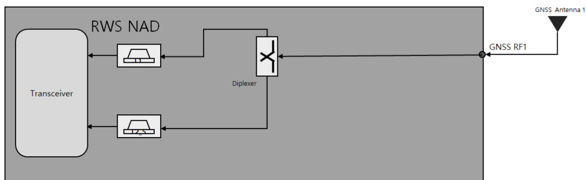
Figure 2-1 RN93V GNSS Block Diagram
