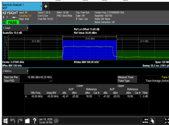
N48(40M)_DFT-s-OFDM_PI_2- BPSK_Outer_Full_Low_CH
