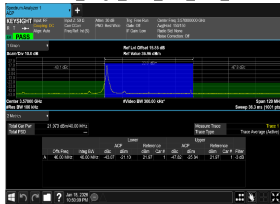
N48(40M)_DFT-s-OFDM_PI_2- BPSK_Edge_1RB_Left_Low_CH
