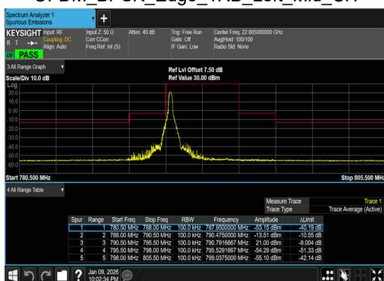
N14(5M)_DFT-s- OFDM_BPSK_Edge_1RB_Left_Mid_CH
