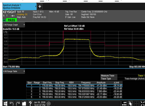
N14(5M)_DFT-s- OFDM_QPSK_Outer_Full_Low_CH
