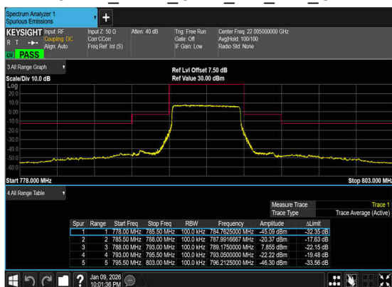
N14(5M)_DFT-s- OFDM_BPSK_Outer_Full_Low_CH
