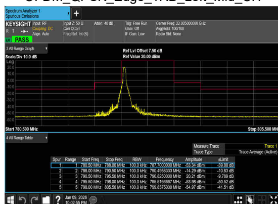
N14(5M)_DFT-s- OFDM_QPSK_Edge_1RB_Left_Mid_CH
