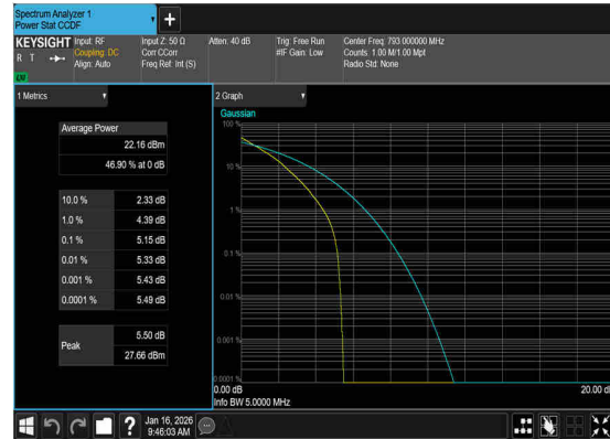
N14(5M)_DFT-s- OFDM_QPSK_Outer_Full_Mid_CH
