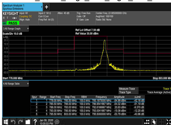
N14(5M)_DFT-s- OFDM_BPSK_Edge_1RB_Right_Low_CH
