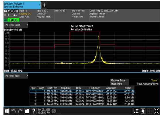
N14(10M)_DFT-s- OFDM_QPSK_Edge_1RB_Right_Mid_CH
