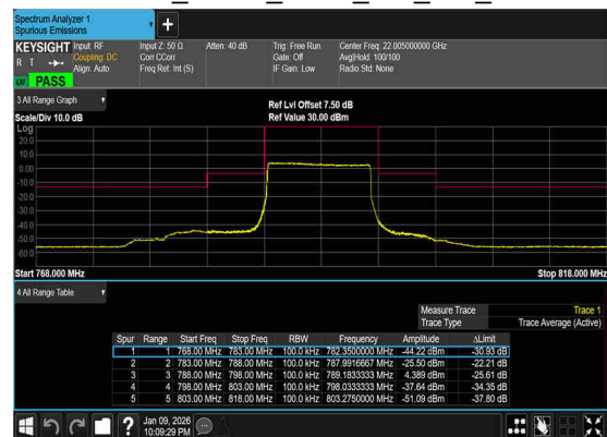
N14(10M)_DFT-s- OFDM_QPSK_Outer_Full_Mid_CH
