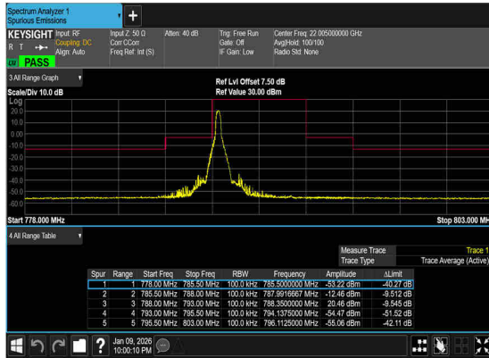
N14(5M)_DFT-s- OFDM_BPSK_Edge_1RB_Left_Low_CH
