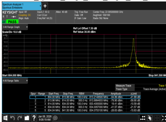
N26(20M)_DFT-s- OFDM_QPSK_Edge_1RB_Right_Mid_CH
