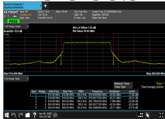
N26(5M)_DFT-s- OFDM_BPSK_Outer_Full_High_CH
