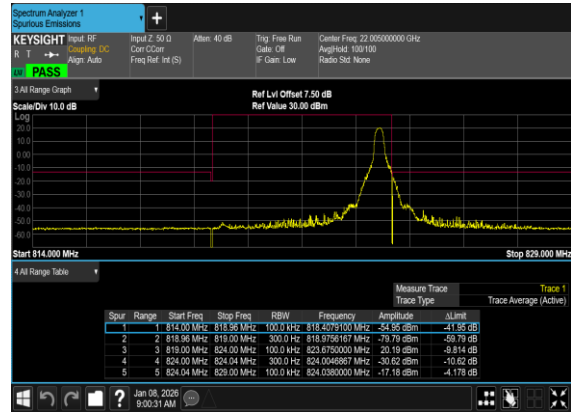
N26(5M)_DFT-s- OFDM_BPSK_Edge_1RB_Right_High_CH
