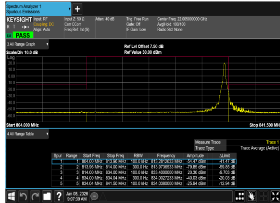
N26(20M)_DFT-s- OFDM_BPSK_Edge_1RB_Right_Mid_CH
