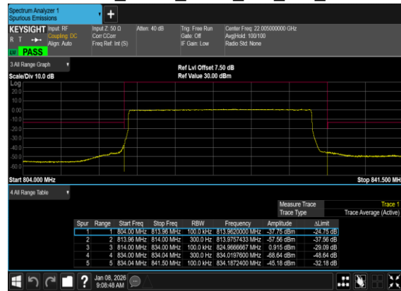
N26(20M)_DFT-s- OFDM_BPSK_Outer_Full_Mid_CH
