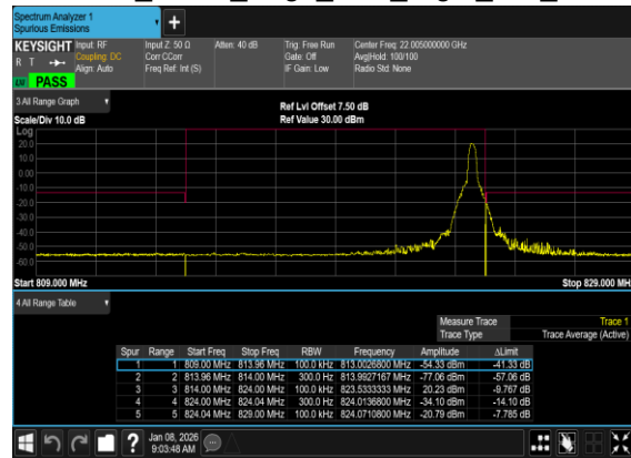
N26(10M)_DFT-s- OFDM_BPSK_Edge_1RB_Right_Mid_CH
