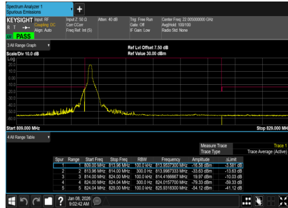
N26(10M)_DFT-s- OFDM_BPSK_Edge_1RB_Left_Mid_CH
