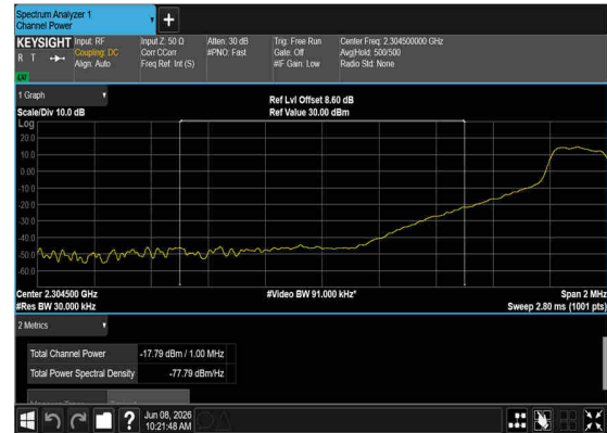
N30(10M)_DFT-s- OFDM_BPSK_Edge_1RB_Left_Low_CH_CHP_PASS
