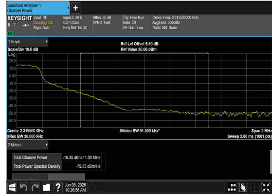
N30(10M)_DFT-s- OFDM_BPSK_Edge_1RB_Right_Low_CH_CHP_PASS
