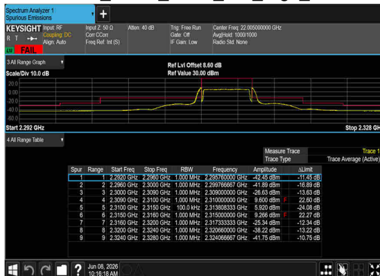
N30(5M)_DFT-s- OFDM_BPSK_Outer_Full_High_CH
