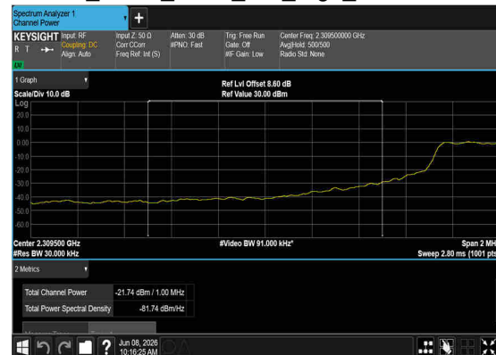
N30(5M)_DFT-s- OFDM_BPSK_Outer_Full_High_CH_CHP_PASS
