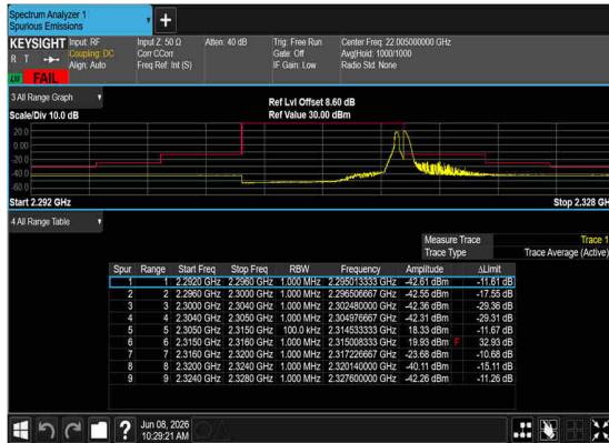
N30(10M)_DFT-s- OFDM_QPSK_Edge_1RB_Right_Low_CH
