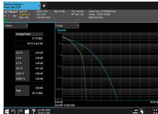
N30(10M)_DFT-s- OFDM_QPSK_Outer_Full_Low_CH
