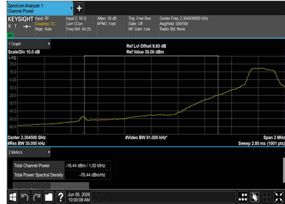
N30(5M)_DFT-s- OFDM_BPSK_Edge_1RB_Left_Low_CH_CHP_PASS
