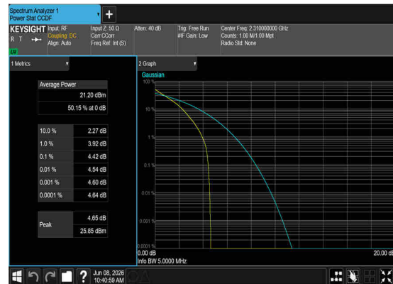
N30(5M)_DFT-s- OFDM_QPSK_Outer_Full_Mid_CH
