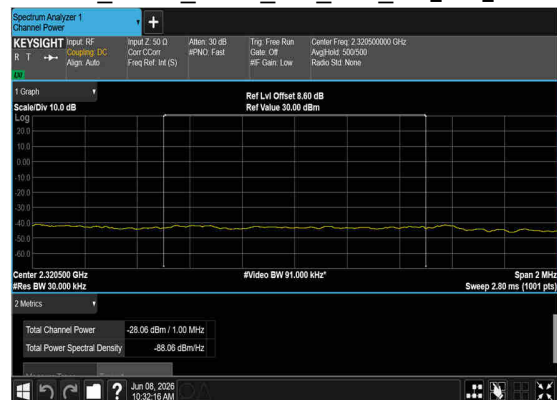
N30(10M)_DFT-s- OFDM_BPSK_Outer_Full_Low_CH_CHP_PASS
