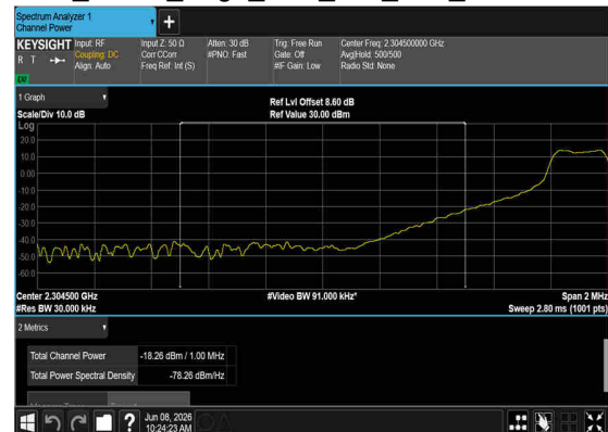
N30(10M)_DFT-s- OFDM_QPSK_Edge_1RB_Left_Low_CH_CHP_PASS
