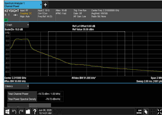
N30(5M)_DFT-s- OFDM_QPSK_Edge_1RB_Right_High_CH_CHP_PASS
