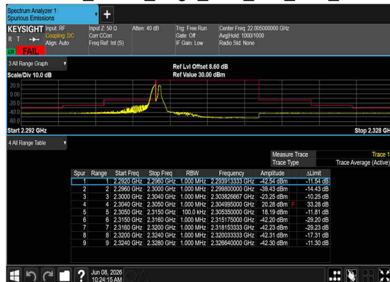
N30(10M)_DFT-s- OFDM_QPSK_Edge_1RB_Left_Low_CH
