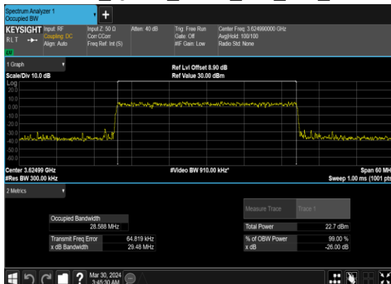
N48(30M)_CP- OFDM_QPSK_Outer_Full_Mid_CH
