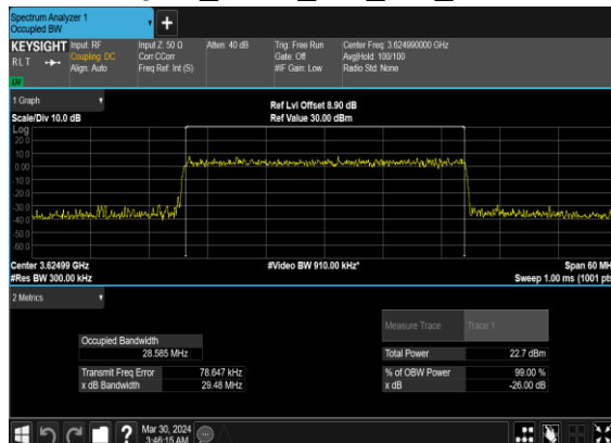
N48(30M)_CP-OFDM_16 QAM_Outer_Full_Mid_CH
