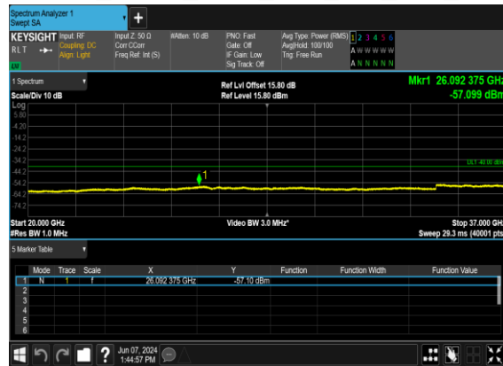
B2_N48(5M)_DFT-s-OFDM_QPSK_Edge_1RB_Left_Low_CH
