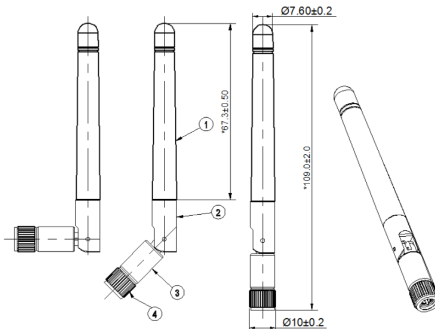
Antenna Dimensions
