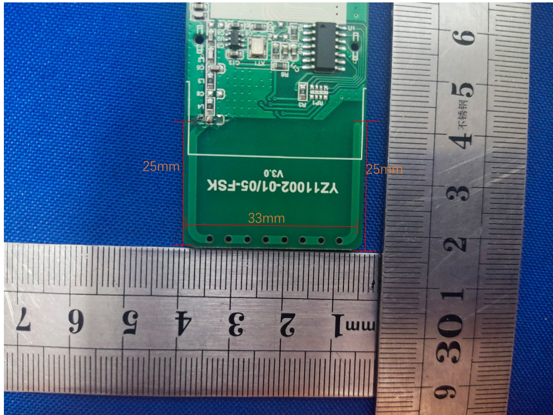
Antenna Size
