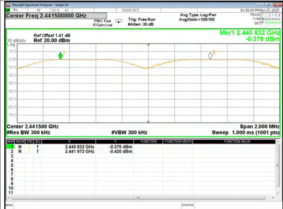
CFS NVNT 1-DH5 2441MHz Ant1
