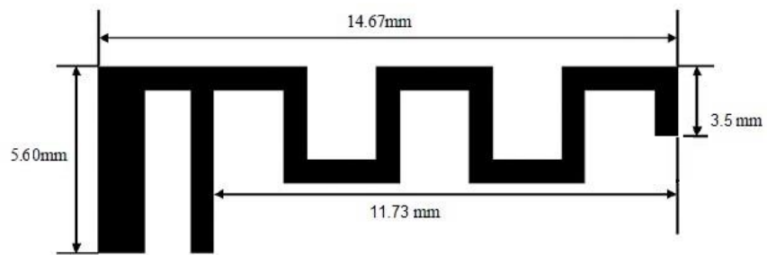
Antenna Photo & Length (mm)
