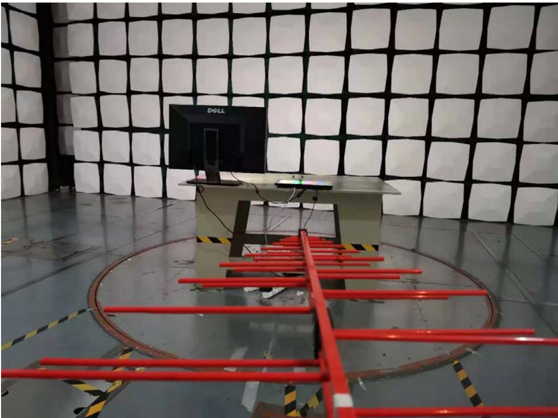
Radiated Emission Below 1GHz Rear View- MGYR15
