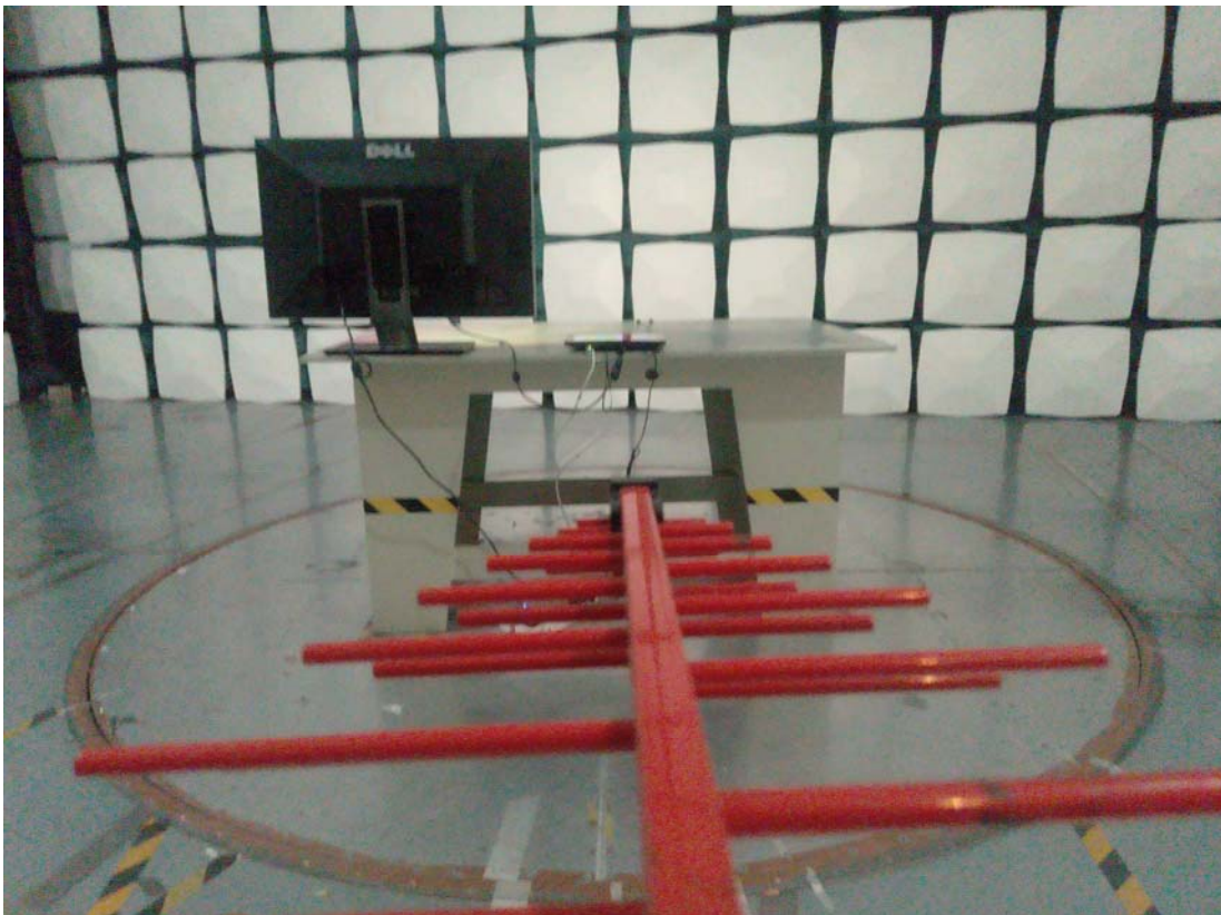
Radiated Emission Below 1GHz Rear View- MGYR10
