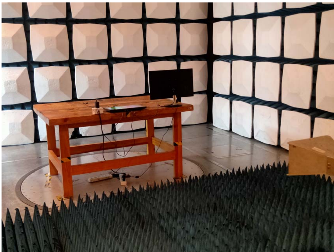
Radiated Emission Above 1GHz Rear View- MGYR15
