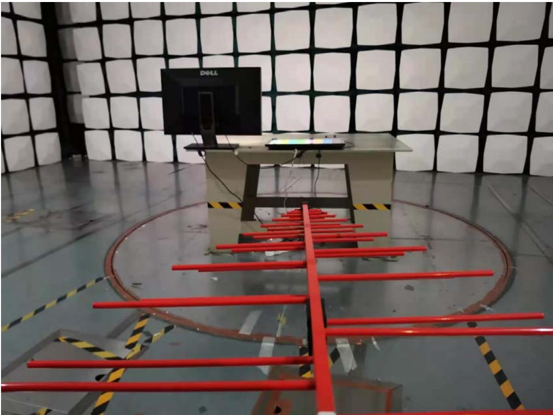
Radiated Emission Below 1GHz Rear View- MGYR21
