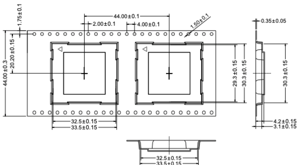
Figure 11 Tape Specifications
