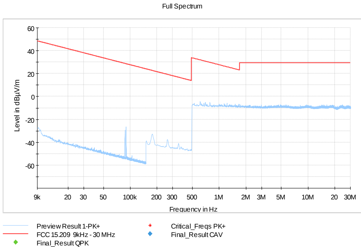
Figure 3. Measured curve with peak detector (Mid channel).
