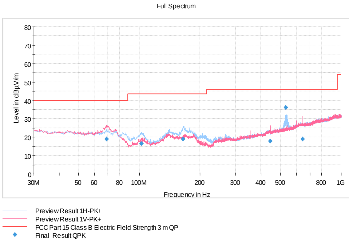
Figure 4. Measured curve with peak detector (Mid channel).
