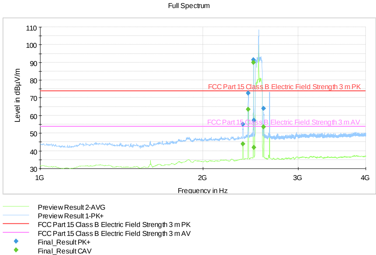
Figure 7. Measured curve with peak and average detectors (High channel).
