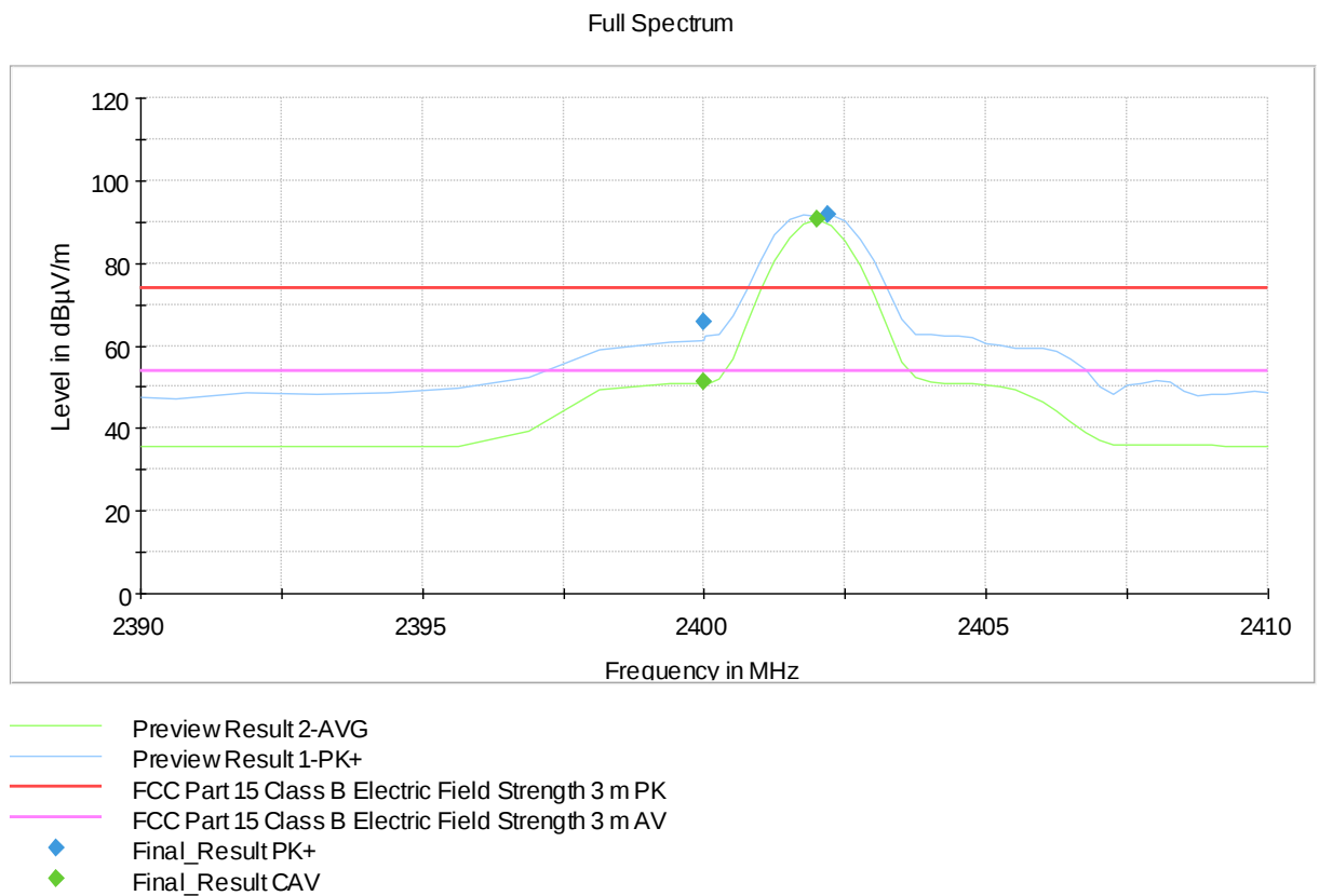
Figure 6. Measured curve with peak and average detectors (Low channel).
