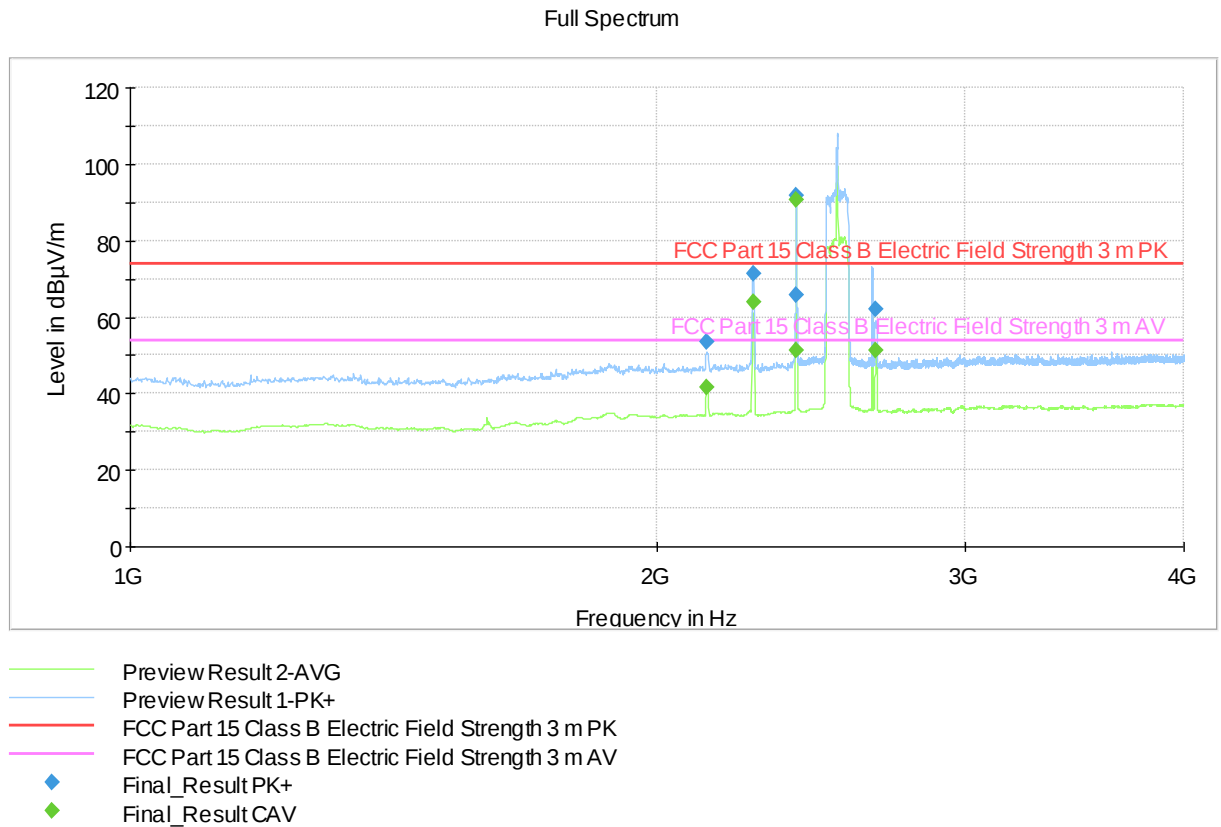
Figure 5. Measured curve with peak and average detectors (Low channel).
