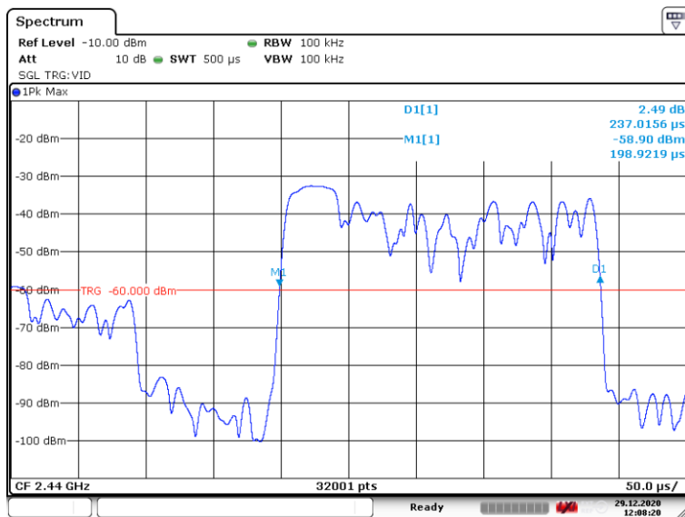
Figure 13. Pulse length
