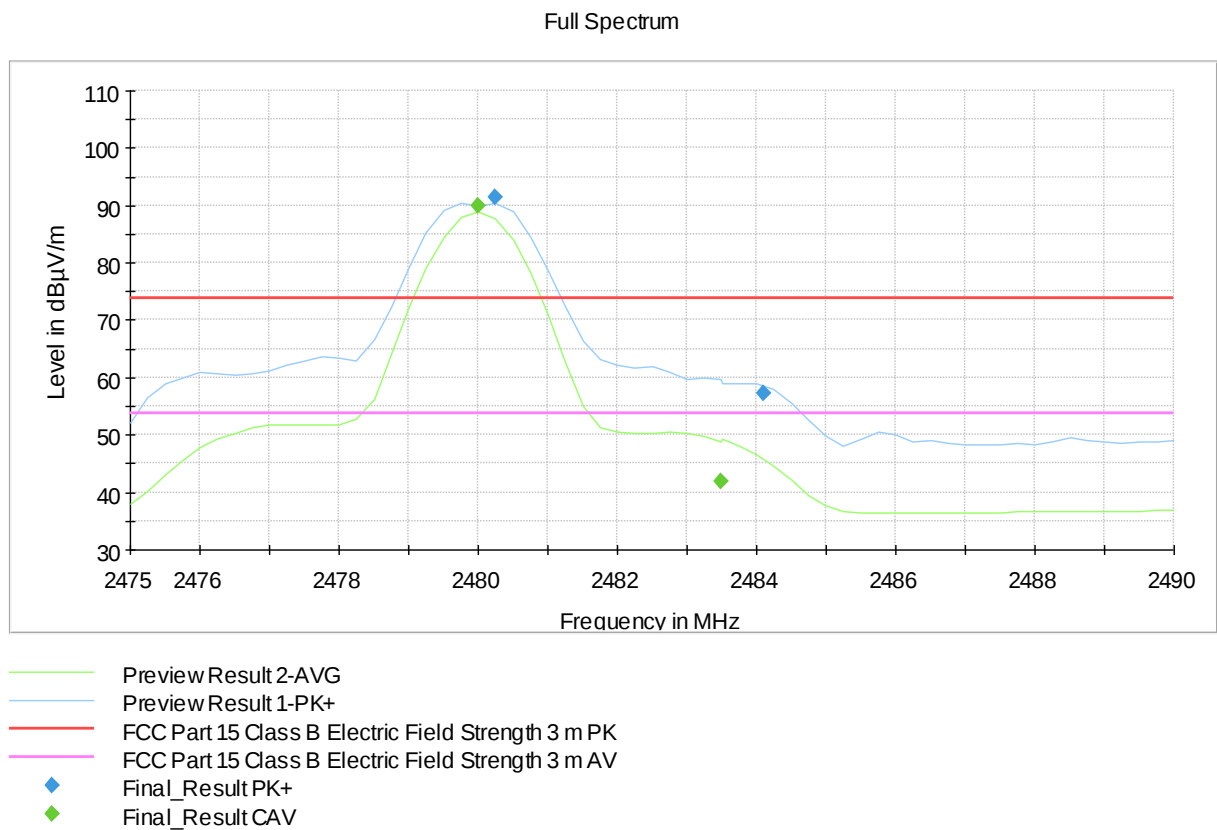
Figure 8. Measured curve with peak and average detectors (High channel).
