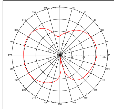
Far-field amplitude of ANTENNA H.nsi
