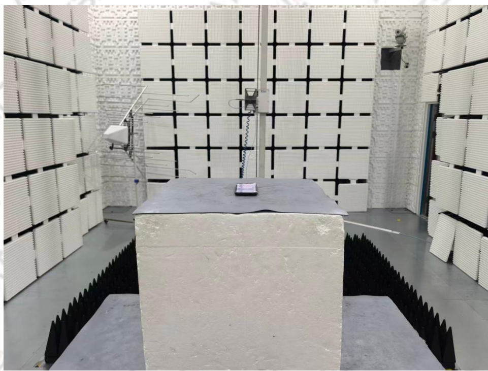
Above 1GHz
