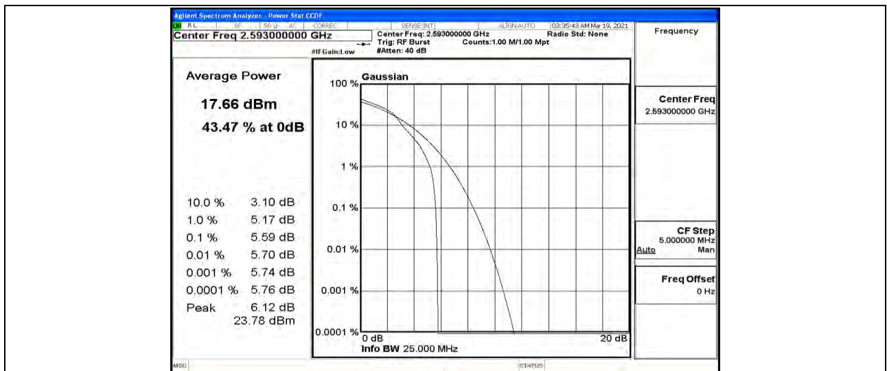
Band41-10MHz-16QAM-40620-50RB#0
