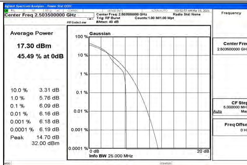
Band41-15MHz-QPSK-39725-75RB#0
