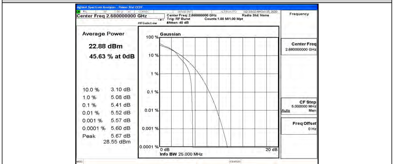
Band41-20MHz-16QAM-41490-100RB#0
