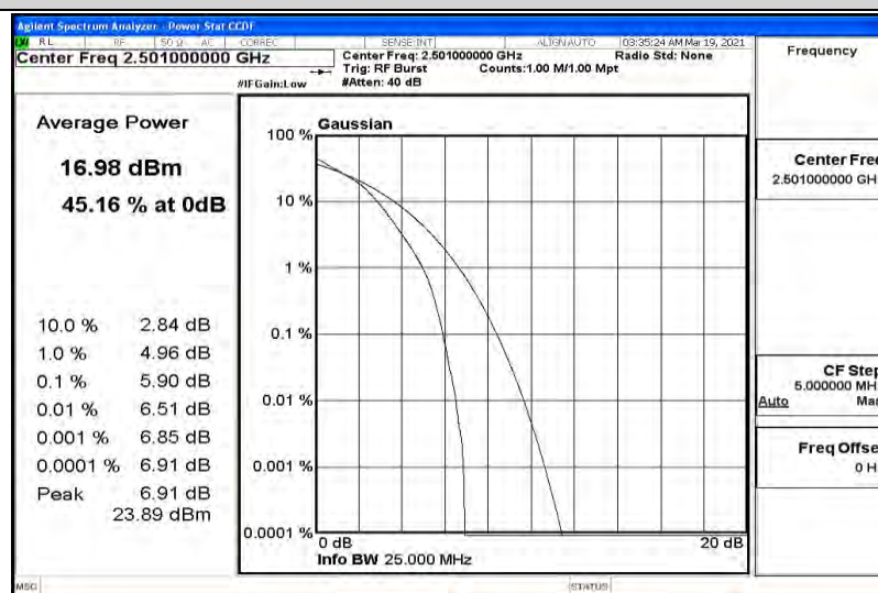
Band41-10MHz-16QAM-40620-1RB#0
