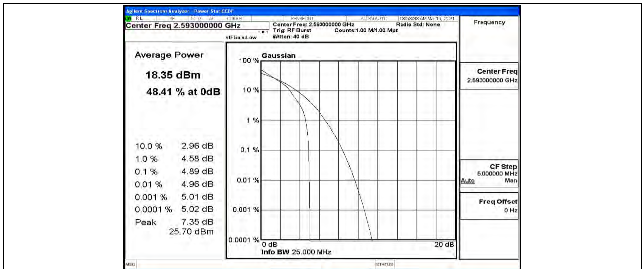
Band41-15MHz-QPSK-40620-75RB#0
