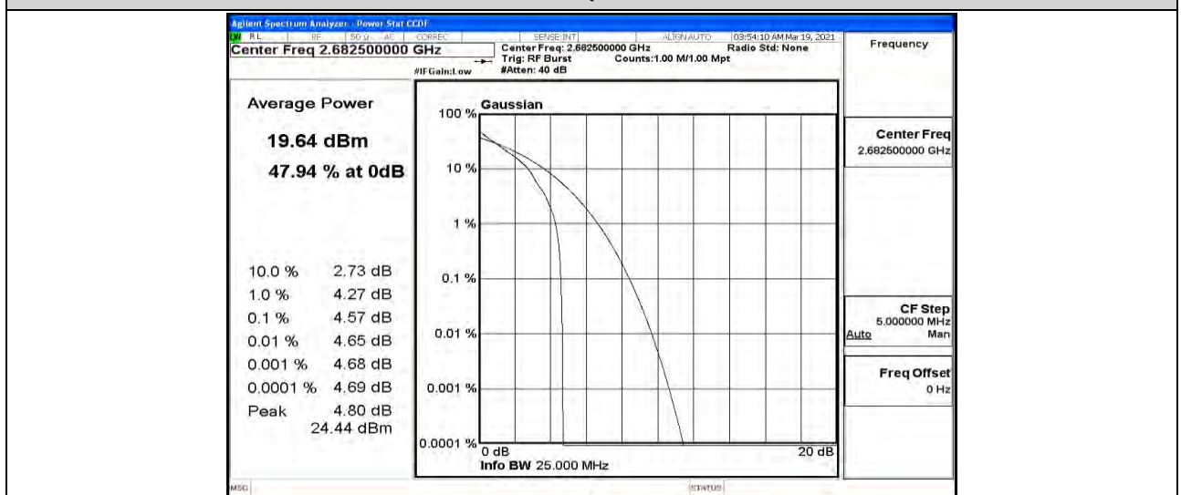
Band41-15MHz-QPSK-41515-75RB#0
