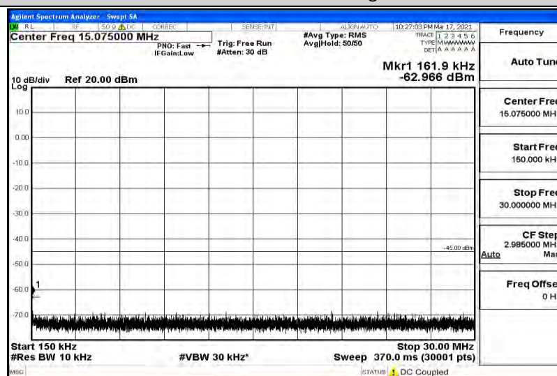
Band41-20MHz-16QAM-L-1RB#0-Range3:30~1000MHz
