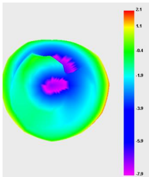
ANT1: 1900Mhz
