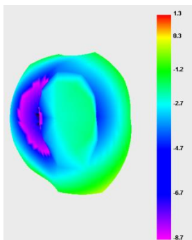
ANT2: 2100Mhz
