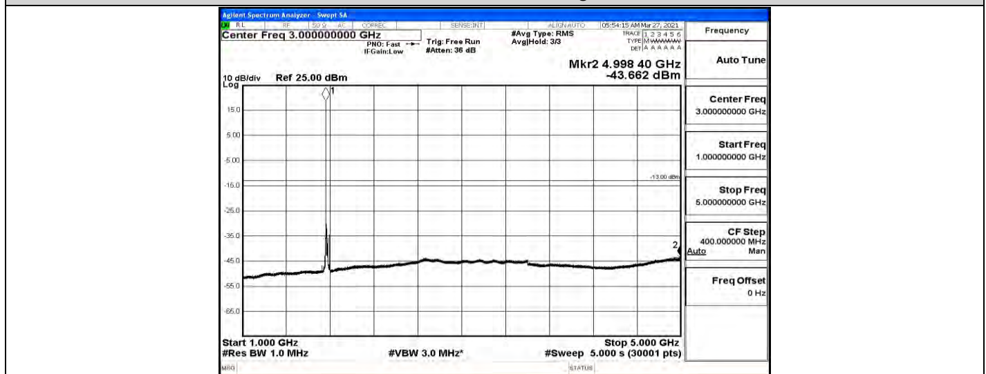
Band66-20MHz-QPSK-132572-1RB#0-Range5:5000~12000MHz
