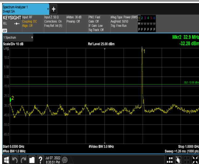
Band17-10MHz-16QAM-23780-1RB#0-Range2:30~1000MHz
