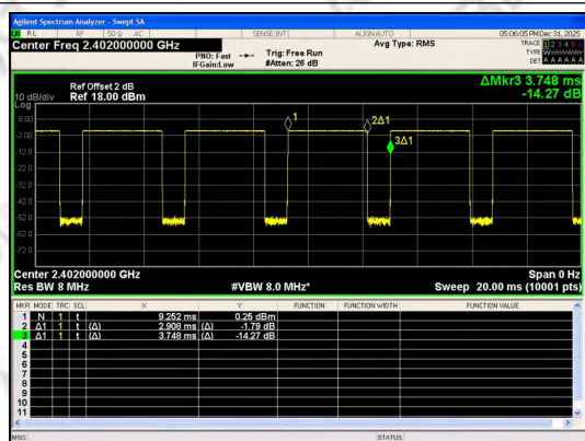
GFSK(DH5)_Channel 0
