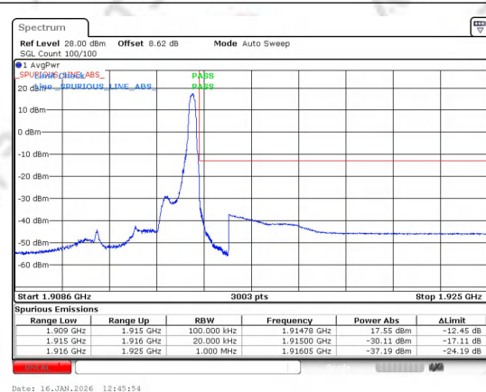
Band 25 1.4MHz/1914.3/High QPSK 6@0
