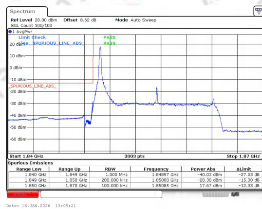
Band 25 15MHz/1857.5/Low QPSK 1@74
