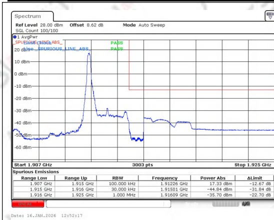
Band 25 3MHz/1913.5/High 16QAM 1@0
