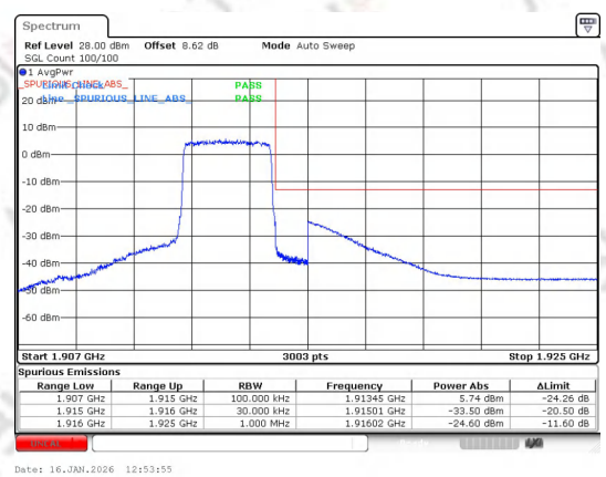
Band 25 3MHz/1913.5/High 16QAM 1@14
