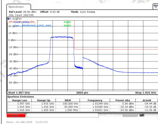
Band 25 3MHz/1913.5/High 16QAM 1@0
