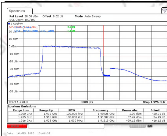
Band 25 10MHz/1910.0/High 16QAM 50@0
