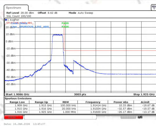
Band 25 1.4MHz/1914.3/High QPSK 1@0
