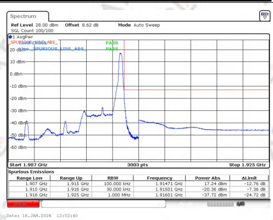
Band 25 3MHz/1913.5/High 16QAM 1@14
