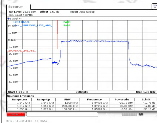
Band 25 15MHz/1857.5/Low QPSK 1@0
