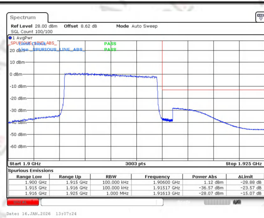
Band 25 10MHz/1910.0/High 64QAM 50@0
