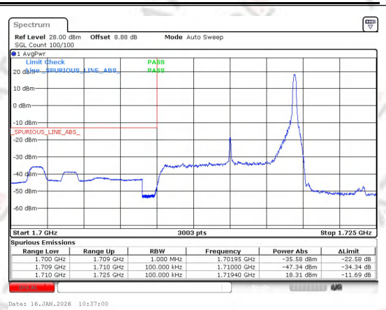
Band 4 10MHz/1715.0/Low QPSK 1@49
