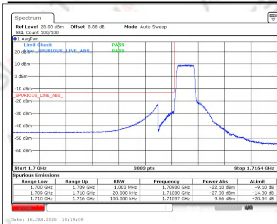
Band 4 1.4MHz/1710.7/Low 64QAM 6@0
