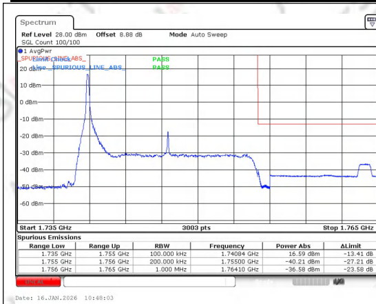
Band 4 15MHz/1747.5/High 16QAM 1@0
