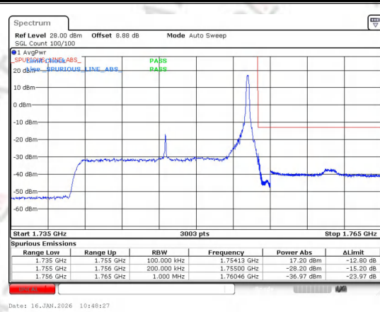
Band 4 15MHz/1747.5/High 16QAM 1@74
