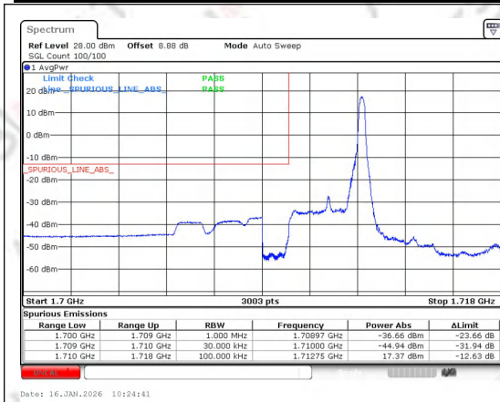
Band 4 3MHz/1711.5/Low 16QAM 1@14
