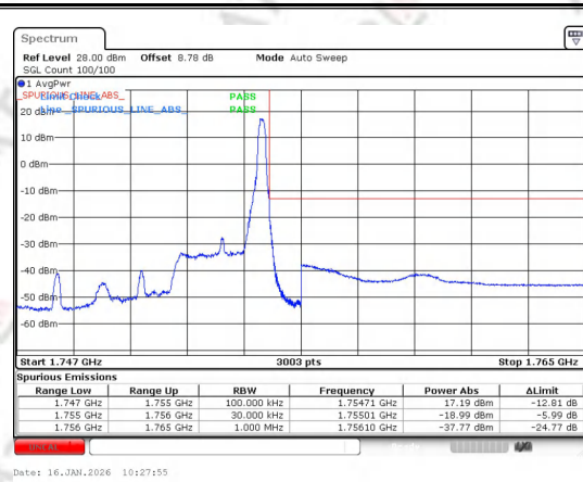
Band 4 3MHz/1753.5/High 16QAM 1@14
