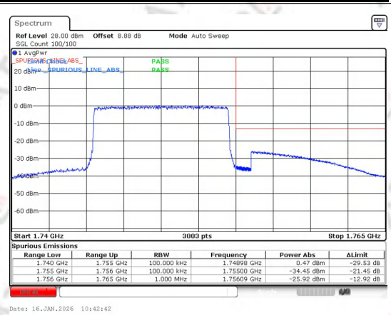
Band 4 10MHz/1750.0/High 64QAM 50@0
