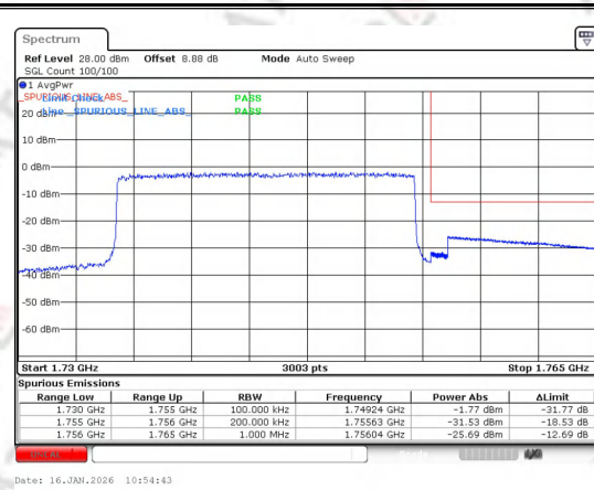
Band 4 20MHz/1745.0/High QPSK 100@0
