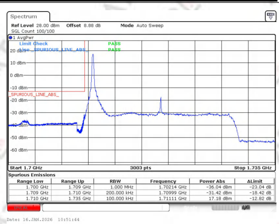
Band 4 20MHz/1720.0/Low 16QAM 1@0
