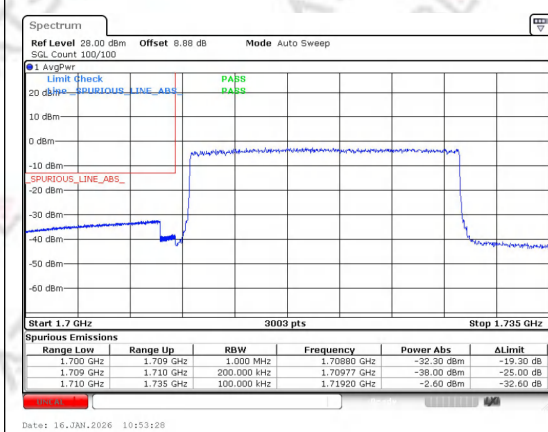
Band 4 20MHz/1720.0/Low 16QAM 1@99
