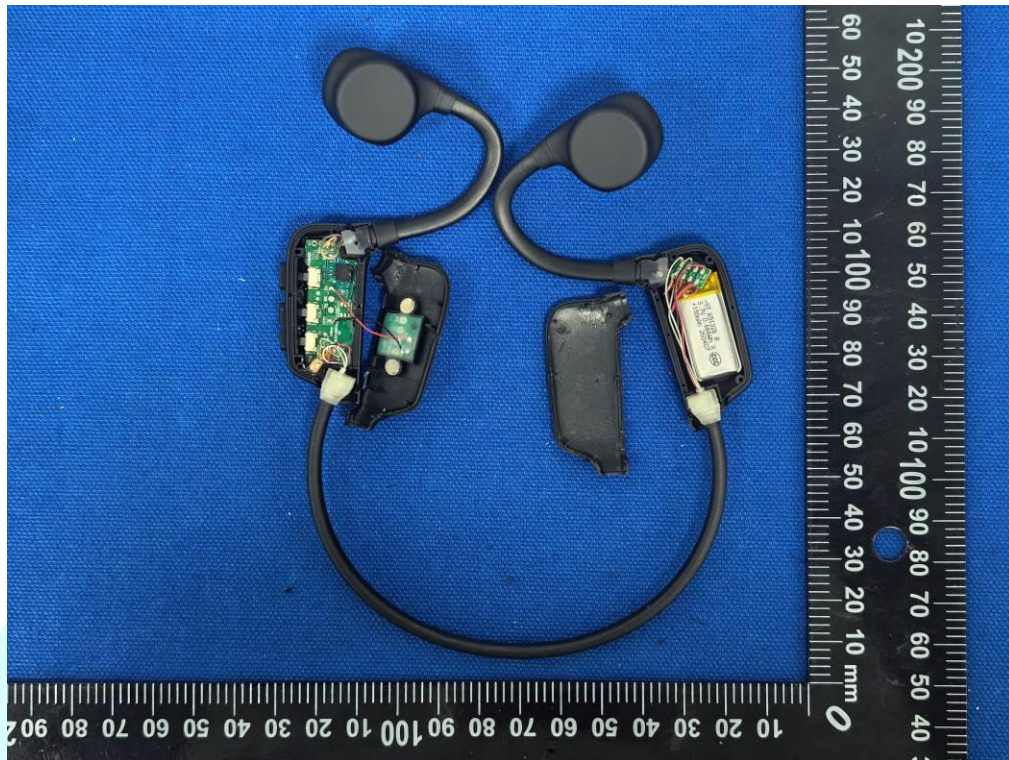
EUT Internal Photos
