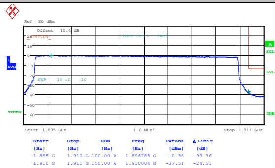
Band2_15MHz_16QAM_19125_1RB#74
