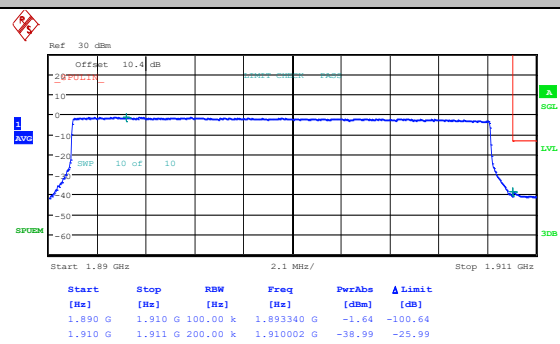
Band2_20MHz_16QAM_19100_1RB#99
