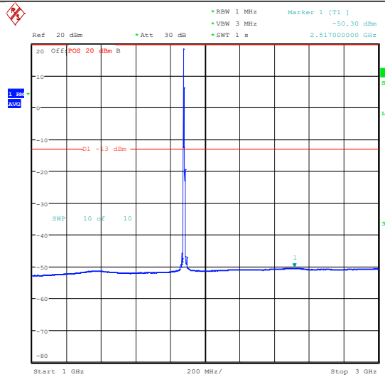
Band2_10MHz_QPSK_19150_1RB#0_1000~3000_1000~3000
