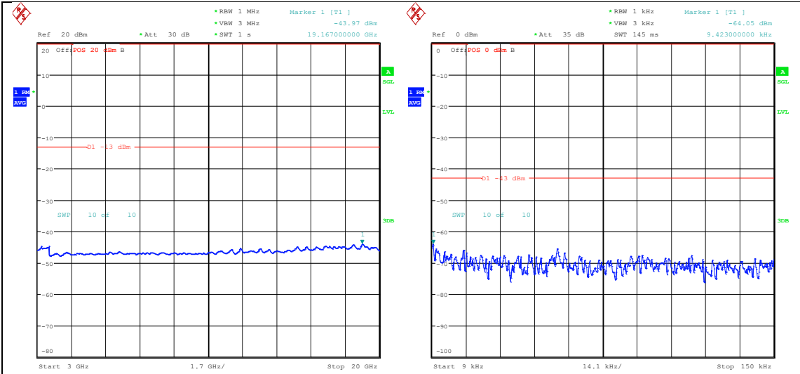
Date: 9.MAY.2024 12:40:35 Band25_10MHz_QPSK_26640_1RB#0_3000~20000_3000~20000 Date: 9.MAY.2024 12:40:43 Band25_10MHz_16QAM_26640_1RB#0_0.009~0.15_0.009~0.15
