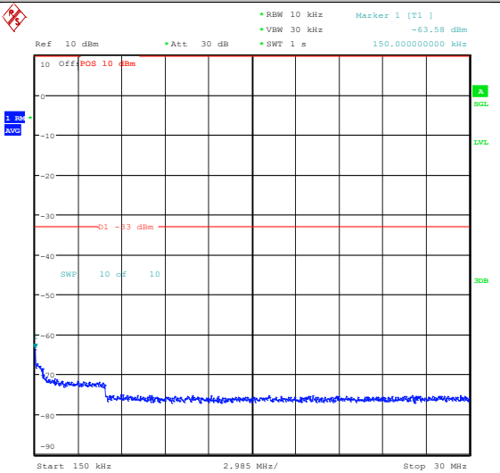
Band25_5MHz_16QAM_26365_1RB#0_3000~20000_00_3000~20000
