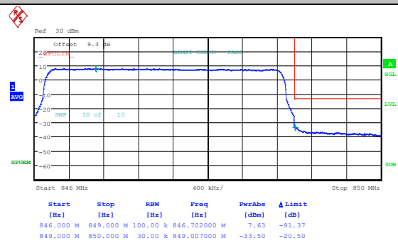
Band26_3MHz_16QAM_27025_1RB#14
