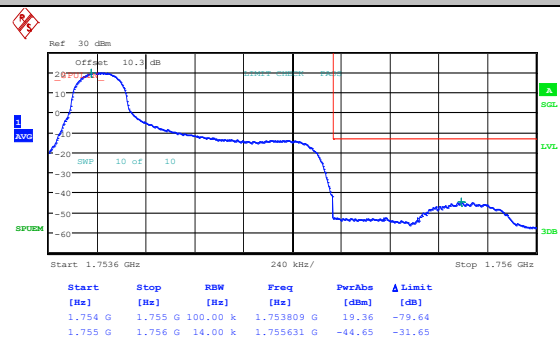
Band4_1.4MHz_16QAM_19957_6RB#0
