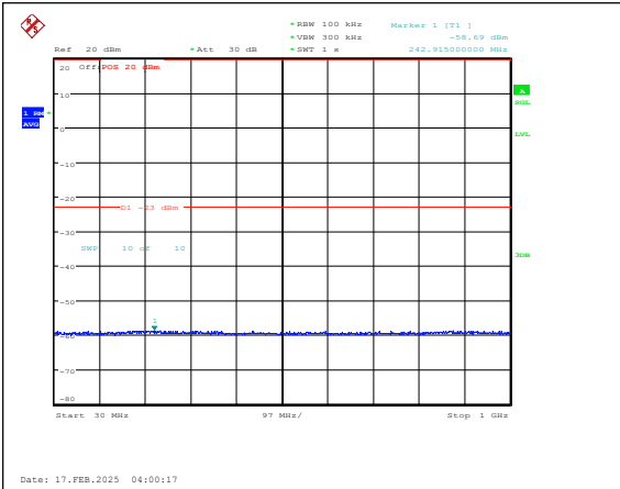
Band25-10MHz-QPSK-26640-1RB#0-30~1000-P ASS
