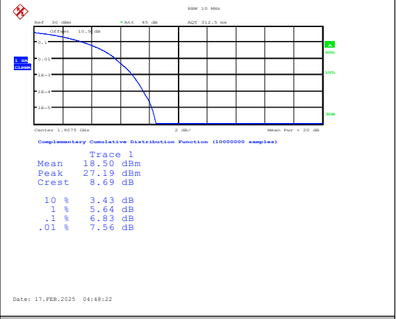
Band25-15MHz-16QAM-26615-75RB#0-PASS
