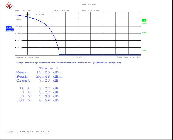
Band25-15MHz-QPSK-26615-75RB#0-PASS
