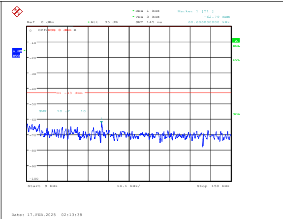
Band25-1.4MHz-16QAM-26047-1RB#0-0.009~0.1 5-PASS
