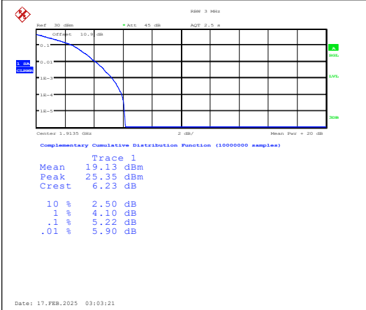
Band25-3MHz-QPSK-26675-1RB#0-PASS
