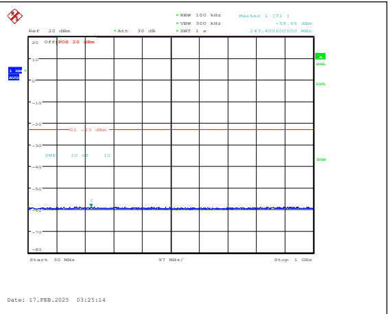
Band25-5MHz-16QAM-26365-1RB#0-30~1000-PA SS
