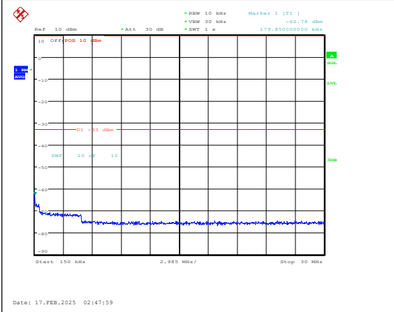
Band25-3MHz-16QAM-26055-1RB#0-0.15~30-PA SS
