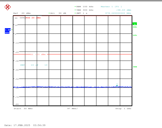
Band25-10MHz-16QAM-26090-1RB#0-30~1000-P ASS
