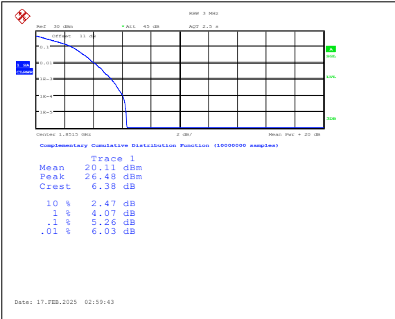
Band25-3MHz-QPSK-26055-1RB#0-PASS
