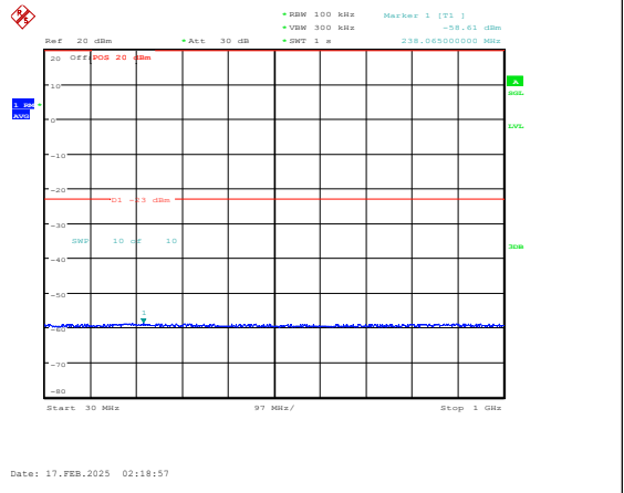
Band25-1.4MHz-16QAM-26683-1RB#0-30~1000-P ASS
