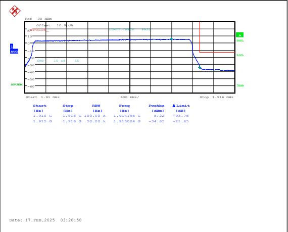
Band25-5MHz-16QAM-26665-25RB#0-PASS
