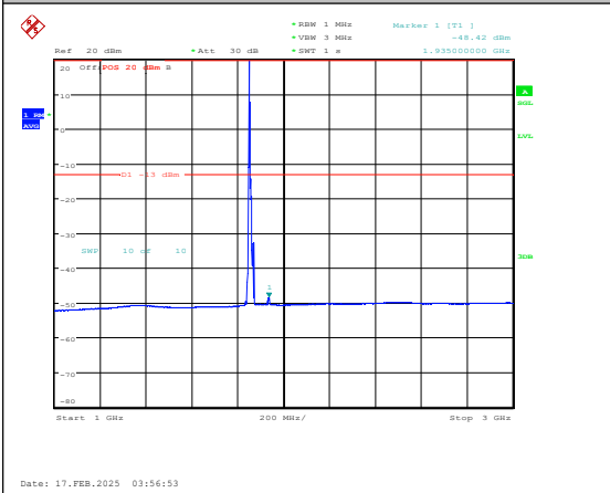
Band25-10MHz-16QAM-26090-1RB#0-1000~300 0-PASS
