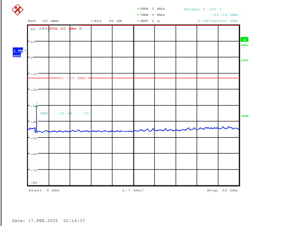
Band25-1.4MHz-16QAM-26047-1RB#0-3000~200 00-PASS
