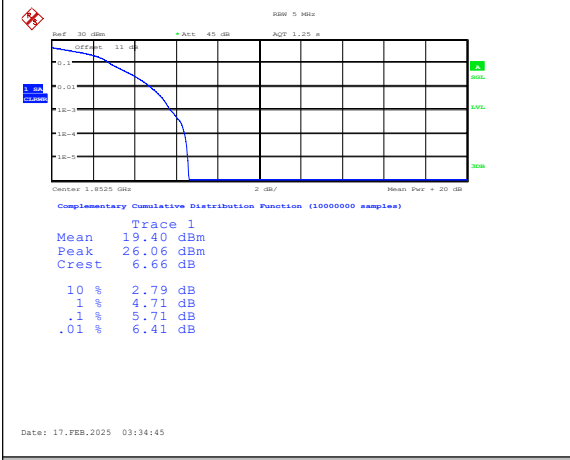
Band25-5MHz-16QAM-26065-1RB#0-PASS
