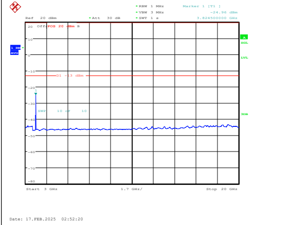
Band25-3MHz-QPSK-26675-1RB#0-3000~20000 -PASS
