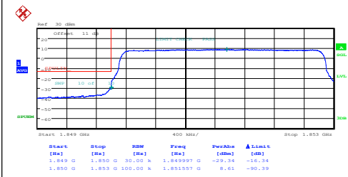
Band25-3MHz-QPSK-26055-1RB#0-PASS
