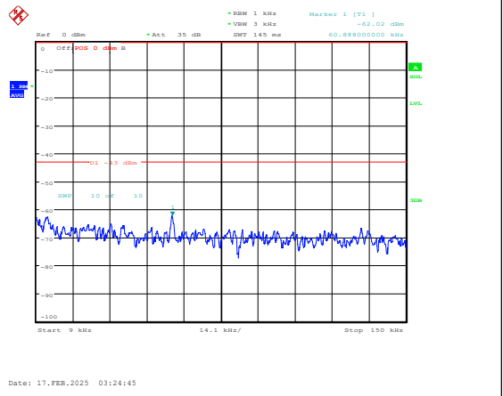
Band25-5MHz-16QAM-26365-1RB#0-0.009~0.15-PASS
