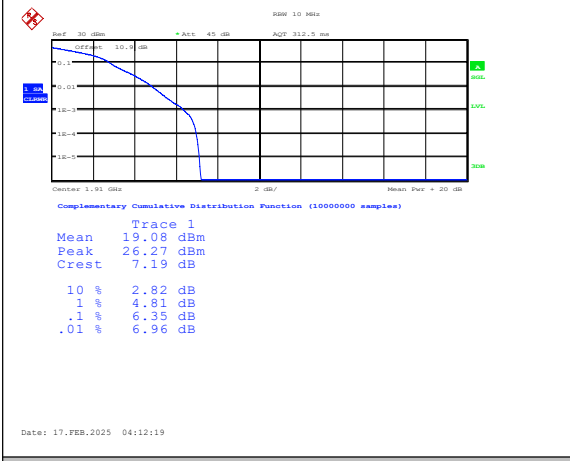
Band25-10MHz-16QAM-26640-1RB#0-PASS
