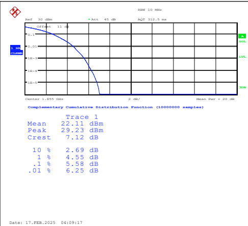
Band25-10MHz-QPSK-26090-50RB#0-PASS
