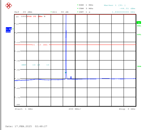
Band25-3MHz-16QAM-26055-1RB#0-1000~3000 -PASS
