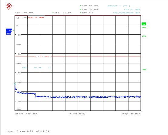
Band25-1.4MHz-16QAM-26047-1RB#0-0.15~30-PASS
