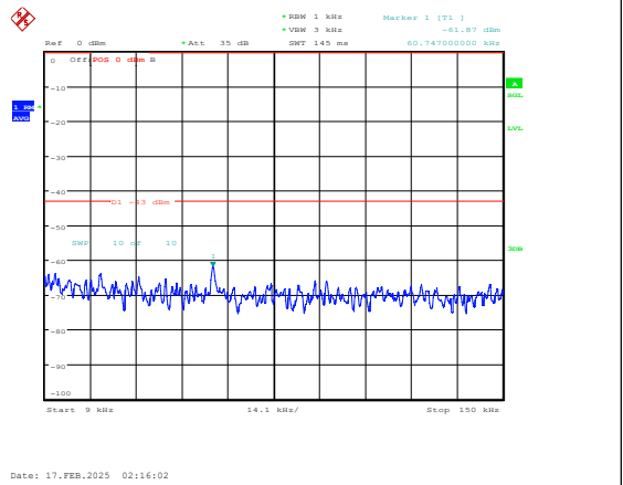
Band25-1.4MHz-16QAM-26365-1RB#0-0.009~0.1 5-PASS
