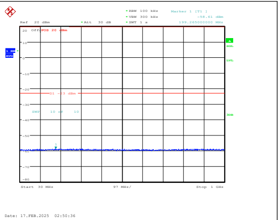
Band25-3MHz-16QAM-26365-1RB#0-30~1000-PA SS
