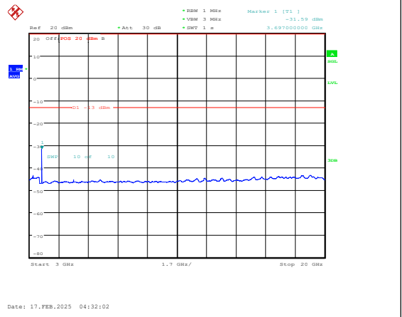
Band25-15MHz-16QAM-26115-1RB#0-3000~2000 0-PASS
