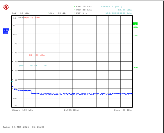
Band25-1.4MHz-QPSK-26365-1RB#0-0.15~30-PA SS
