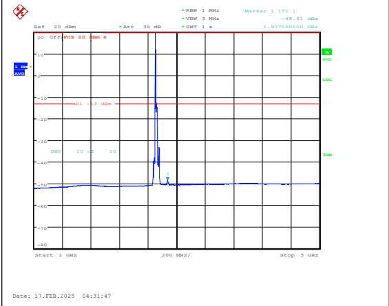
Band25-15MHz-16QAM-26115-1RB#0-1000~300 0-PASS
