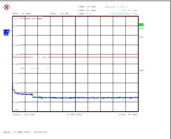
Band25-15MHz-QPSK-26365-1RB#0-0.15~30-PA SS
