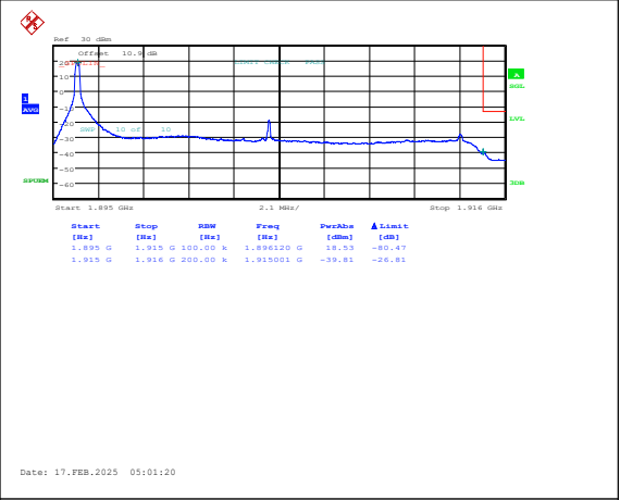
Band25-20MHz-16QAM-26590-1RB#0-PASS
