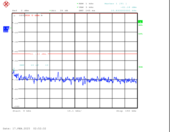
Band25-3MHz-16QAM-26675-1RB#0-0.009~0.15- PASS
