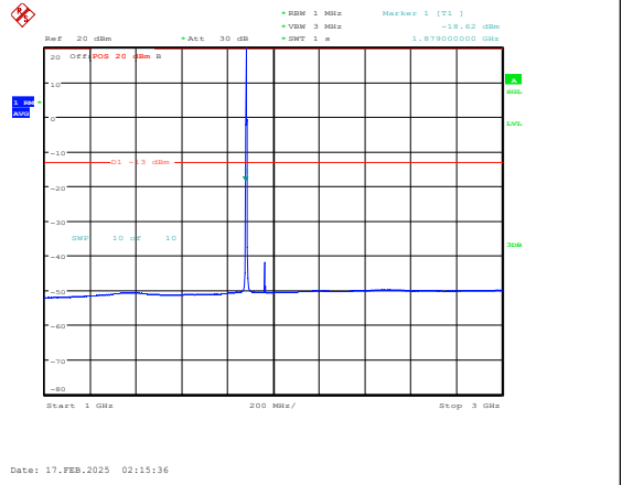
Band25-1.4MHz-QPSK-26365-1RB#0-1000~3000-P PASS
