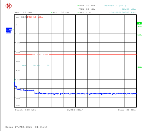
Band25-15MHz-16QAM-26115-1RB#0-0.15~30-P ASS
