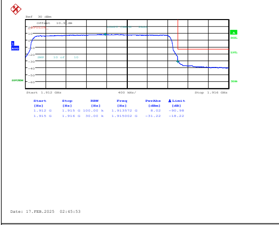
Band25-3MHz-QPSK-26675-15RB#0-PASS
