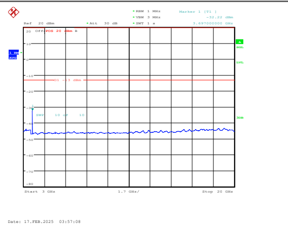
Band25-10MHz-16QAM-26090-1RB#0-3000~2000 0-PASS
