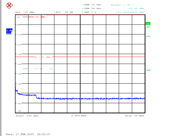
Band25-3MHz-16QAM-26675-1RB#0-0.15~30-PA SS
