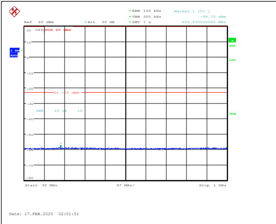
Band25-3MHz-QPSK-26675-1RB#0-30~1000-PA SS
