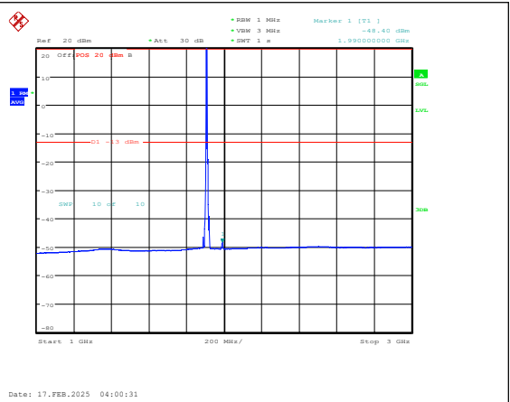
Band25-10MHz-QPSK-26640-1RB#0-1000~3000- PASS
