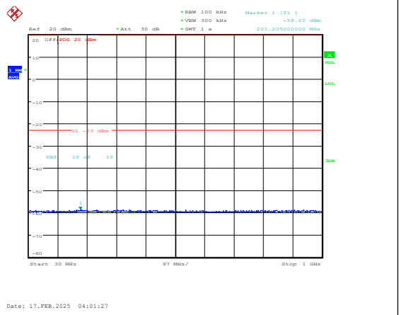
Band25-10MHz-16QAM-26640-1RB#0-30~1000-P ASS
