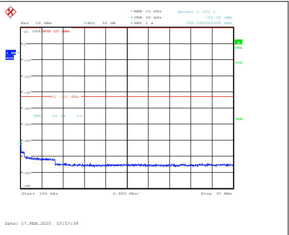
Band25-10MHz-QPSK-26365-1RB#0-0.15~30-PA SS
