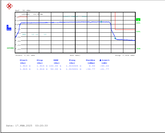
Band25-5MHz-QPSK-26665-25RB#0-PASS
