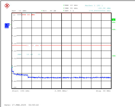
Band25-3MHz-16QAM-26365-1RB#0-0.15~30-PA SS
