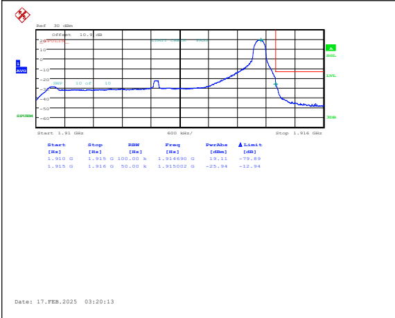
Band25-5MHz-16QAM-26665-1RB#24-PASS
