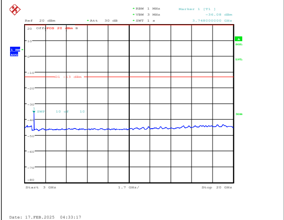
Band25-15MHz-QPSK-26365-1RB#0-3000~2000 0-PASS
