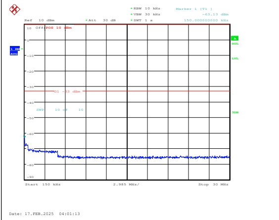
Band25-10MHz-16QAM-26640-1RB#0-0.15~30-P ASS
