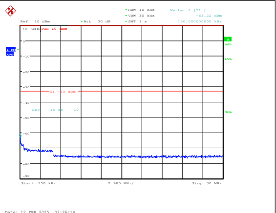
Band25-5MHz-QPSK-26665-1RB#0-0.15~30-PAS S
