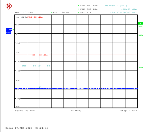
Band25-5MHz-QPSK-26365-1RB#0-30~1000-PA
