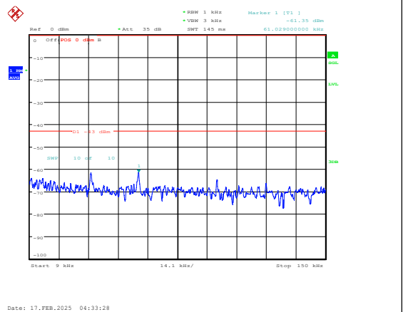
Band25-15MHz-16QAM-26365-1RB#0-0.009~0.15 -PASS
