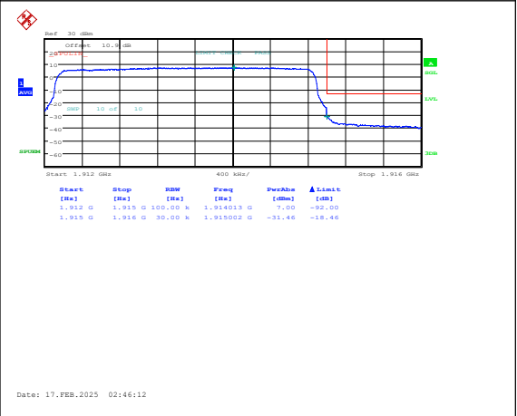
Band25-3MHz-16QAM-26675-1RB#14-PASS
