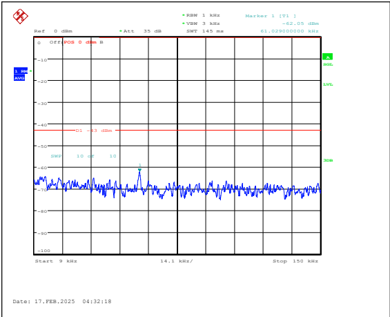
Band25-15MHz-QPSK-26365-1RB#0-0.009~0.15 -PASS
