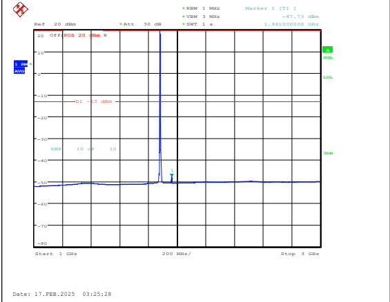
Band25-5MHz-16QAM-26365-1RB#0-1000~3000 -PASS
