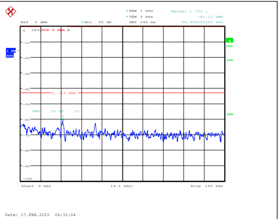
Band25-15MHz-16QAM-26115-1RB#0-0.009~0.15 -PASS
