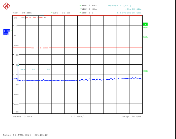
Band25-3MHz-16QAM-26055-1RB#0-3000~20000 -PASS
