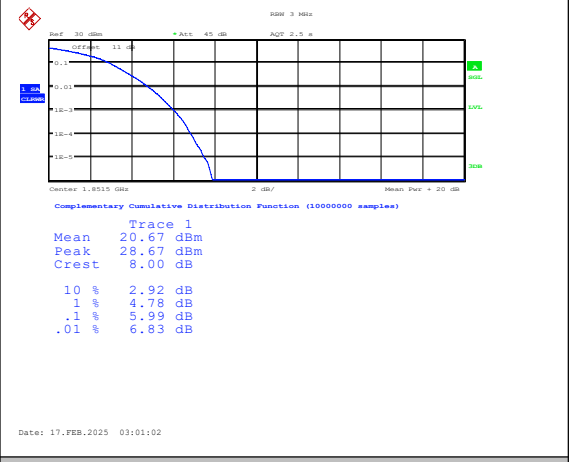
Band25-3MHz-16QAM-26055-15RB#0-PASS
