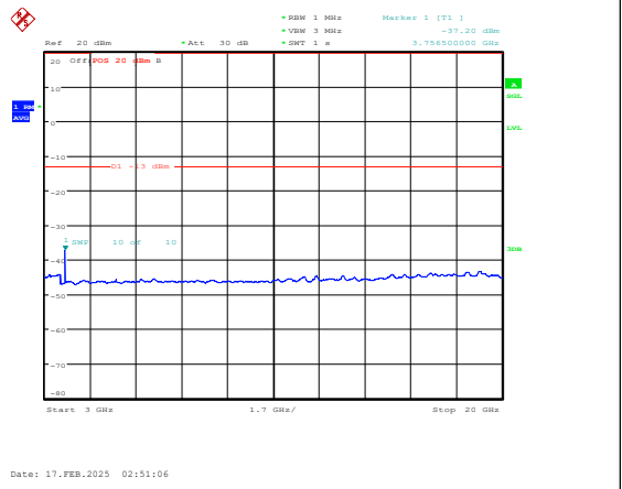
Band25-3MHz-16QAM-26365-1RB#0-3000~20000 -PASS
