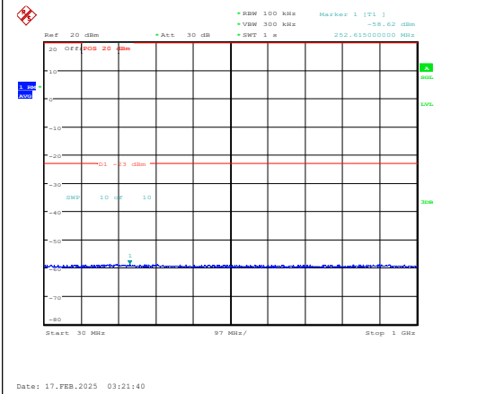
Band25-5MHz-QPSK-26065-1RB#0-30~1000-PA SS
