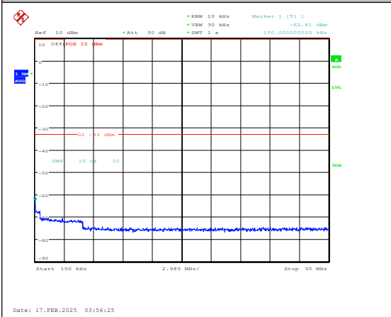
Band25-10MHz-16QAM-26090-1RB#0-0.15~30-P ASS
