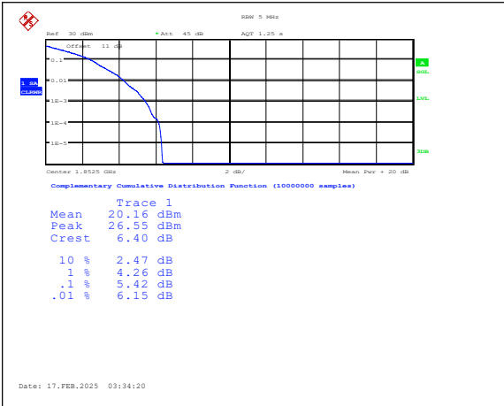
Band25-5MHz-QPSK-26065-1RB#0-PASS
