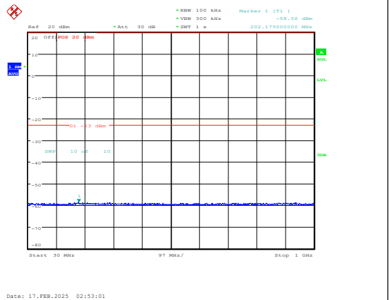
Band25-3MHz-16QAM-26675-1RB#0-30~1000-PA SS
