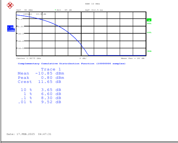
Band25-15MHz-16QAM-26615-1RB#0-PASS
