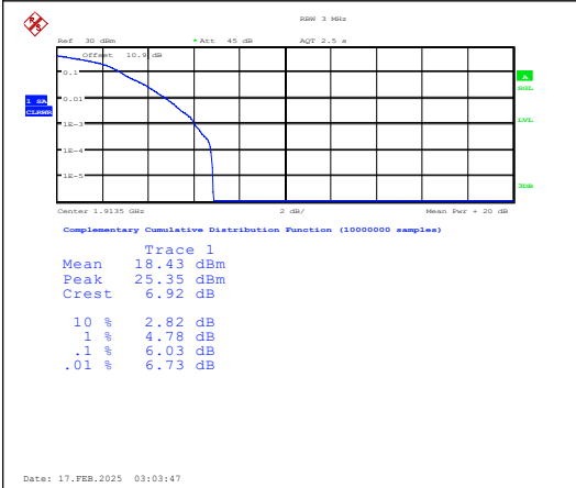
Band25-3MHz-16QAM-26675-1RB#0-PASS
