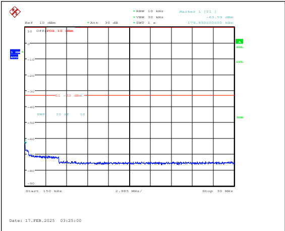
Band25-5MHz-16QAM-26365-1RB#0-0.15~30-PA SS
