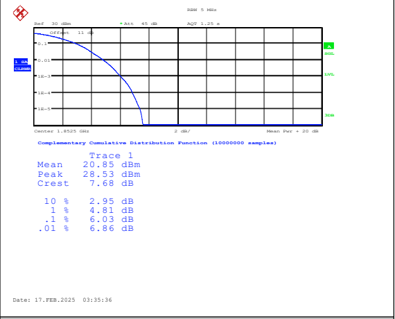
Band25-5MHz-16QAM-26065-25RB#0-PASS
