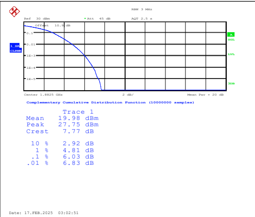
Band25-3MHz-16QAM-26365-15RB#0-PASS
