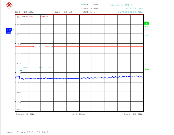
Band25-1.4MHz-QPSK-26365-1RB#0-3000~2000 0-PASS
