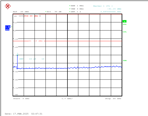
Band25-3MHz-QPSK-26055-1RB#0-3000~20000 -PASS
