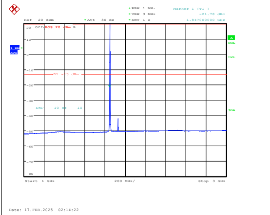
Band25-1.4MHz-16QAM-26047-1RB#0-1000~30 00-PASS
