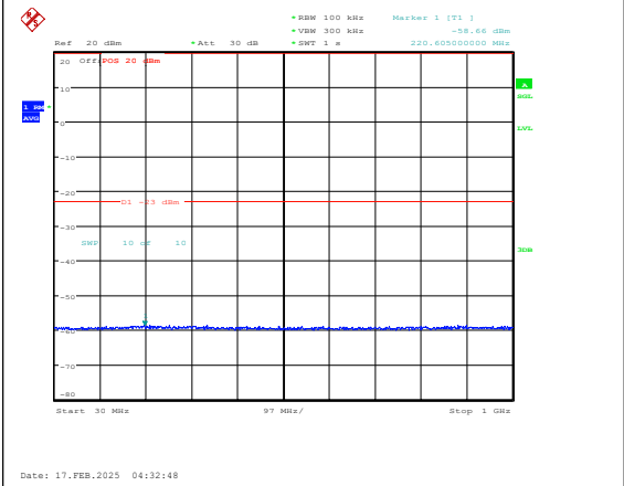
Band25-15MHz-QPSK-26365-1RB#0-30~1000-P ASS
