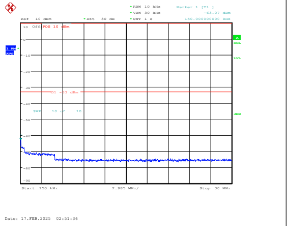
Band25-3MHz-QPSK-26675-1RB#0-0.15~30-PAS S
