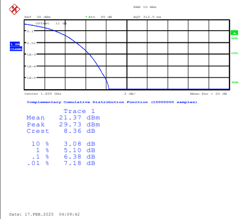
Band25-10MHz-16QAM-26090-50RB#0-PASS
