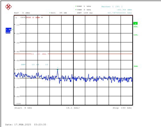
Band25-5MHz-QPSK-26365-1RB#0-0.009~0.15-PASS
