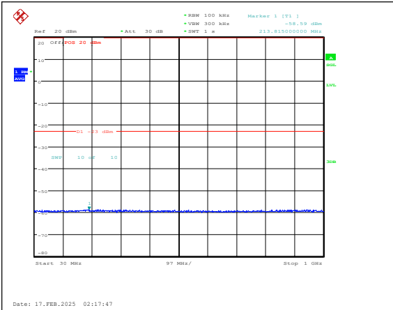
Band25-1.4MHz-QPSK-26683-1RB#0-30~1000-P ASS
