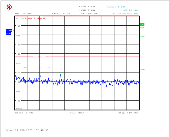
Band25-3MHz-QPSK-26365-1RB#0-0.009~0.15-PASS
