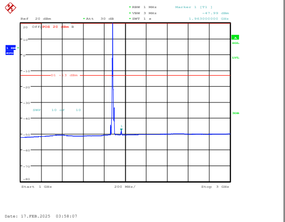
Band25-10MHz-QPSK-26365-1RB#0-1000~3000-P PASS
