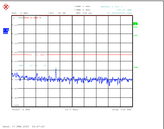
Band25-3MHz-16QAM-26055-1RB#0-0.009~0.15- PASS
