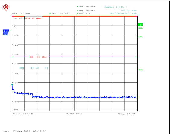
Band25-5MHz-QPSK-26365-1RB#0-0.15~30-PAS
