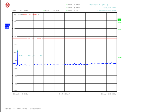
Band25-10MHz-QPSK-26640-1RB#0-3000~2000 0-PASS
