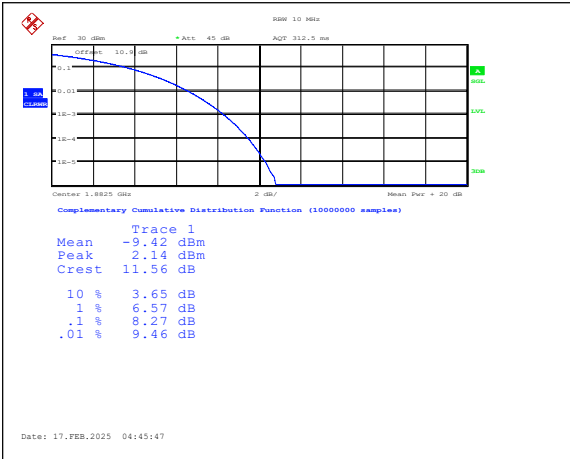
Band25-15MHz-16QAM-26365-1RB#0-PASS
