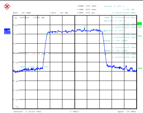
Band25-5MHz-16QAM-26365-25RB#0-PASS
