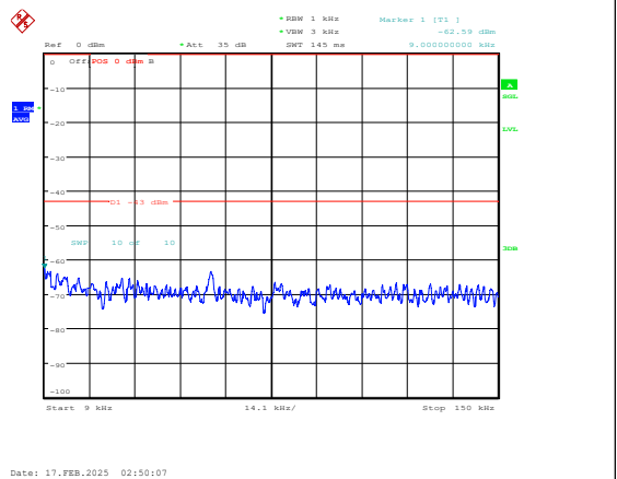
Band25-3MHz-16QAM-26365-1RB#0-0.009~0.15-PASS
