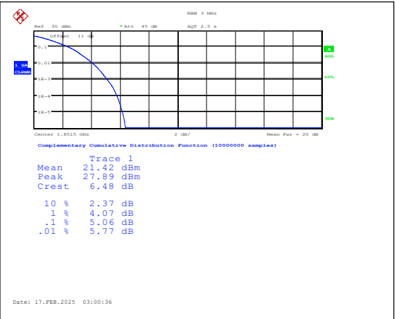
Band25-3MHz-QPSK-26055-15RB#0-PASS
