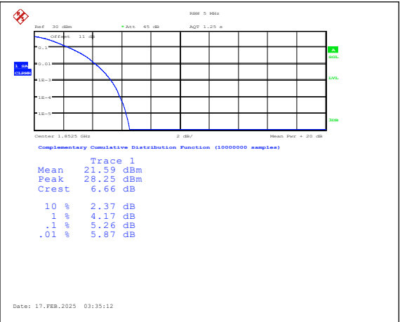
Band25-5MHz-QPSK-26065-25RB#0-PASS
