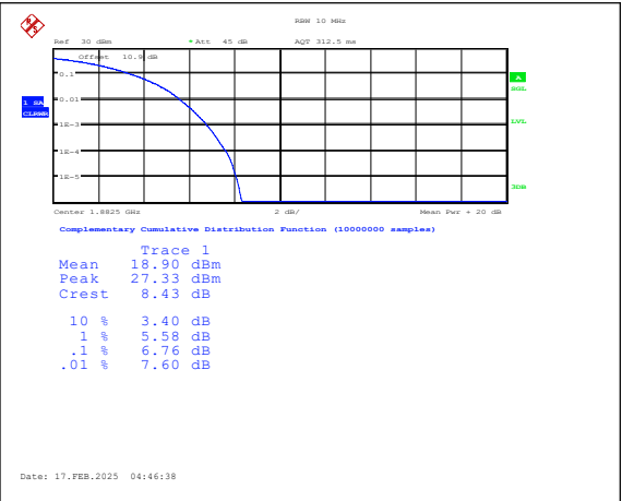
Band25-15MHz-16QAM-26365-75RB#0-PASS
