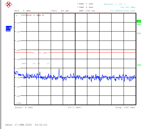
Band25-3MHz-QPSK-26675-1RB#0-0.009~0.15- PASS
