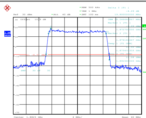
Band25-20MHz-16QAM-26140-100RB#0-PASS
