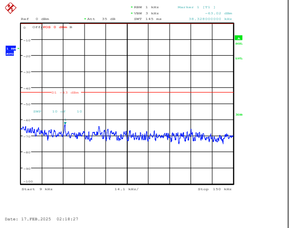
Band25-1.4MHz-16QAM-26683-1RB#0-0.009~0.1 5-PASS
