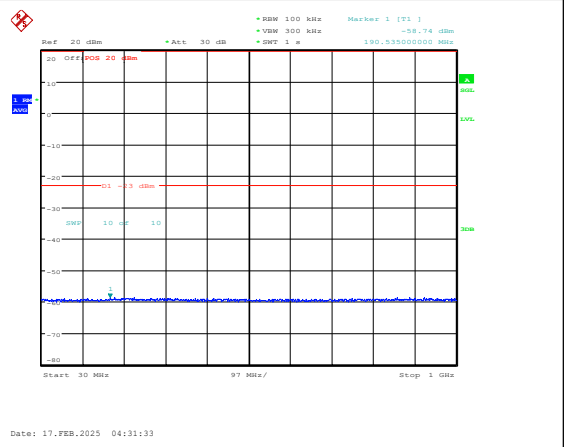
Band25-15MHz-16QAM-26115-1RB#0-30~1000-P ASS
