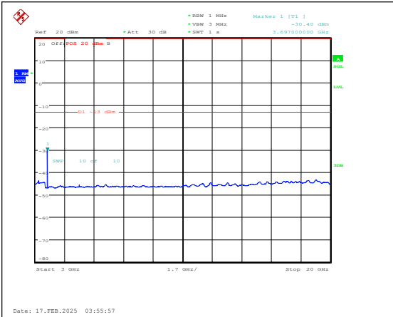
Band25-10MHz-QPSK-26090-1RB#0-3000~2000 0-PASS
