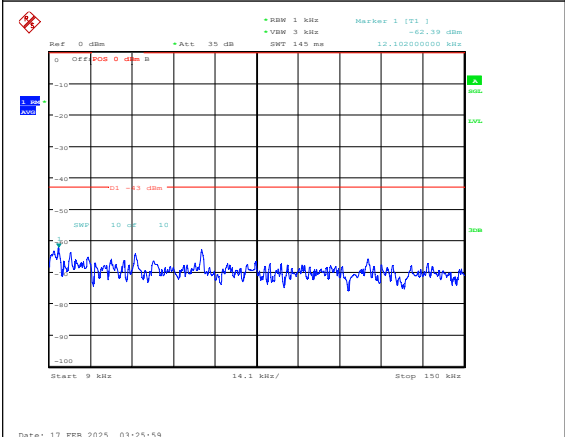
Band25-5MHz-QPSK-26665-1RB#0-0.009~0.15- PASS
