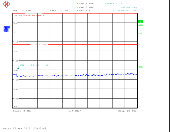
Band25-5MHz-16QAM-26365-1RB#0-3000~20000 -PASS
