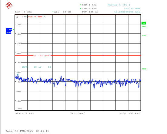
Band25-5MHz-QPSK-26065-1RB#0-0.009~0.15- PASS
