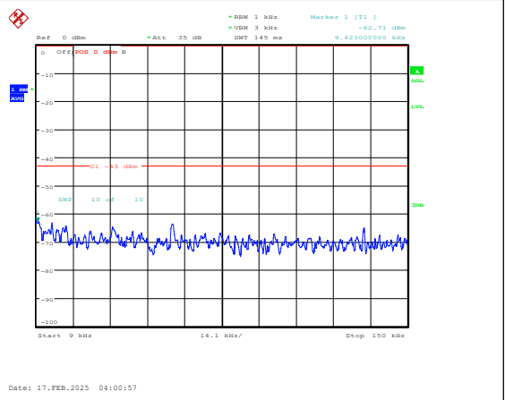
Band25-10MHz-16QAM-26640-1RB#0-0.009~0.15 -PASS
