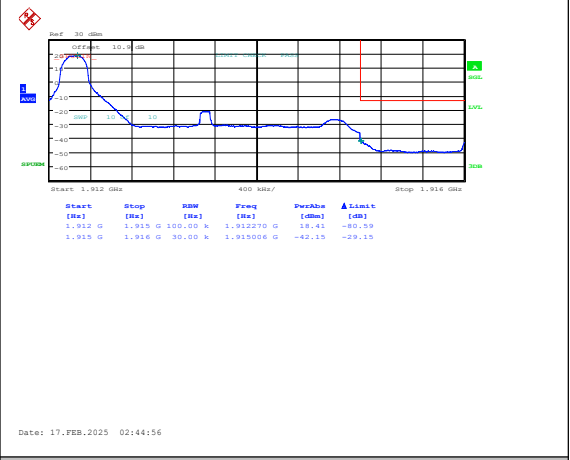
Band25-3MHz-QPSK-26675-1RB#14-PASS
