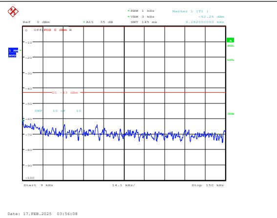
Band25-10MHz-16QAM-26090-1RB#0-0.009~0.15 -PASS
