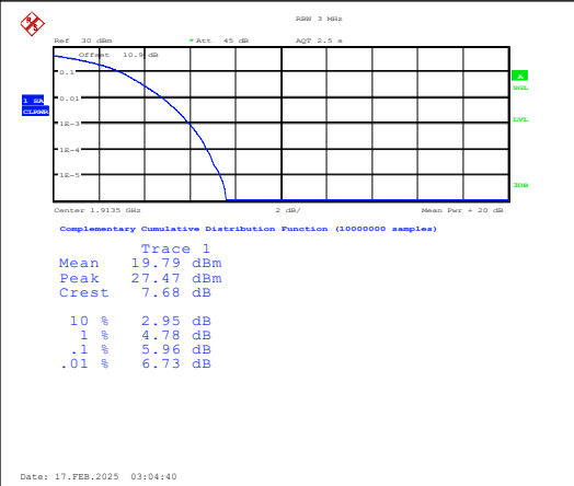
Band25-3MHz-16QAM-26675-15RB#0-PASS
