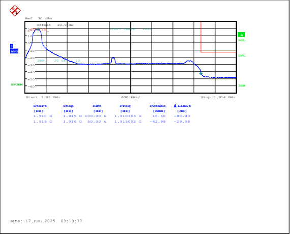
Band25-5MHz-16QAM-26665-1RB#0-PASS
