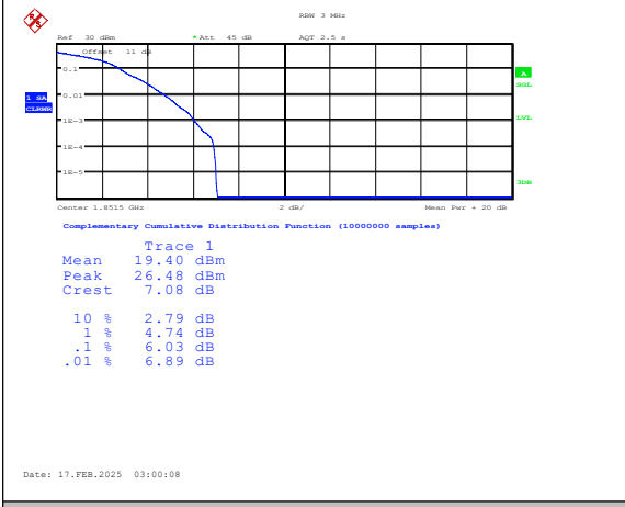
Band25-3MHz-16QAM-26055-1RB#0-PASS
