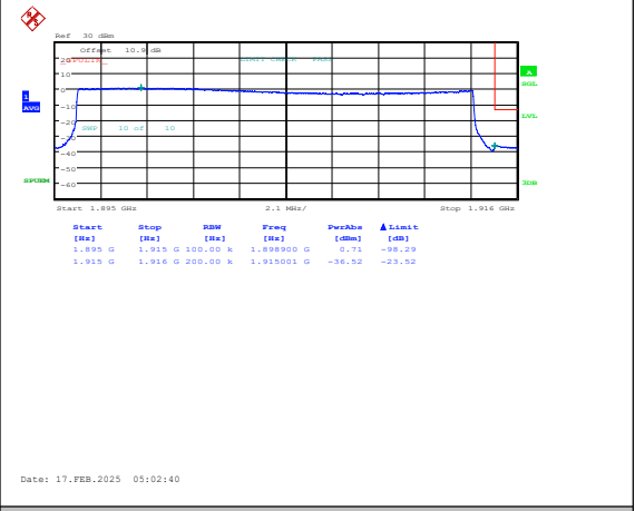
Band25-20MHz-16QAM-26590-100RB#0-PASS
