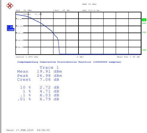
Band25-10MHz-16QAM-26090-1RB#0-PASS
