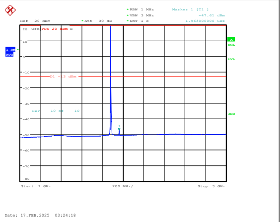
Band25-5MHz-QPSK-26365-1RB#0-1000~3000-P
