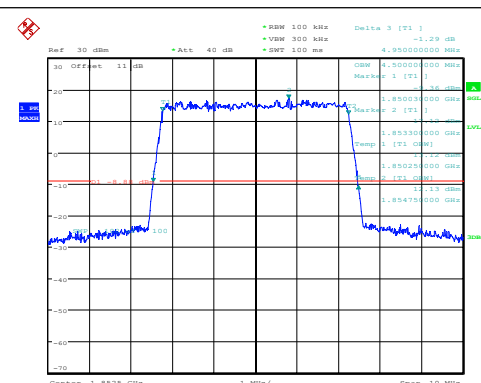
Band25-5MHz-QPSK-26065-25RB#0-PASS
