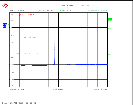
Band25-1.4MHz-QPSK-26683-1RB#0-1000~3000- PASS
