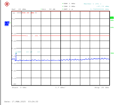
Band25-5MHz-QPSK-26365-1RB#0-3000~20000-PA
