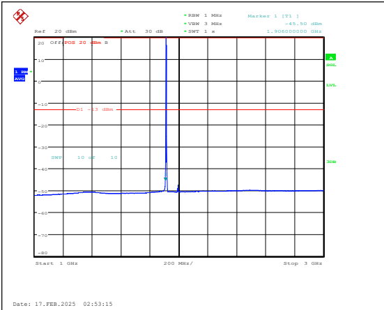
Band25-3MHz-16QAM-26675-1RB#0-1000~3000 -PASS
