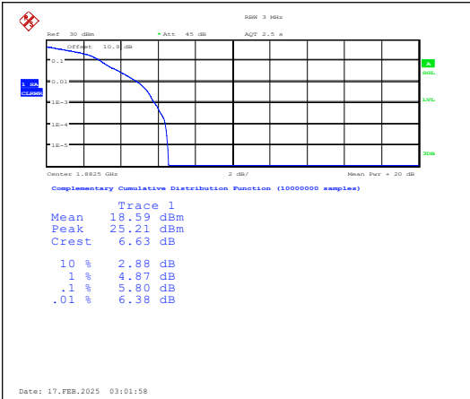
Band25-3MHz-16QAM-26365-1RB#0-PASS
