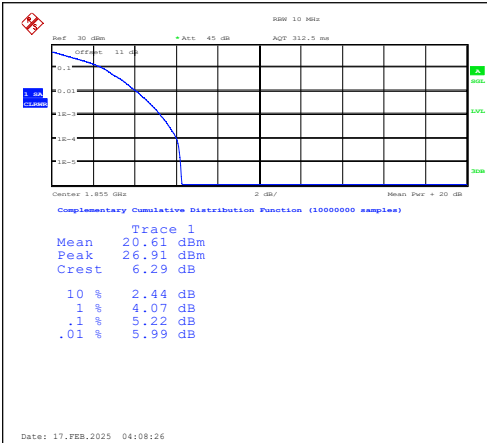
Band25-10MHz-QPSK-26090-1RB#0-PASS
