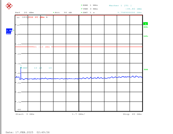
Band25-3MHz-QPSK-26365-1RB#0-3000~20000-PA
