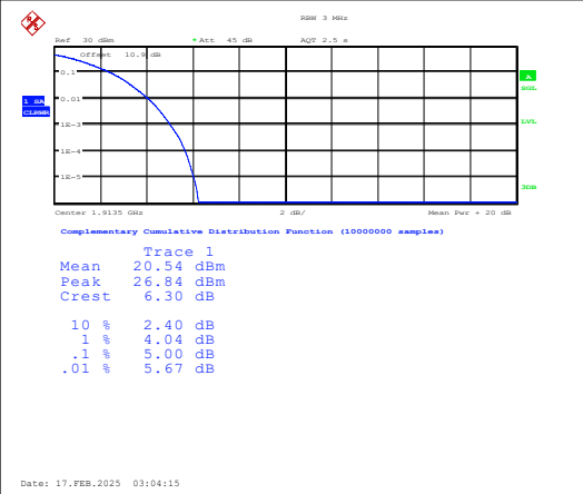
Band25-3MHz-QPSK-26675-15RB#0-PASS
