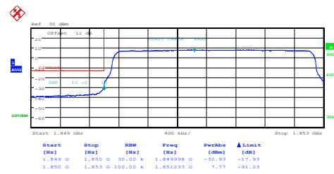
Band25-3MHz-16QAM-26055-1RB#0-PASS
