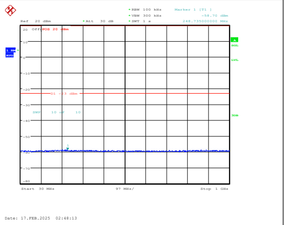
Band25-3MHz-16QAM-26055-1RB#0-30~1000-PA SS
