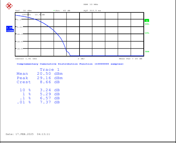
Band25-10MHz-16QAM-26640-50RB#0-PASS
