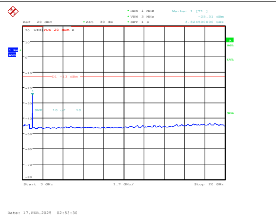
Band25-3MHz-16QAM-26675-1RB#0-3000~20000 -PASS
