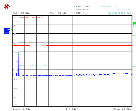
Band25-1.4MHz-16QAM-26683-1RB#0-3000~200 00-PASS
