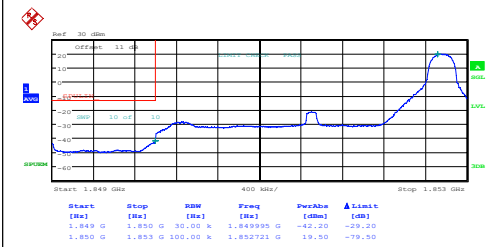
Band25-3MHz-QPSK-26055-15RB#0-PASS
