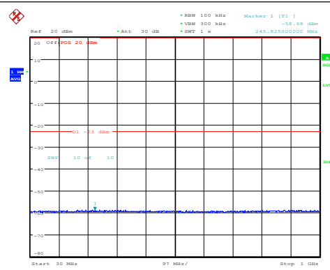
Band25-1.4MHz-16QAM-26365-1RB#0-30~1000-PASS
