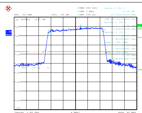
Band25-20MHz-QPSK-26140-100RB#0-PASS
