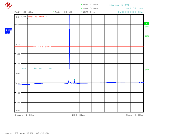
Band25-5MHz-QPSK-26065-1RB#0-1000~3000-P ASS
