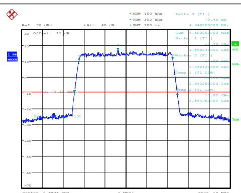
Band25-5MHz-16QAM-26065-25RB#0-PASS
