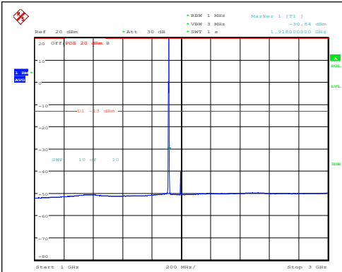
Band25-1.4MHz-16QAM-26683-1RB#0-1000~30 00-PASS
