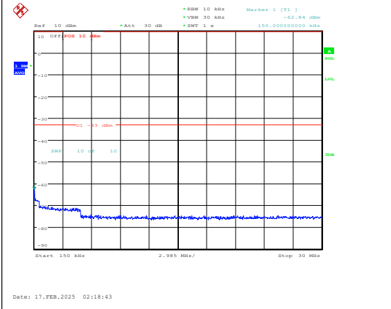
Band25-1.4MHz-16QAM-26683-1RB#0-0.15~30- PASS
