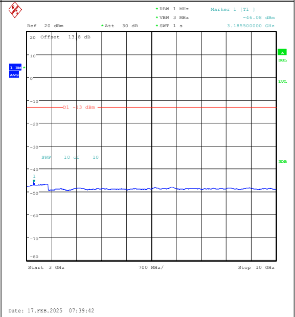
Band26(824-849)-1.4MHz-16QAM-26915-1RB#0-3000~10000-PASS
