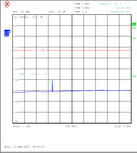
Band26(824-849)-5MHz-16QAM-26915-1RB#0-1 000~3000-PASS
