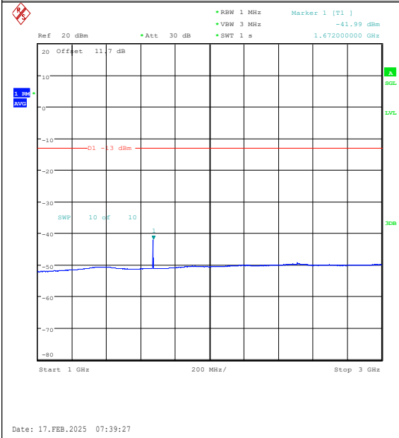
Band26(824-849)-1.4MHz-16QAM-26915-1RB#0-1000~3000-PASS
