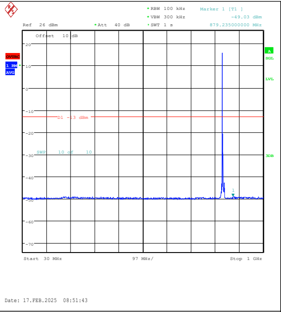
Band26(824-849)-5MHz-16QAM-26915-1RB#0-30 ~1000-PASS
