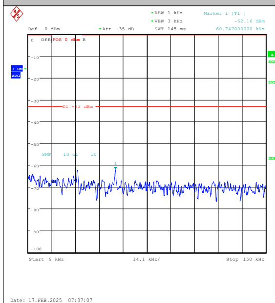
Band26(824-849)-1.4MHz-QPSK-26915-1RB#0-0 .009~0.15-PASS
