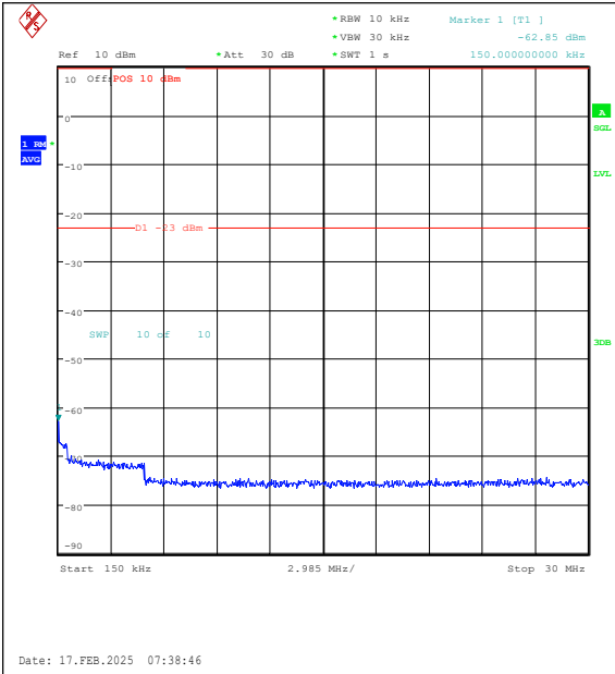
Band26(824-849)-1.4MHz-16QAM-26915-1RB#0-0.15~30-PASS
