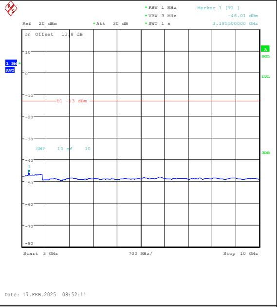
Band26(824-849)-5MHz-16QAM-26915-1RB#0-30 00~10000-PASS
