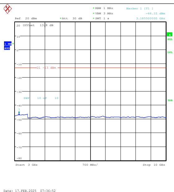
Band26(824-849)-1.4MHz-16QAM-26797-1RB#0- 3000~10000-PASS
