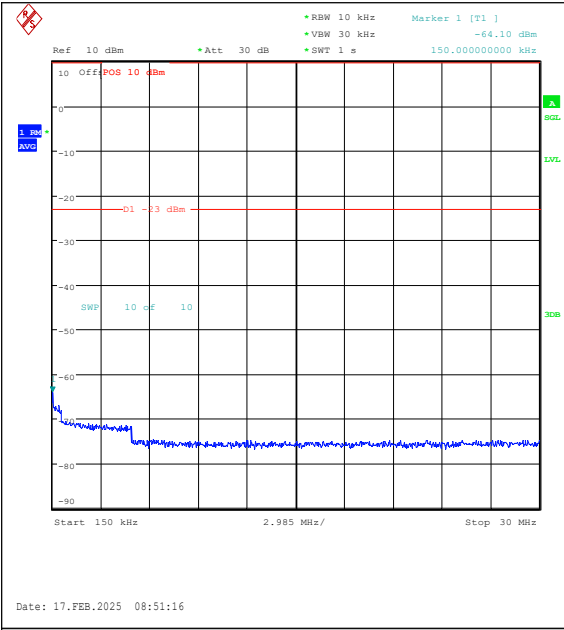
Band26(824-849)-5MHz-16QAM-26915-1RB#0-0. 15~30-PASS
