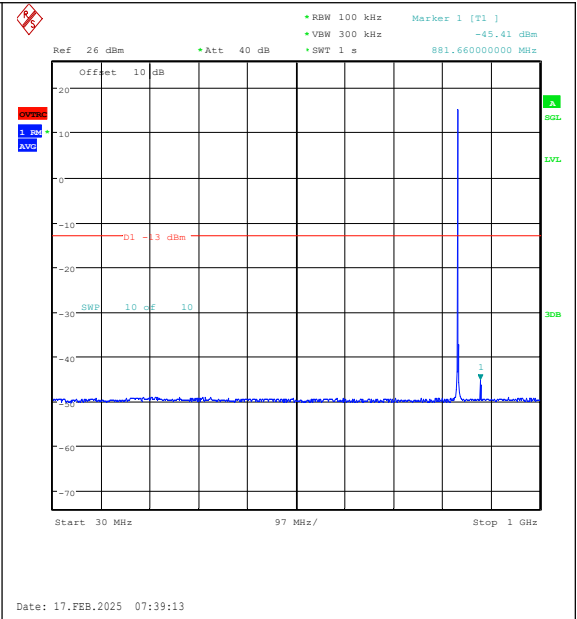
Band26(824-849)-1.4MHz-16QAM-26915-1RB#0-30~1000-PASS
