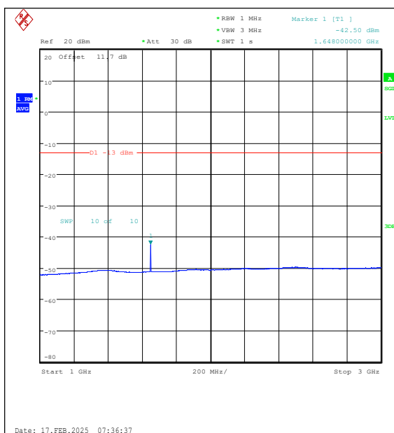
Band26(824-849)-1.4MHz-16QAM-26797-1RB#0- 1000~3000-PASS
