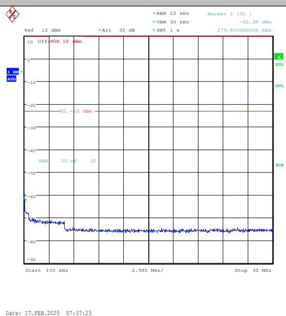
Band26(824-849)-1.4MHz-QPSK-26915-1RB#0-0. 15~30-PASS
