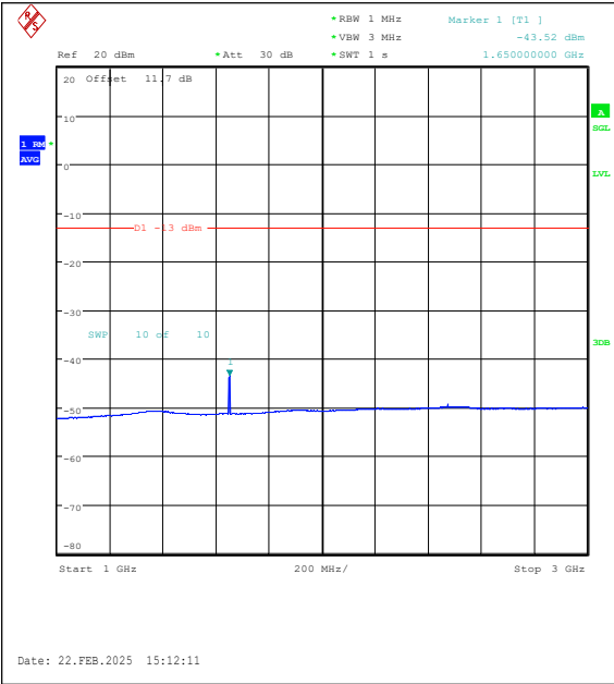
Band26(824-849)-15MHz-16QAM-26865-1RB#0-1000~3000-PASS
