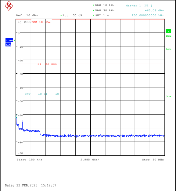
Band26(824-849)-15MHz-QPSK-26915-1RB#0-0.15~30-PASS
