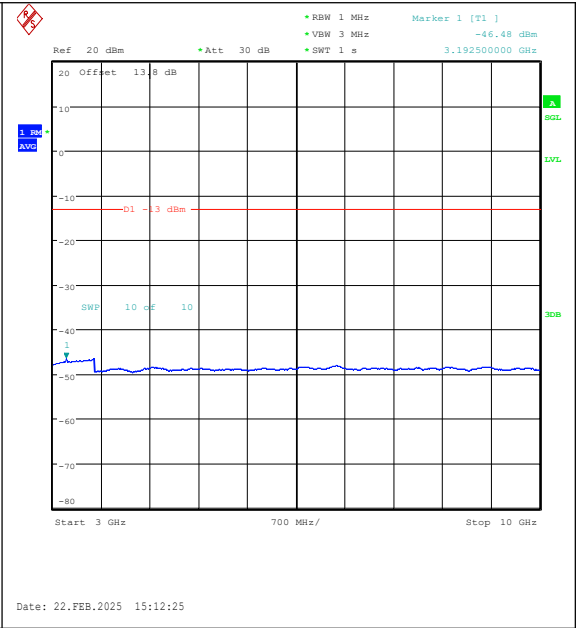
Band26(824-849)-15MHz-16QAM-26865-1RB#0-3000~10000-PASS
