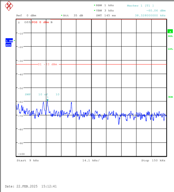
Band26(824-849)-15MHz-QPSK-26915-1RB#0-0.009~0.15-PASS
