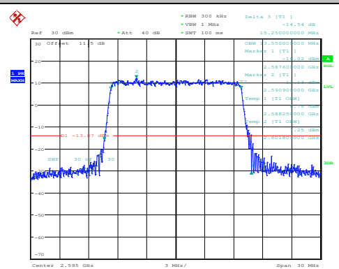
Band38-15MHz-16QAM-37825-75RB#0-PASS
