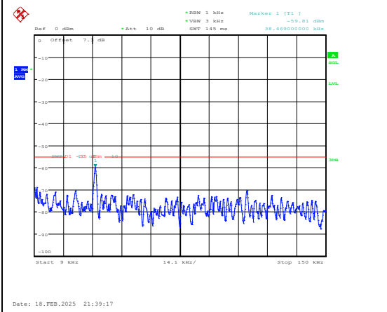
Band38-5MHz-QPSK-38225-1RB#0-0.009~0.15-PASS
