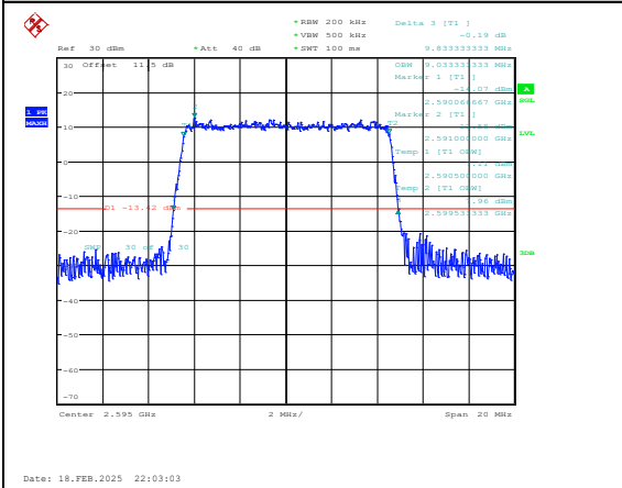
Band38-10MHz-QPSK-38000-50RB#0-PASS
