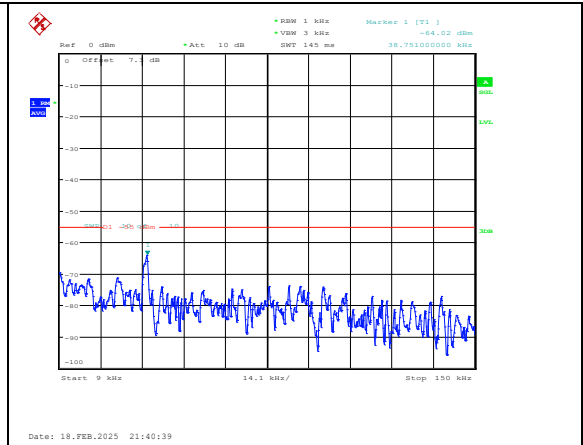
Band38-5MHz-16QAM-38225-1RB#0-0.009~0.15- PASS
