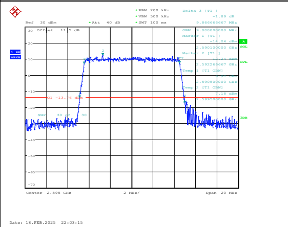
Band38-10MHz-16QAM-38000-50RB#0-PASS
