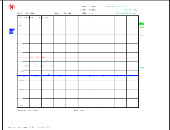
Band38-5MHz-16QAM-38225-1RB#0-20000~2700 0-PASS
