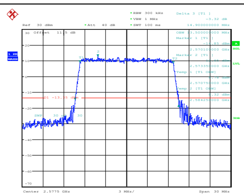
Band38-15MHz-16QAM-37825-75RB#0-PASS
