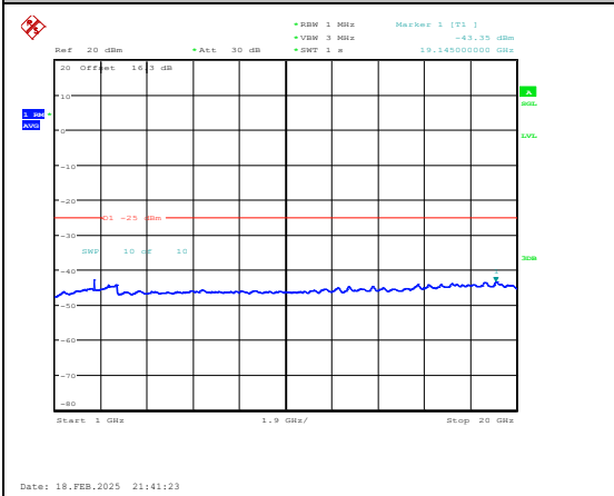
Band38-5MHz-16QAM-38225-1RB#0-1000~2000 0-PASS
