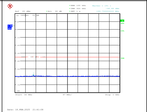
Band38-5MHz-16QAM-38225-1RB#0-30~1000-PA SS
