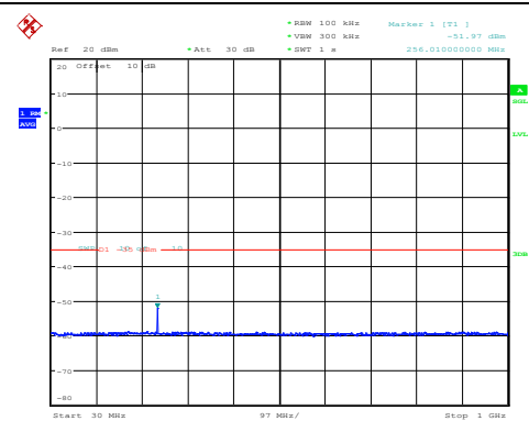
Band38-5MHz-16QAM-37775-1RB#0-30~1000-PA SS
