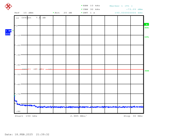
Band38-5MHz-QPSK-38225-1RB#0-0.15~30-PAS
