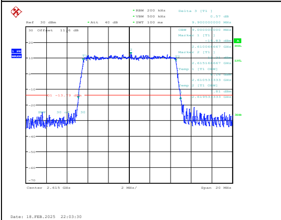
Band38-10MHz-QPSK-38200-50RB#0-PASS
