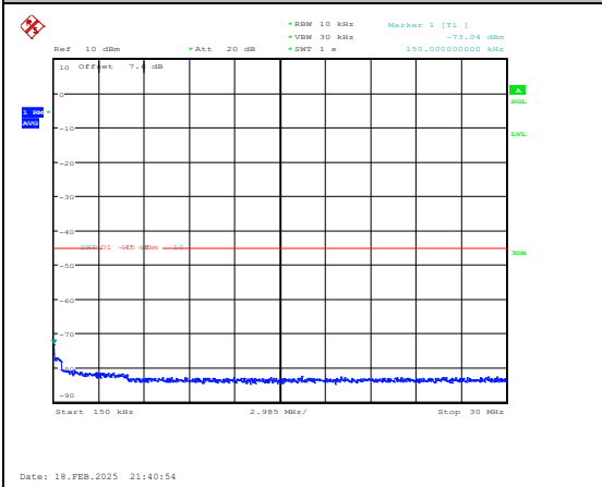
Band38-5MHz-16QAM-38225-1RB#0-0.15~30-PA SS
