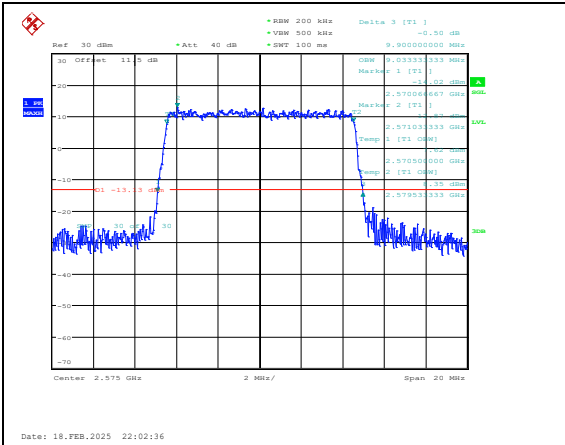
Band38-10MHz-QPSK-37800-50RB#0-PASS
