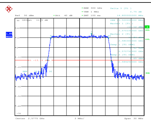
Band38-15MHz-QPSK-37825-75RB#0-PASS
