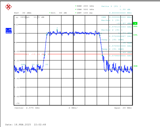
Band38-10MHz-16QAM-37800-50RB#0-PASS
