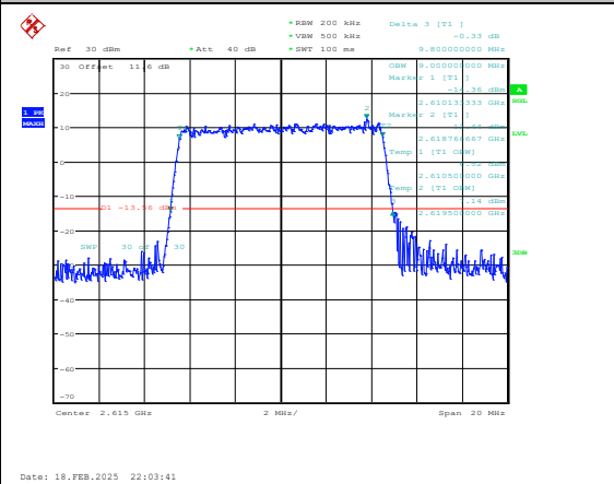
Band38-10MHz-16QAM-38200-50RB#0-PASS
