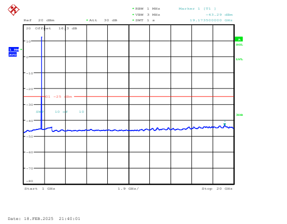
Band38-5MHz-QPSK-38225-1RB#0-1000~20000-PASS
