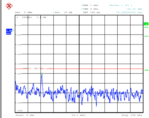
Band38-5MHz-16QAM-37775-1RB#0-1000~2000 0-PASS
