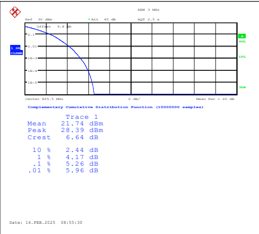
Band5-3MHz-QPSK-20415-15RB#0-PASS
