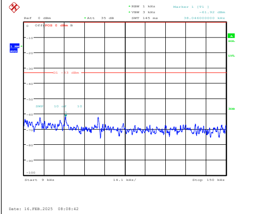
Band5-1.4MHz-QPSK-20525-1RB#0-0.009~0.15- PASS
