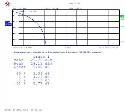
Band5-5MHz-QPSK-20525-25RB#0-PASS
