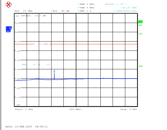
Band5-1.4MHz-16QAM-20407-1RB#0-1000~300 0-PASS
