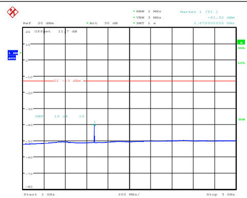
Band5-1.4MHz-QPSK-20525-1RB#0-1000~3000-P ASS
