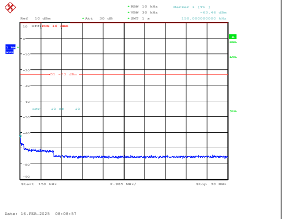
Band5-1.4MHz-QPSK-20525-1RB#0-0.15~30-PAS S
