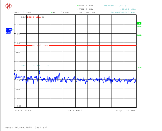
Band5-1.4MHz-QPSK-20643-1RB#0-0.009~0.15- PASS
