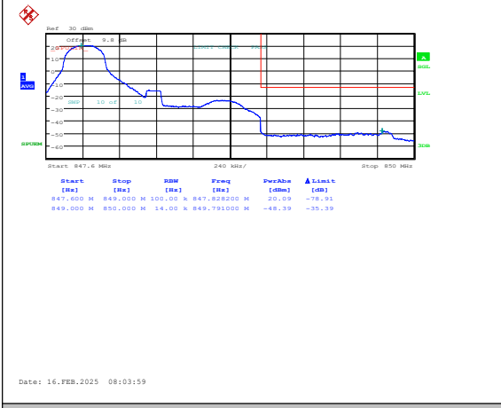
Band5-1.4MHz-QPSK-20643-1RB#0-PASS
