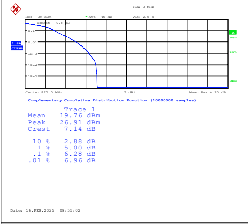
Band5-3MHz-16QAM-20415-1RB#0-PASS
