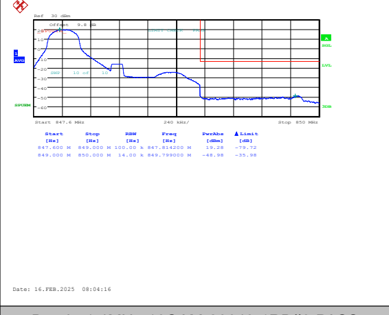
Band5-1.4MHz-16QAM-20643-1RB#0-PASS
