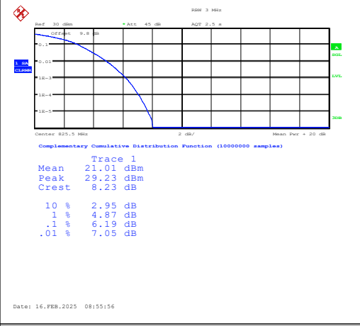
Band5-3MHz-16QAM-20415-15RB#0-PASS
