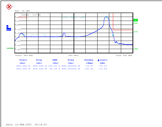
Band5-5MHz-16QAM-20625-1RB#24-PASS
