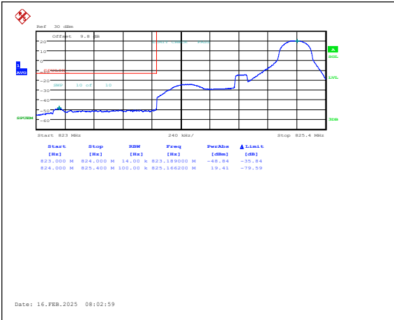
Band5-1.4MHz-16QAM-20407-1RB#5-PASS
