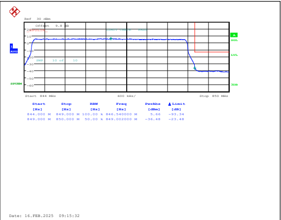
Band5-5MHz-16QAM-20625-25RB#0-PASS
