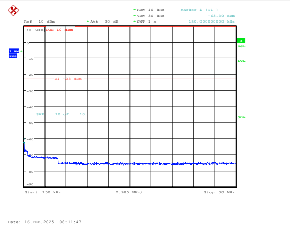
Band5-1.4MHz-QPSK-20643-1RB#0-0.15~30-PAS S
