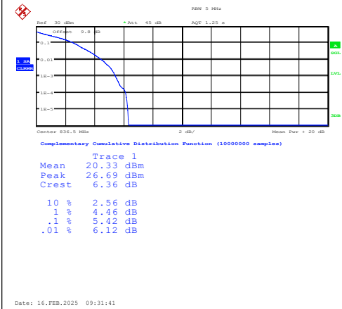
Band5-5MHz-QPSK-20525-1RB#0-PASS
