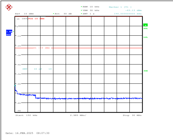
Band5-1.4MHz-16QAM-20407-1RB#0-0.15~30-P ASS
