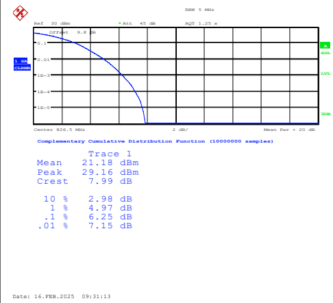
Band5-5MHz-16QAM-20425-25RB#0-PASS
