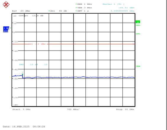
Band5-1.4MHz-16QAM-20407-1RB#0-3000~1000 0-PASS
