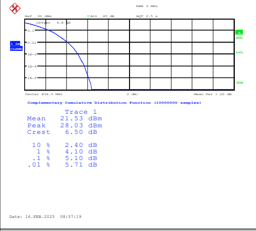
Band5-3MHz-QPSK-20525-15RB#0-PASS
