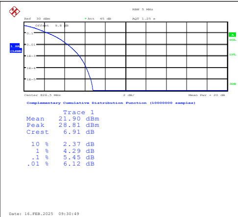
Band5-5MHz-QPSK-20425-25RB#0-PASS
