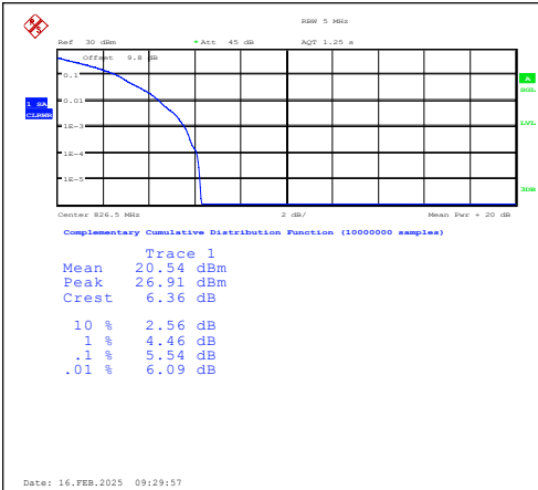
Band5-5MHz-QPSK-20425-1RB#0-PASS
