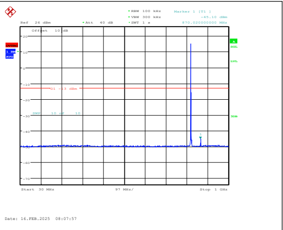
Band5-1.4MHz-16QAM-20407-1RB#0-30~1000-P ASS
