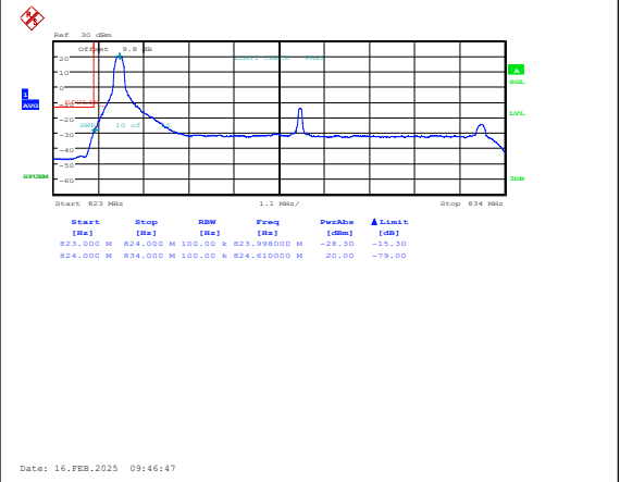
Band5-10MHz-16QAM-20450-1RB#0-PASS
