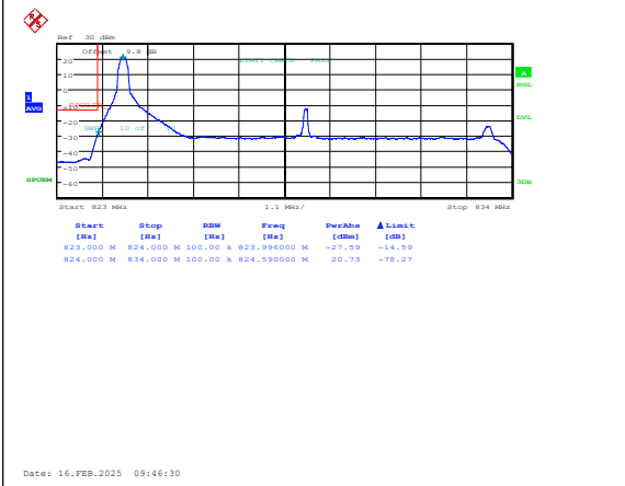
Band5-10MHz-QPSK-20450-1RB#0-PASS
