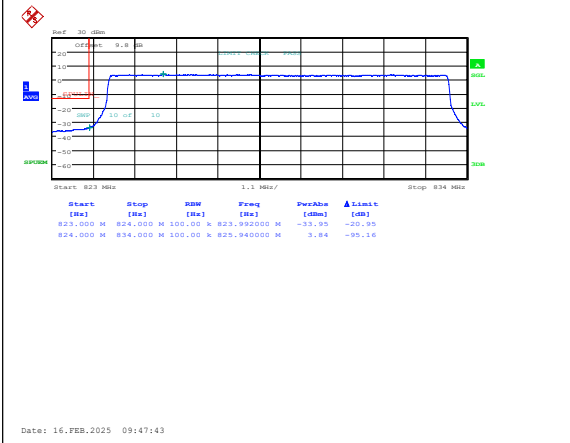
Band5-10MHz-QPSK-20450-50RB#0-PASS
