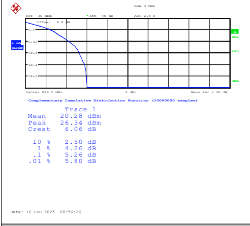
Band5-3MHz-QPSK-20525-1RB#0-PASS
