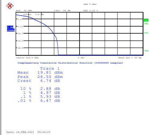
Band5-5MHz-16QAM-20425-1RB#0-PASS
