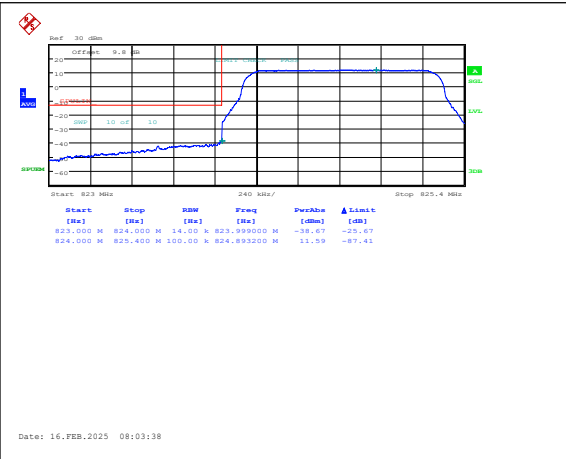
Band5-1.4MHz-16QAM-20407-6RB#0-PASS
