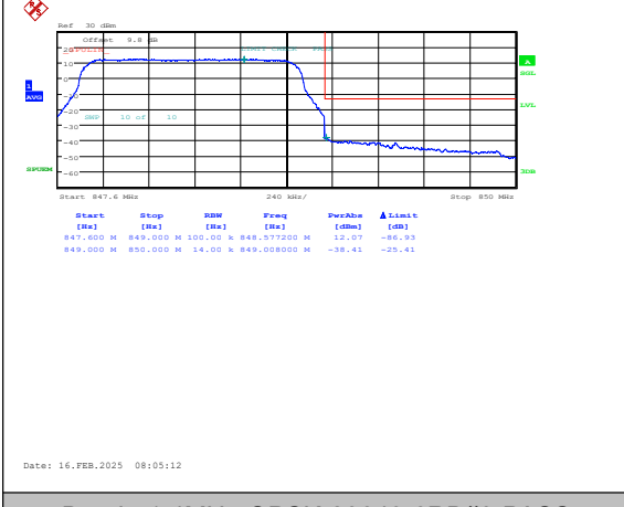
Band5-1.4MHz-QPSK-20643-6RB#0-PASS
