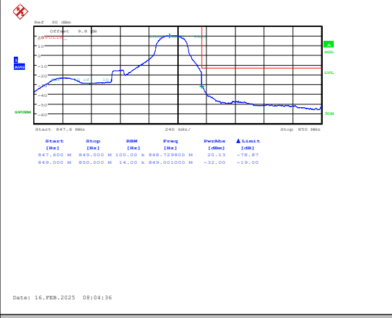
Band5-1.4MHz-QPSK-20643-1RB#5-PASS
