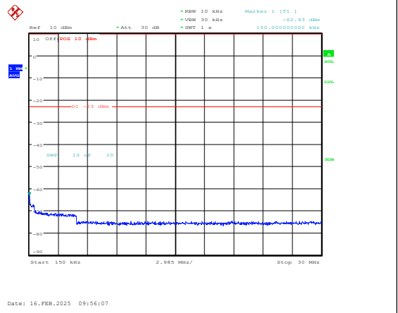
Band5-10MHz-QPSK-20600-1RB#0-0.15~30-PAS S
