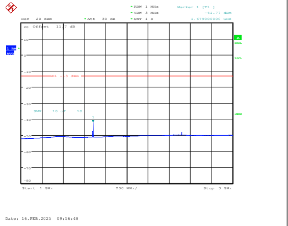
Band5-10MHz-QPSK-20600-1RB#0-1000~3000-P ASS
