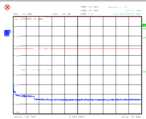
Band5-10MHz-QPSK-20450-1RB#0-0.15~30-PAS
