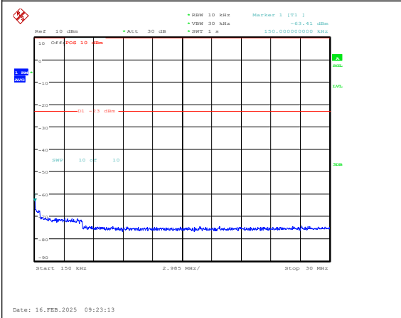
Band5-5MHz-16QAM-20625-1RB#0-0.15~30-PA SS
