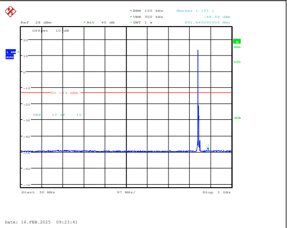
Band5-5MHz-16QAM-20625-1RB#0-30~1000-PAS S
