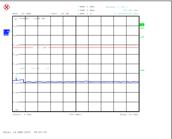
Band5-3MHz-16QAM-20525-1RB#0-3000~10000-PASS
