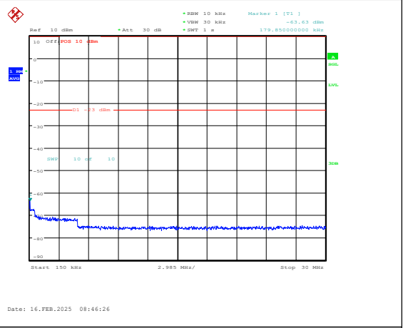
Band5-3MHz-QPSK-20635-1RB#0-0.15~30-PASS
