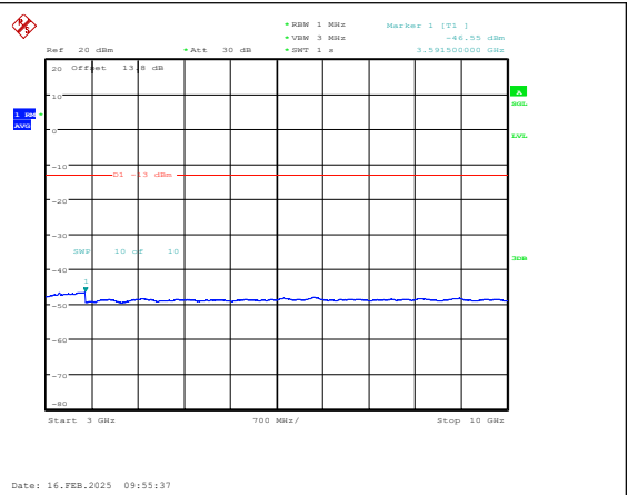
Band5-10MHz-16QAM-20525-1RB#0-3000~10000 -PASS
