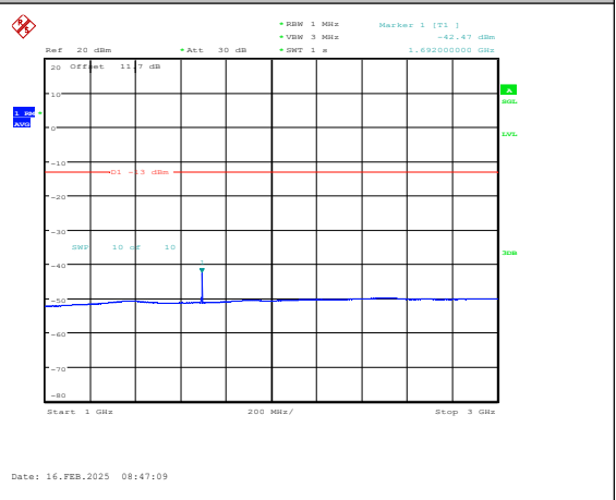
Band5-3MHz-QPSK-20635-1RB#0-1000~3000-PASS
