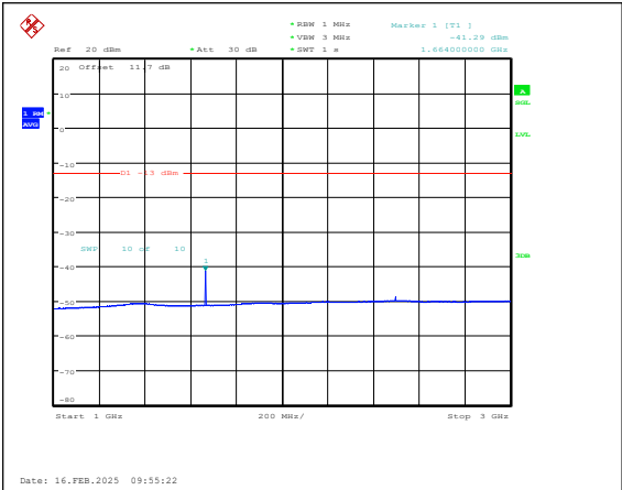
Band5-10MHz-16QAM-20525-1RB#0-1000~3000 -PASS
