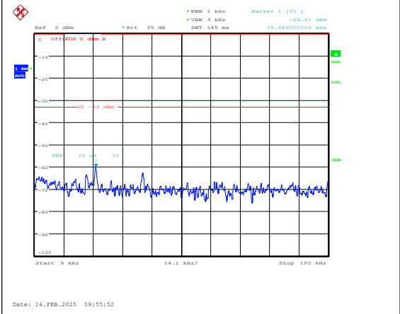
Band5-10MHz-QPSK-20600-1RB#0-0.009~0.15- PASS
