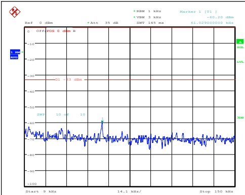
Band5-10MHz-QPSK-20450-1RB#0-0.009~0.15-PASS
