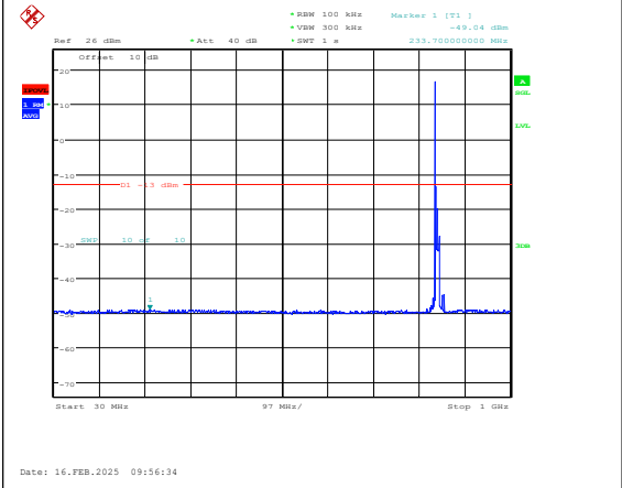
Band5-10MHz-QPSK-20600-1RB#0-30~1000-PA SS
