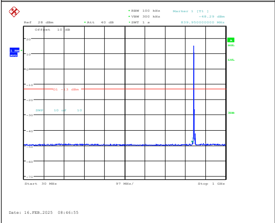
Band5-3MHz-QPSK-20635-1RB#0-30~1000-PASS
