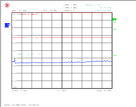
Band66-10MHz-QPSK-132322-1RB#0-3000~20000-PASS
