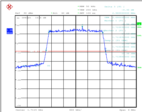
Band66-3MHz-QPSK-131987-15RB#0-PASS
