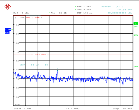
Band66-15MHz-16QAM-132047-1RB#0-0.009~0.1 5-PASS
