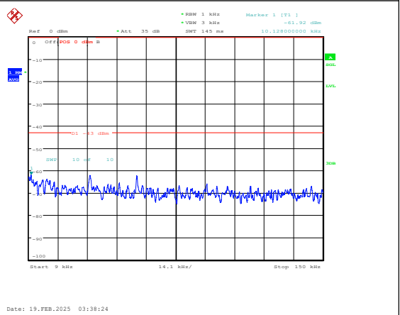
Band66-10MHz-16QAM-132322-1RB#0-0.009~0.1 5-PASS
