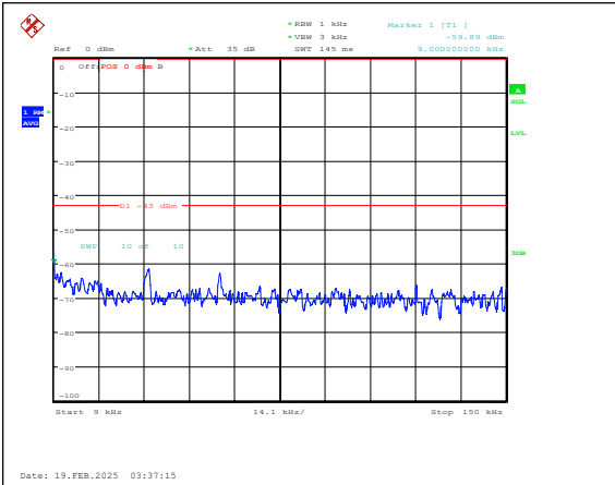
Band66-10MHz-QPSK-132322-1RB#0-0.009~0.1 5-PASS
