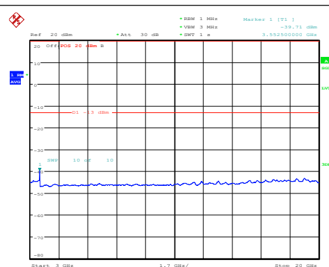
Band66-3MHz-16QAM-132657-1RB#0-3000~2000 0-PASS
