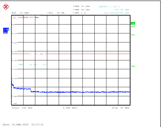
Band66-10MHz-QPSK-132322-1RB#0-0.15~30-PA SS
