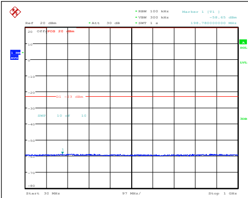
Band66-1.4MHz-QPSK-132665-1RB#0-30~1000-PASS
