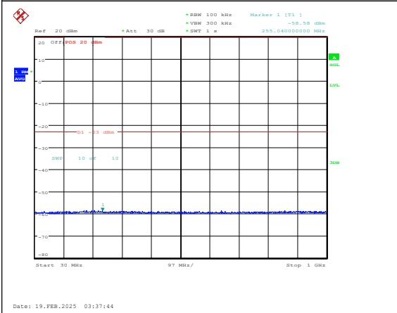
Band66-10MHz-QPSK-132322-1RB#0-30~1000-PASS
