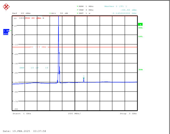
Band66-10MHz-QPSK-132322-1RB#0-1000~3000-PASS
