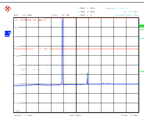
Band66-3MHz-16QAM-132657-1RB#0-1000~300 0-PASS
