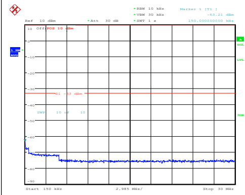
Band66-1.4MHz-QPSK-132665-1RB#0-3000~200-00-PASS
