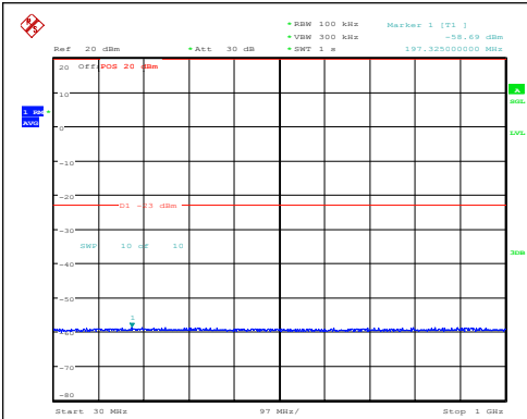
Band66-10MHz-QPSK-132622-1RB#0-30~1000-PASS
