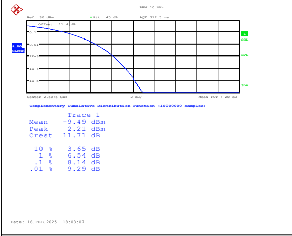
Band7-15MHz-16QAM-20825-1RB#0-PASS
