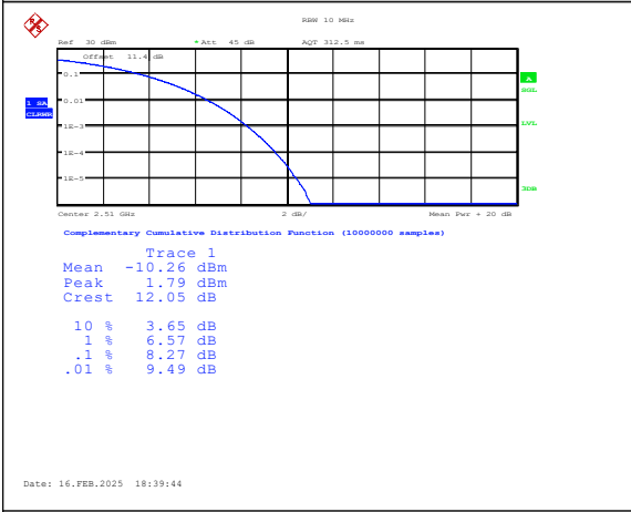
Band7-20MHz-16QAM-20850-1RB#0-PASS
