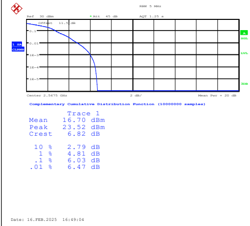
Band7-5MHz-16QAM-21425-1RB#0-PASS
