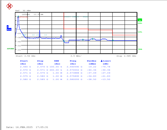
Band7-10MHz-QPSK-21400-1RB#0-PASS
