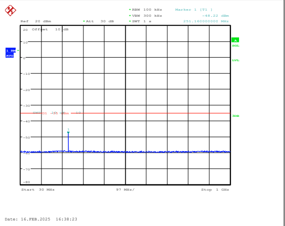
Band7-5MHz-16QAM-21425-1RB#0-30~1000-PAS S
