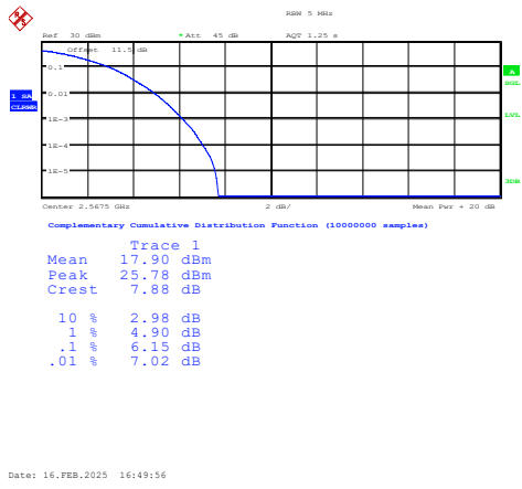
Band7-5MHz-16QAM-21425-25RB#0-PASS
