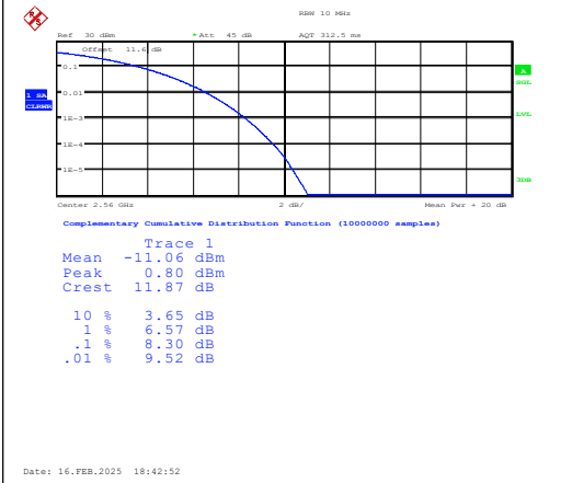
Band7-20MHz-16QAM-21350-1RB#0-PASS
