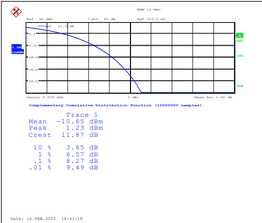
Band7-20MHz-16QAM-21100-1RB#0-PASS
