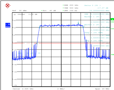
Band7-10MHz-QPSK-20800-50RB#0-PASS
