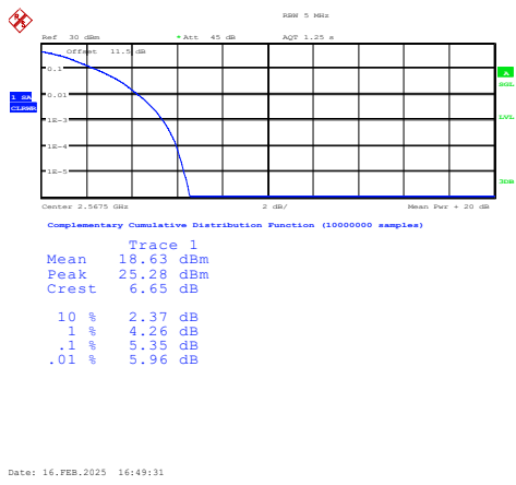
Band7-5MHz-QPSK-21425-25RB#0-PASS
