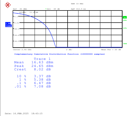
Band7-20MHz-QPSK-21350-100RB#0-PASS
