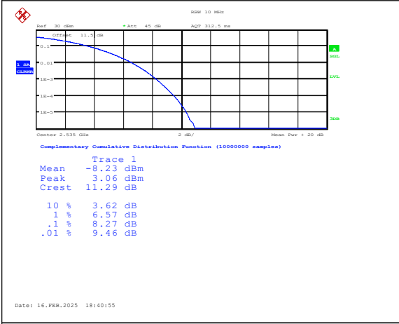
Band7-20MHz-QPSK-21100-1RB#0-PASS
