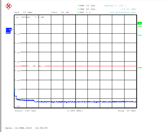
Band7-5MHz-16QAM-21425-1RB#0-0.15~30-PA SS
