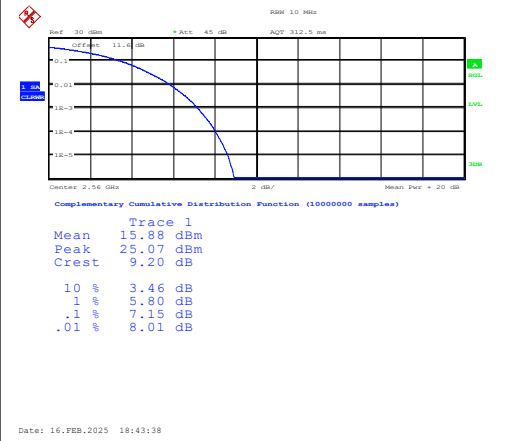
Band7-20MHz-16QAM-21350-100RB#0-PASS
