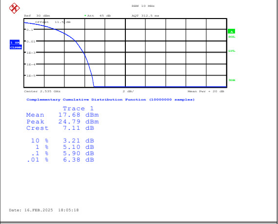
Band7-15MHz-QPSK-21100-75RB#0-PASS
