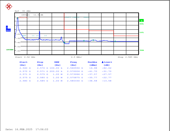
Band7-10MHz-16QAM-21400-1RB#0-PASS
