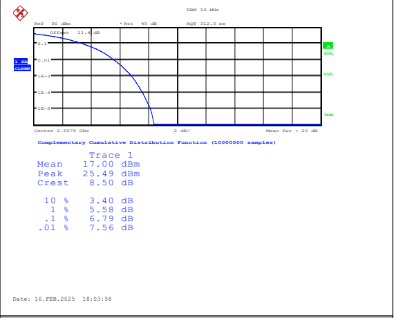
Band7-15MHz-16QAM-20825-75RB#0-PASS
