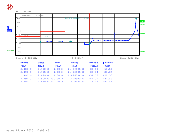
Band7-10MHz-16QAM-20800-1RB#49-PASS
