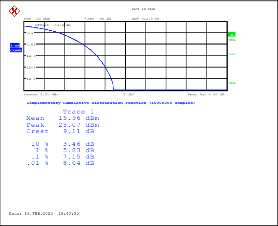
Band7-20MHz-16QAM-20850-100RB#0-PASS
