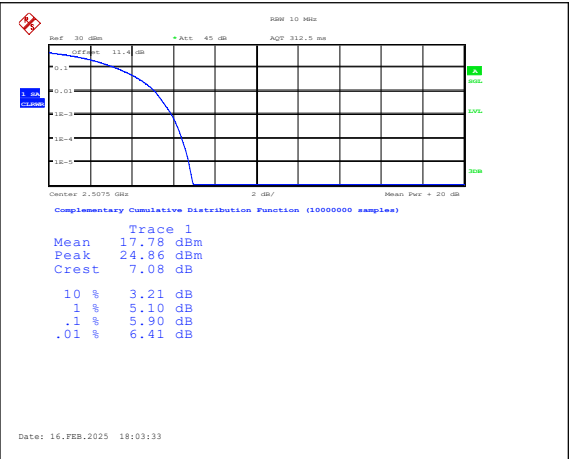
Band7-15MHz-QPSK-20825-75RB#0-PASS
