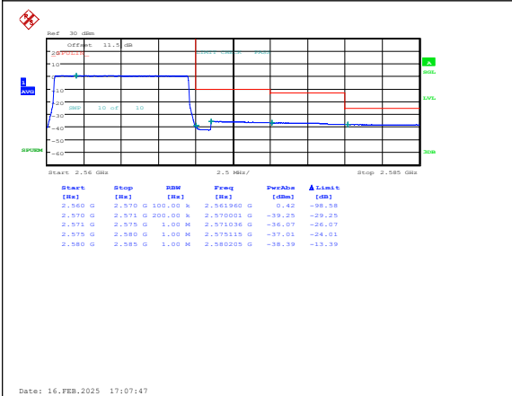
Band7-10MHz-QPSK-21400-50RB#0-PASS
