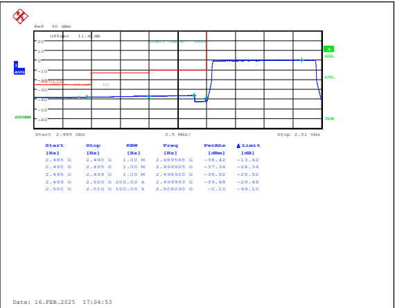
Band7-10MHz-16QAM-20800-50RB#0-PASS
