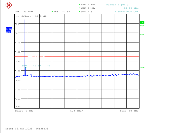
Band7-5MHz-16QAM-21425-1RB#0-1000~20000 -PASS
