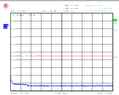
Band7-10MHz-QPSK-20800-1RB#0-0.15~30-PASS
