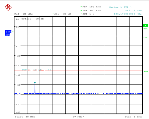
Band7-5MHz-16QAM-20775-1RB#0-30~1000-PAS S
