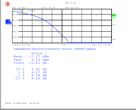
Band7-15MHz-QPSK-21100-1RB#0-PASS
