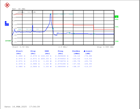
Band7-10MHz-QPSK-21400-1RB#49-PASS
