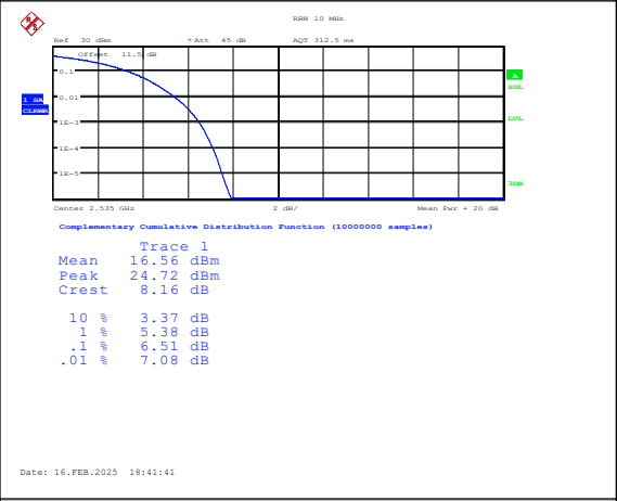
Band7-20MHz-QPSK-21100-100RB#0-PASS
