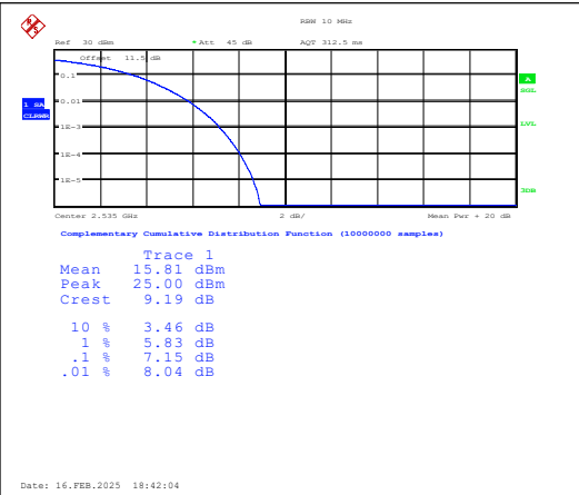
Band7-20MHz-16QAM-21100-100RB#0-PASS
