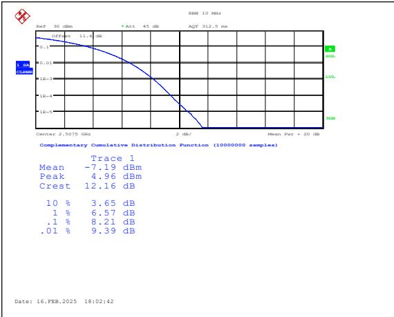
Band7-15MHz-QPSK-20825-1RB#0-PASS
