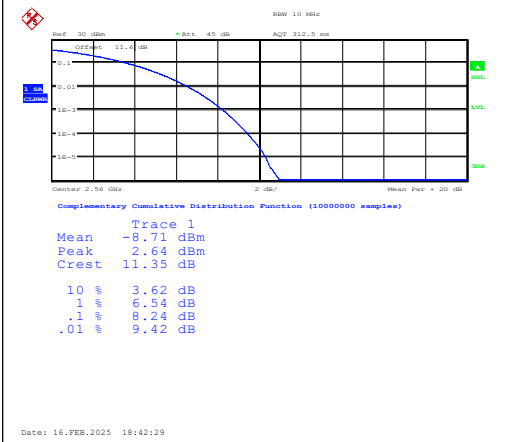
Band7-20MHz-QPSK-21350-1RB#0-PASS
