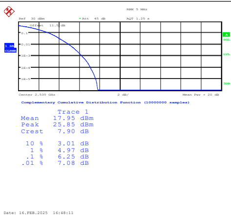
Band7-5MHz-16QAM-21100-25RB#0-PASS
