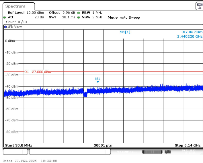
11N20MIMO_5180_30~5140
