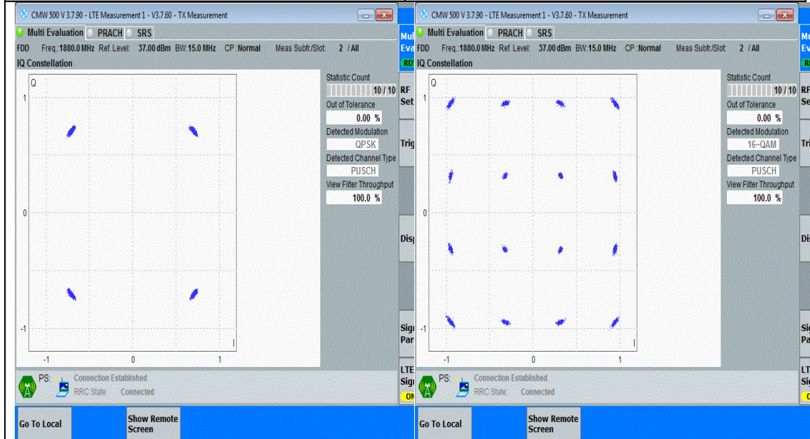
Band2-15MHz-QPSK-18900-75RB#0-PASS
