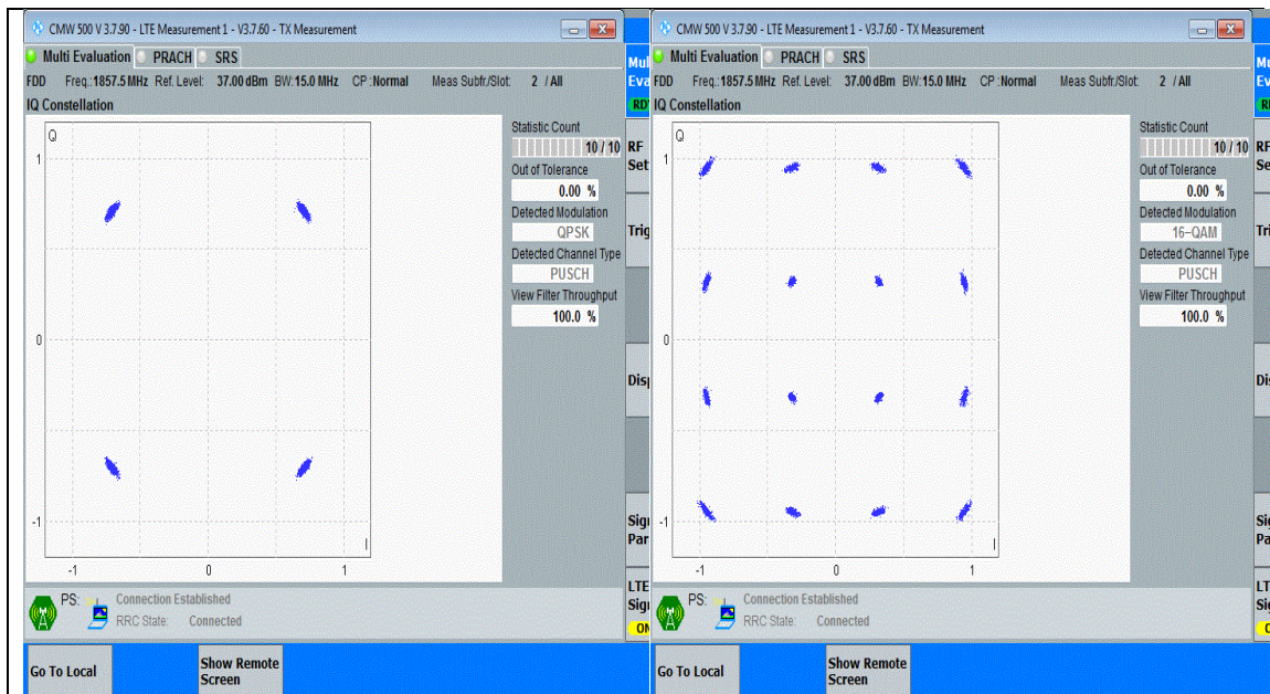
Band2-15MHz-QPSK-18675-75RB#0-PASS
