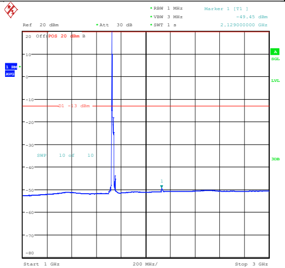
Band4-15MHz-QPSK-20175-1RB#0-0.15~30-PAS S
