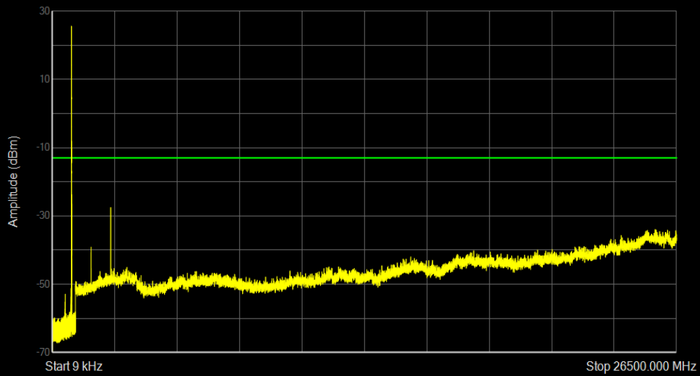
Band5 16QAM BW=10MHz Channel=20525 RB Size=1 Position=#0
