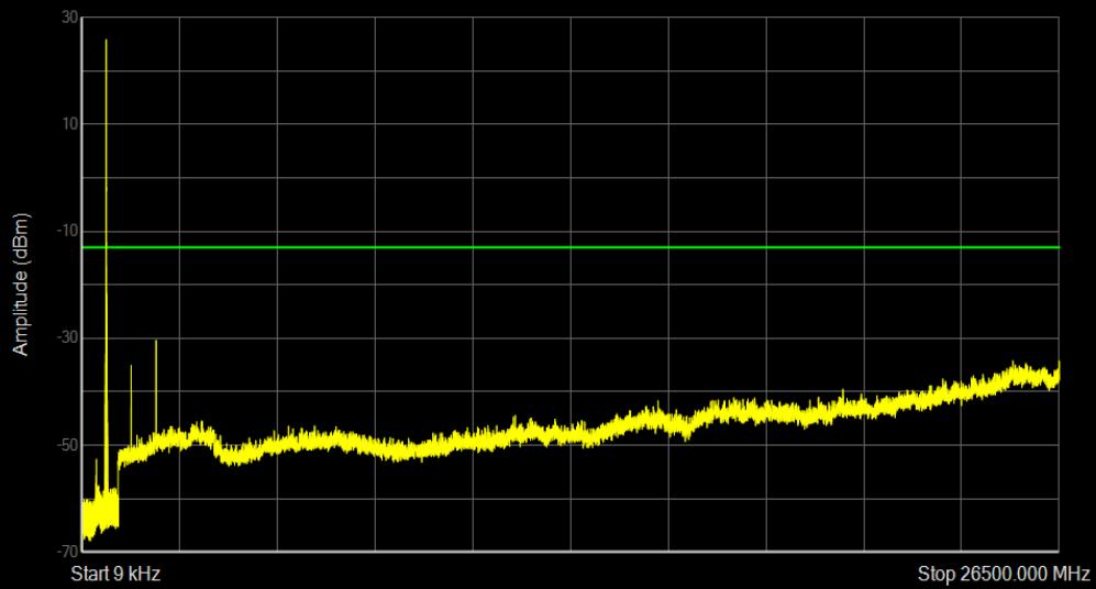
Band71 16QAM BW=10MHz Channel=133297 RB Size=1 Position=#0
