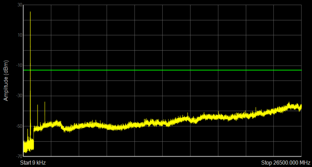
Band71 16QAM BW=10MHz Channel=133422 RB Size=1 Position=#0
