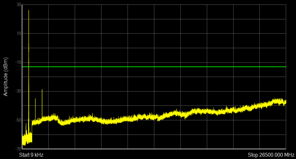
Band71 16QAM BW=15MHz Channel=133297 RB Size=1 Position=#0
