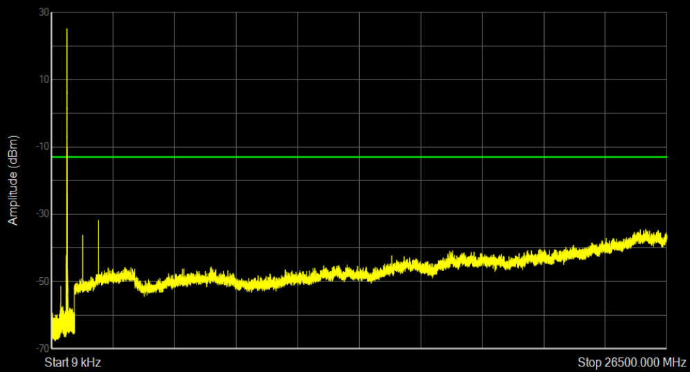
Band71 16QAM BW=20MHz Channel=133372 RB Size=1 Position=#0
